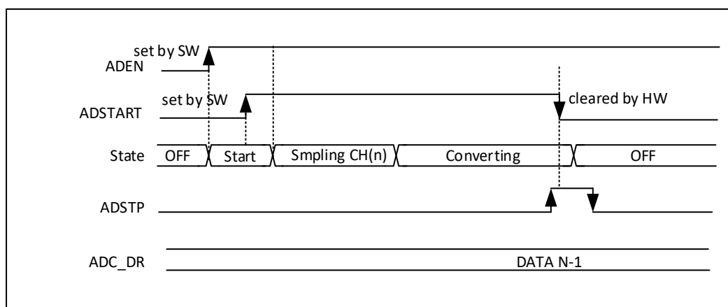
图 12-7 Stop ongoing regular conversions
