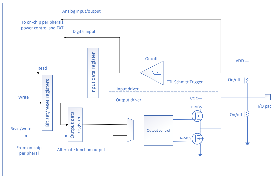
图 5 1Basic structure of an IO port bit
