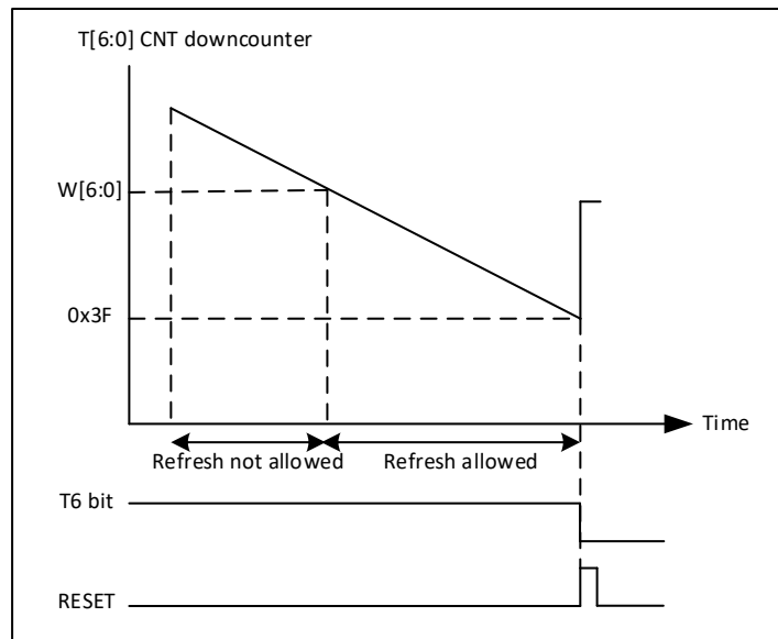
图 26-2 window watchdog timing diagram
