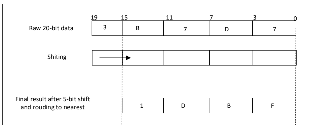
图 12-21 Numerical example with 5-bit shift and rounding
