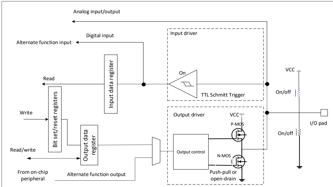
图 7-3 Alternative function configuration
