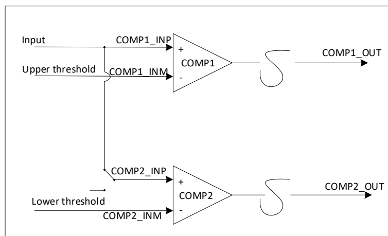
图 14-3 window comparator
