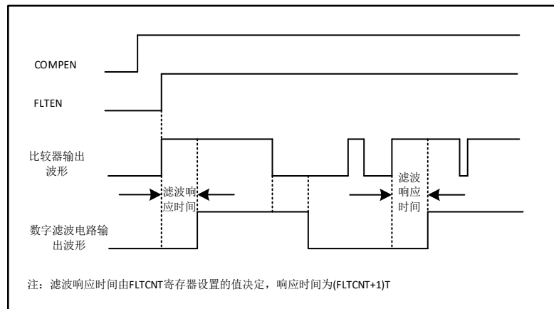
图 14-4 COMP filter
