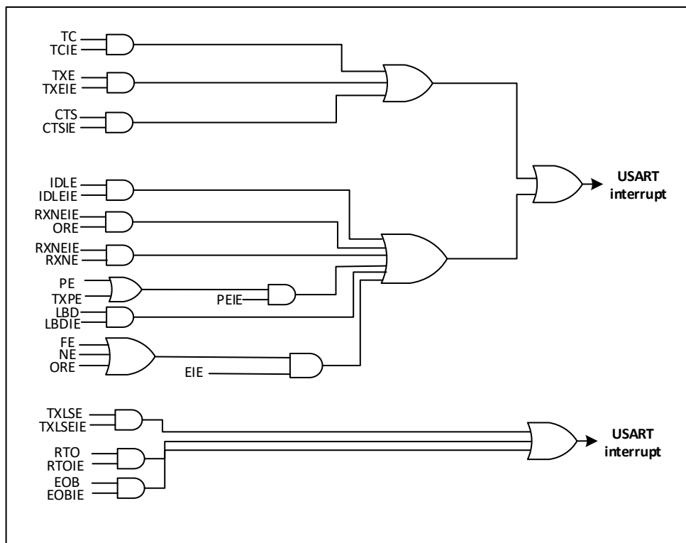
图 30-25 USART interrupt mapping diagram
