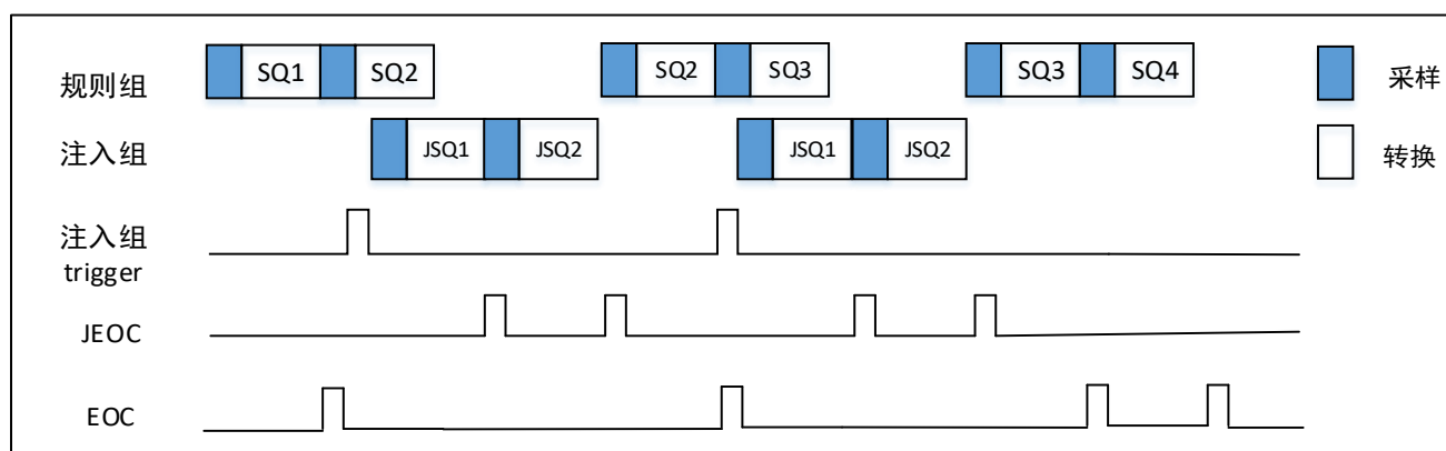
图 12-5 ADC trigger injection timing
