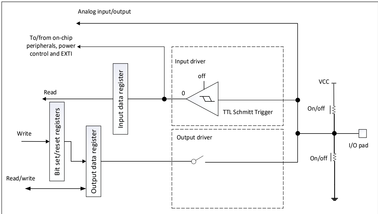
图 7-4 high impedance-analog configuration
