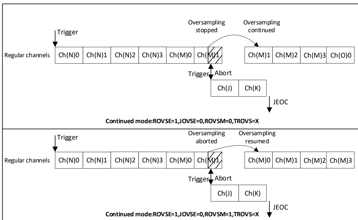
图 12-23 Regular over sampling mode(4x Ratio)
