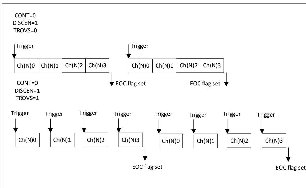
图 12-22 Triggered regular oversampling mode (TROVS=1)
