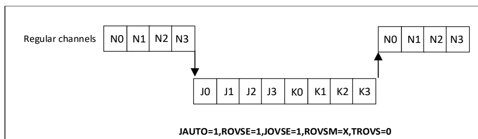
图 12-26 oversampling in auto-injected mode
