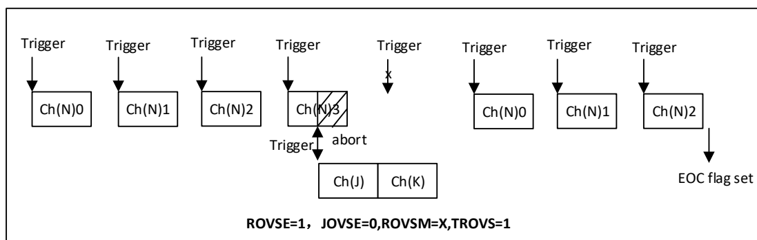
图 12-24 Regular and injected oversampling modes used simultaneously
