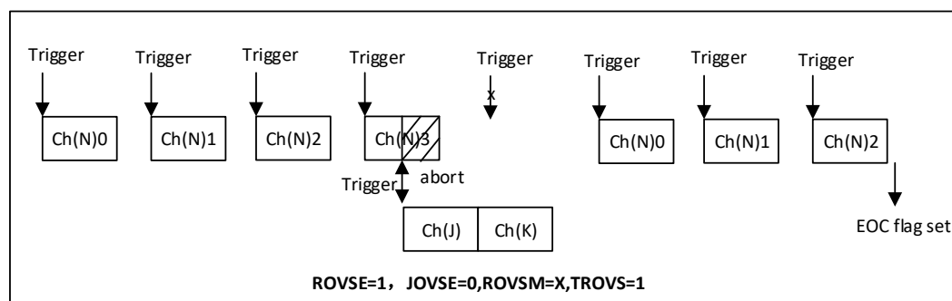
图 12-25 Triggered regular oversampling with injection
