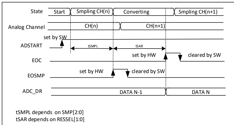
图 12-6 analog to digital conversion timing
