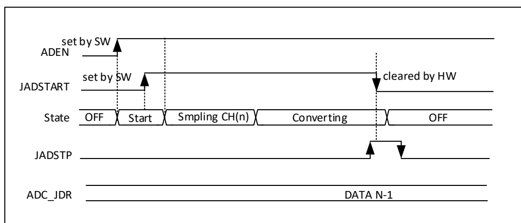
图 12-8 Stop ongoing injected conversions
