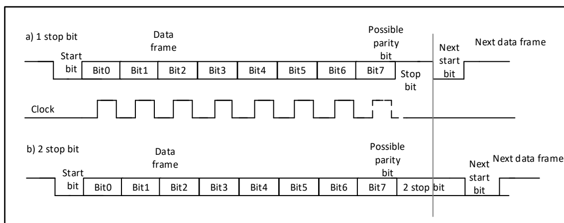
Figure 30-3 Configuring Stop Bits
