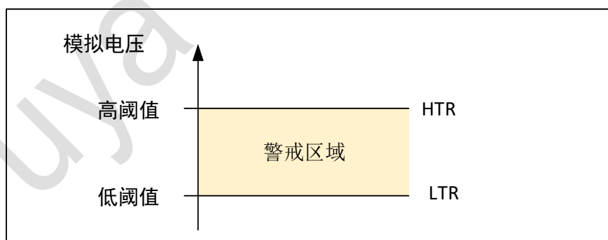
Figure 14-4 Analog Watchdog Protection Area
