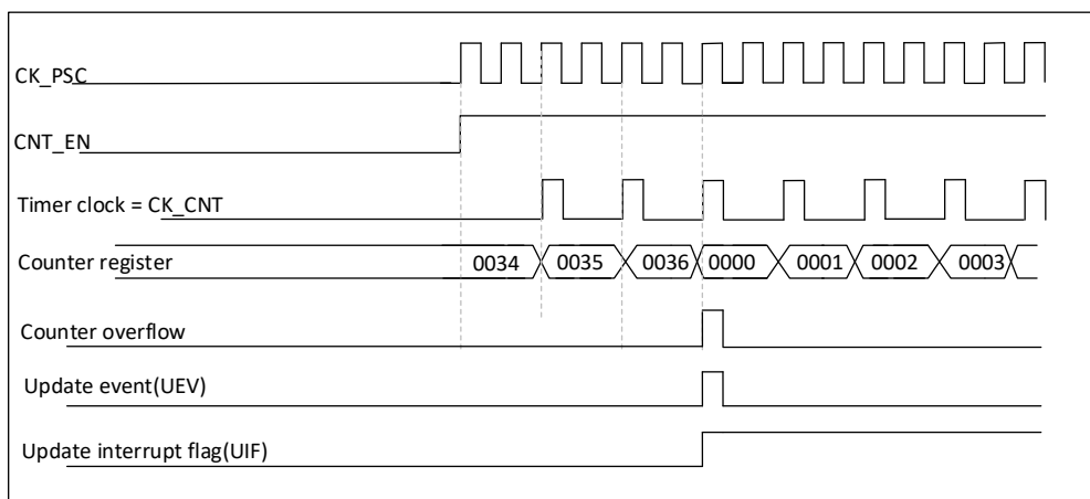
Figure 22-5 Timing diagram of the counter with internal clock divider factor of 2
