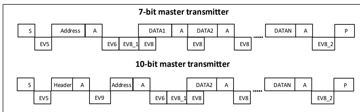
Figure 28-5 Master transmitter transfer sequence diagram
