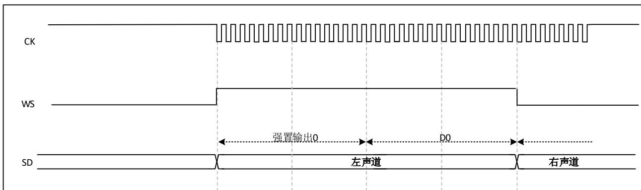
Figure 29-27 LSB-aligned 16-bit data extended to 32-bit packet frame, CKPOL=1
