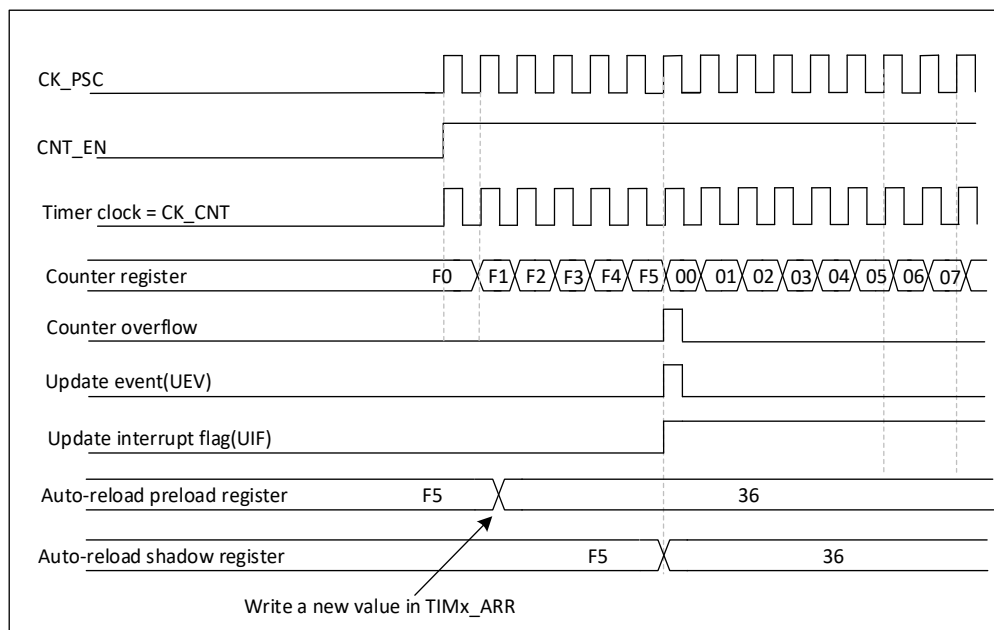
Figure 19-9 Counter timing diagram, update event when ARPE=1 (preloaded with TIMx_ARR)
