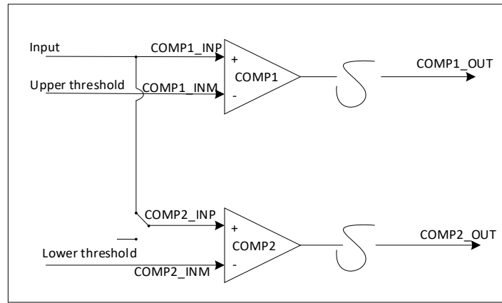
Figure 16-2 Window Comparator
