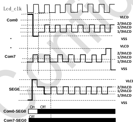
Figure 15-3 1/8DUTY 1/3 BIAS Drive Waveforms
