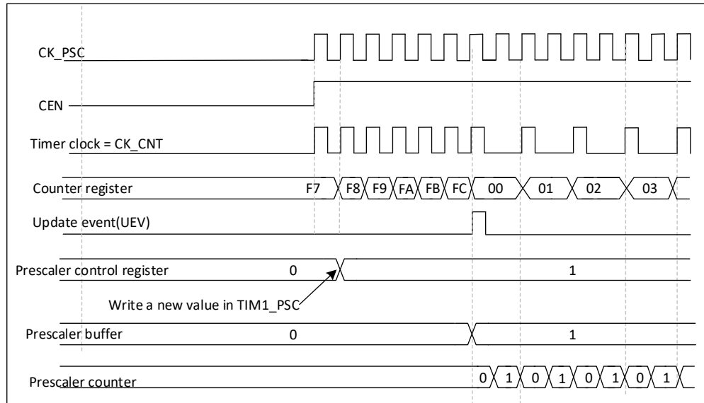
Figure 22-2 Timing diagram of the counter when the prescaler parameter is changed from 1 to 2
