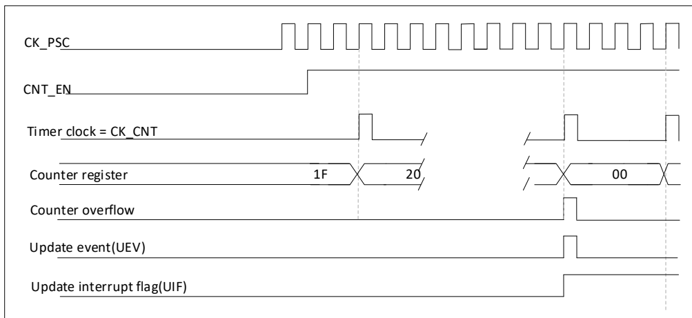
Figure 19-7 Timing diagram of the counter with internal clock dividing factor N
