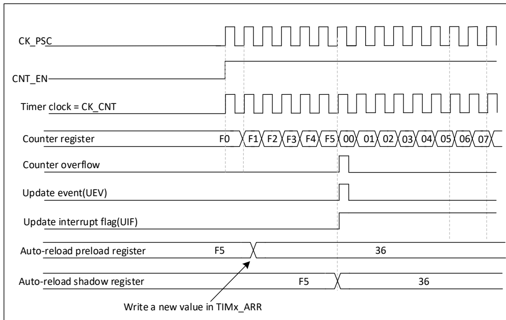
Figure 22-9 Counter timing diagram, update event when ARPE=1 (preloaded with TIMx_ARR)
