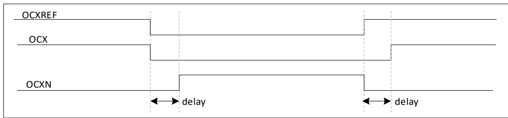
Figure 23-22 Complementary outputs with dead-time insertion
