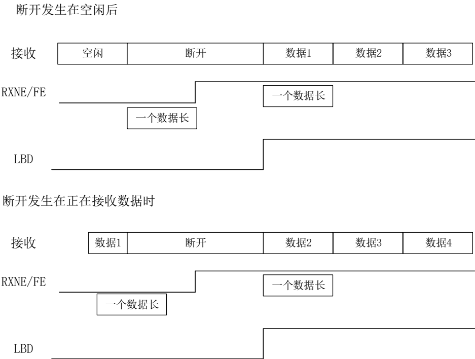
Figure 30-11 Break detection and frame error detection in LIN mode
