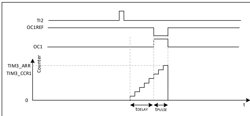
Figure 20-31 Example of single pulse mode
