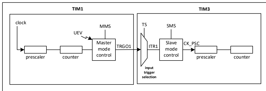
Figure 23-35 Example of Master/Slave Timers
