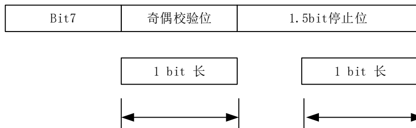
Figure 30-17 Detecting Parity Errors Using 1.5 Stop Bits
