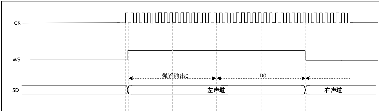
Figure 29-26 LSB-aligned 16-bit data extended to 32-bit packet frame, CKPOL=0
