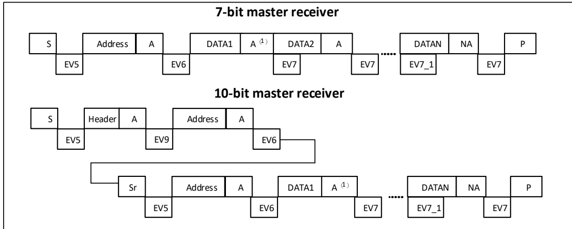
Figure 28-6 Method 1: Timing diagram for master mode transmission.
