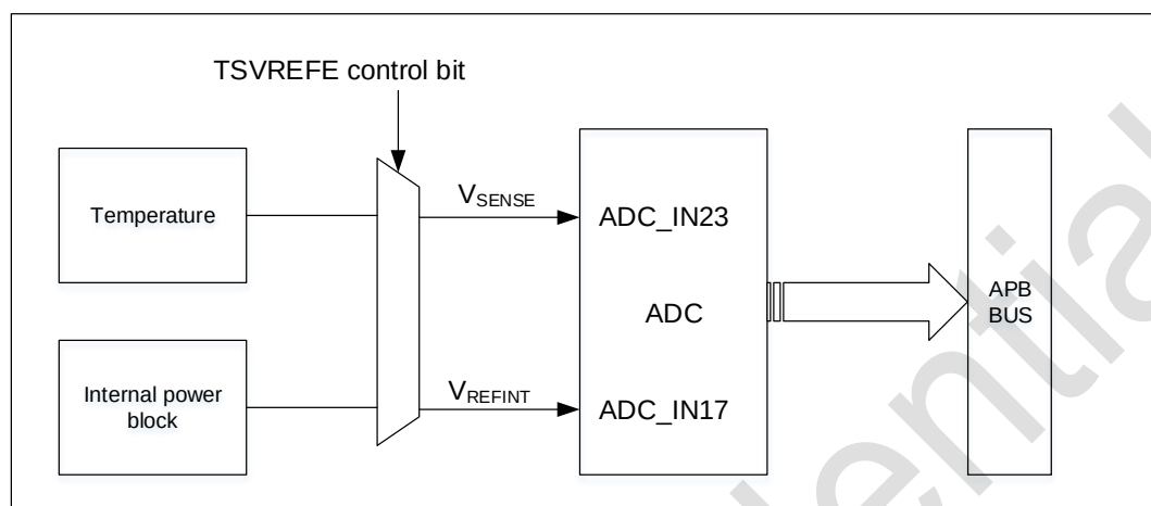
Figure 14-5 Temperature Sensor Channel Block Diagram
