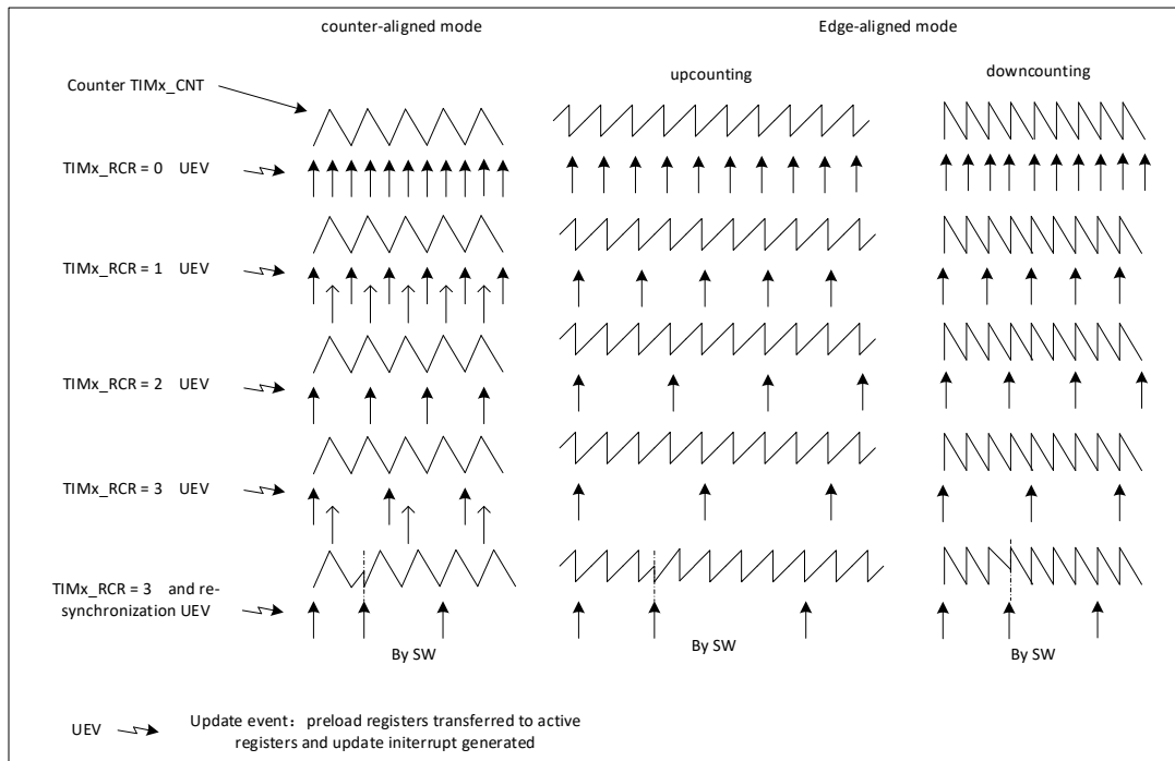
Figure 19-21 Example of update rate in different modes and register setting of TIMx_RCR
