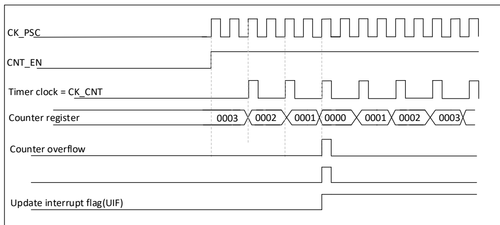
Figure 19-16 Counter timing diagram with internal clock divider factor of 2 and TIMx\_ARR = 0x36
