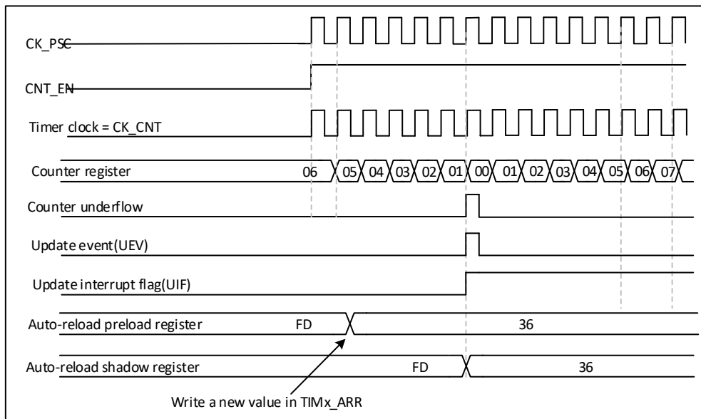
Figure 20-19 Counter timing diagram, update event at ARPE=1 (counter underflow)
