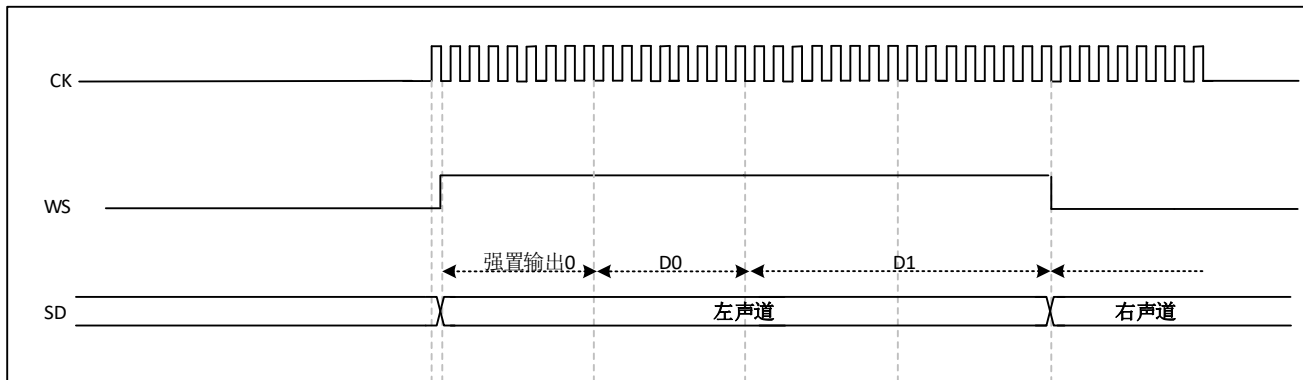
Figure 29-24 LSB-aligned 24-bit data, CKPOL=0
