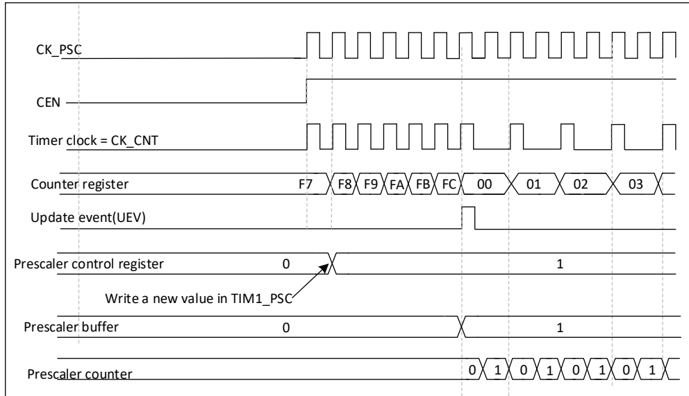
Figure 23-3 Timing diagram of the counter when the prescaler parameter changes from 1 to 2
