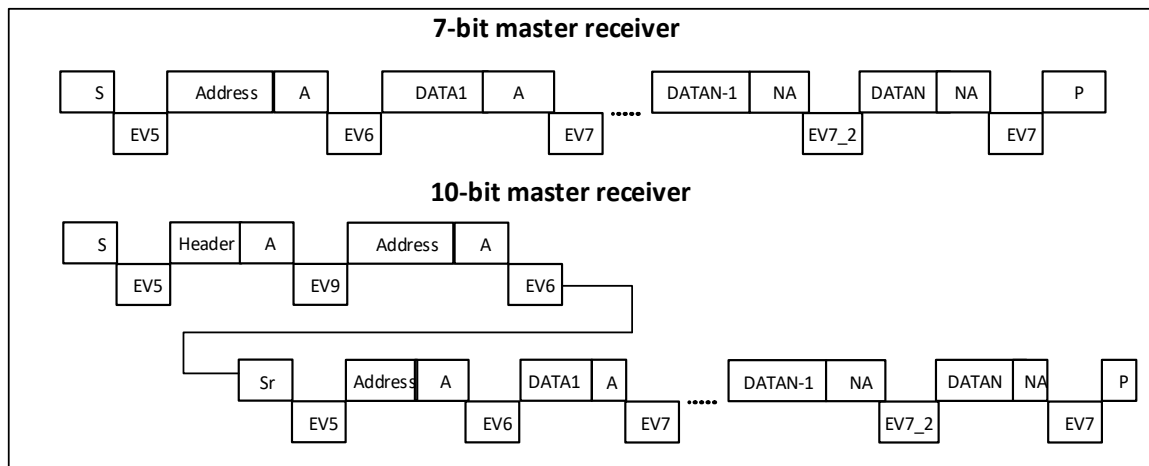
Figure 28-7 Method 2: Timing diagram for master transmission when N > 2
