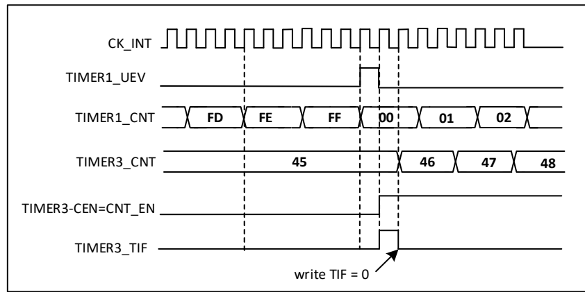
Figure 23-38 Using Timer 1's update event to trigger Timer 2
