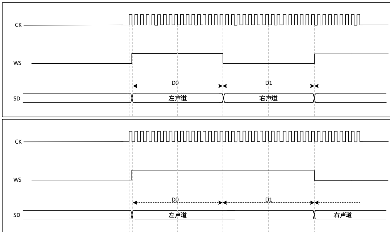
Figure 29-22 LSB-aligned 16-bit or 32-bit full precision, CKPOL = 0
