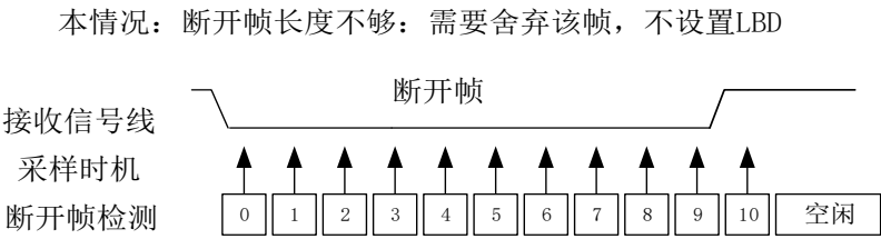
Figure 30-9 Case where the break frame length is insufficient in LIN mode
