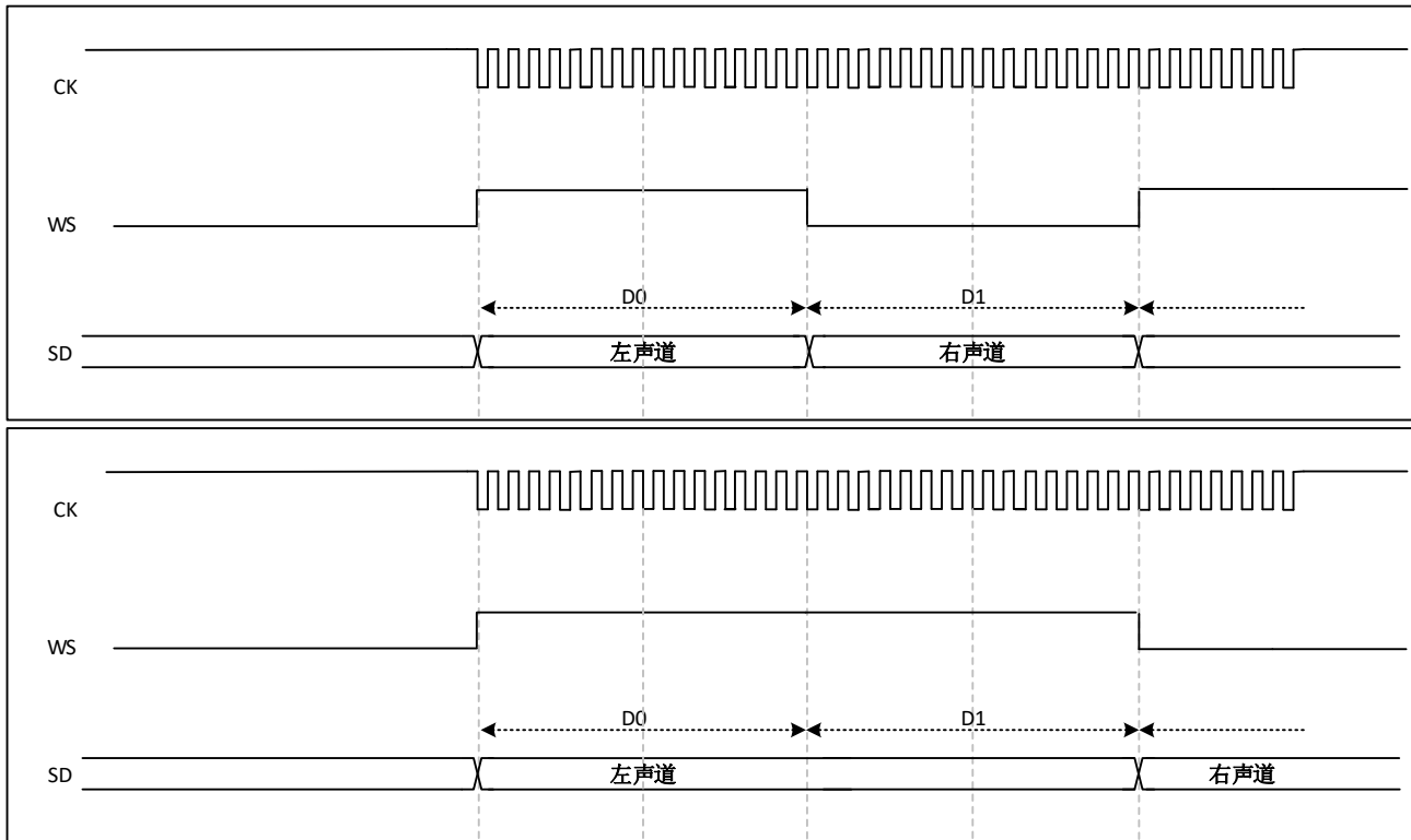
Figure 29-23 LSB-aligned 16-bit or 32-bit full precision, CKPOL = 0
