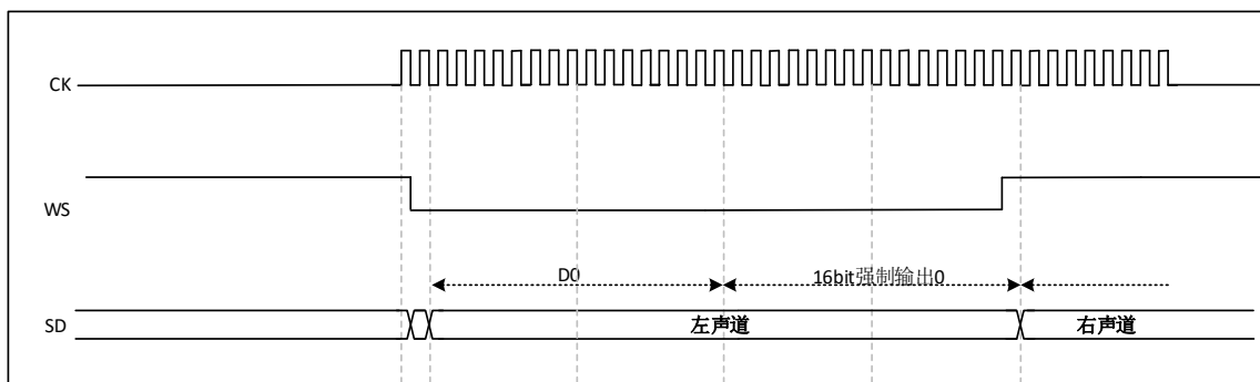
Figure 29-15 I2S Philips protocol standard waveform (16-bit extended to 32-bit packet frame, CPOL = 0)
