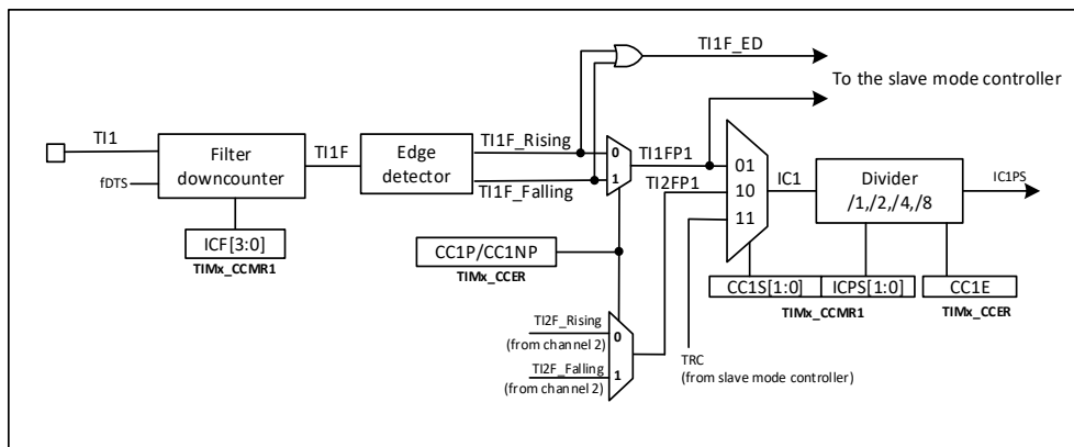
Figure 20-24 Capture/compare channels (e.g., channel 1 input section)
