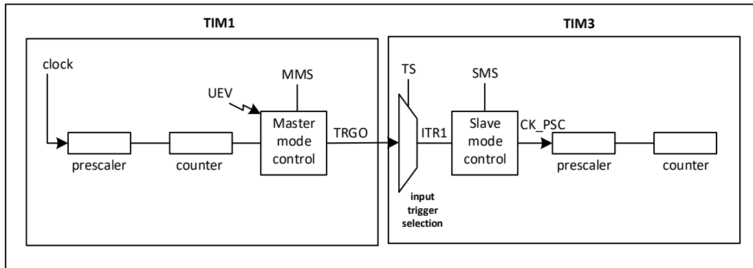
Figure 20-38 Example of a master/slave timer
