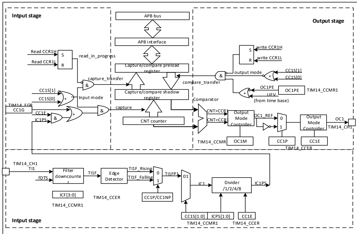
Figure 22-11 TIM14 Capture/Compare Channel Diagram
