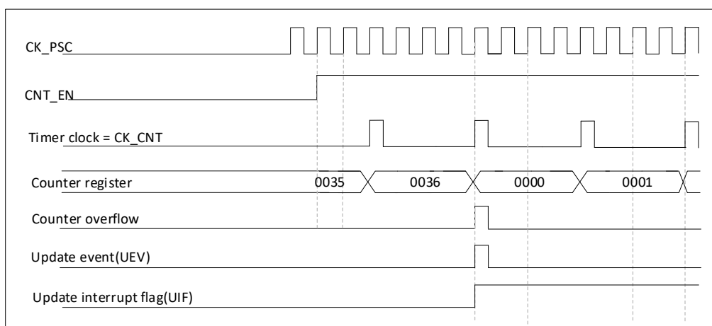
Figure 21-6 Timing diagram of the counter with internal clock divider factor of 4
