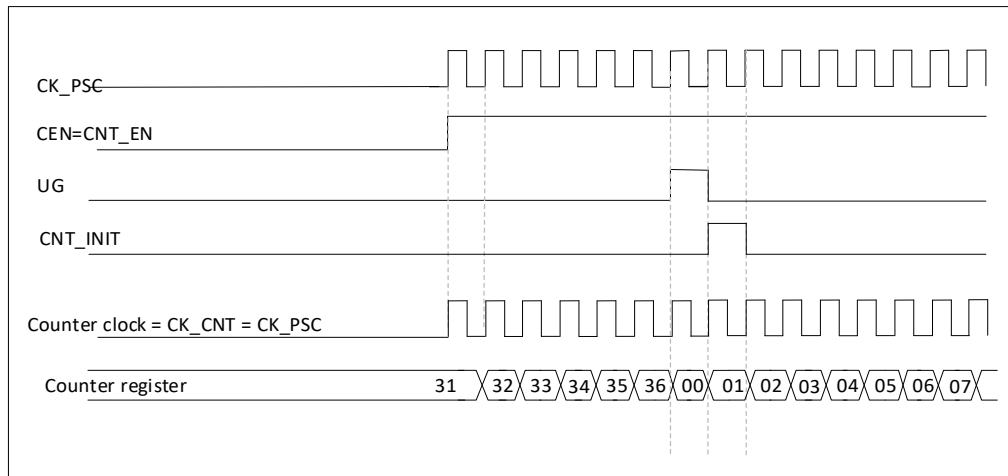
Figure 23-12 Control circuit in normal mode, internal clock division factor is 1
