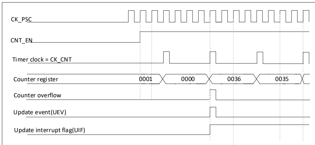
Figure 19-12 Timing diagram of the counter with internal clock divider factor of 4
