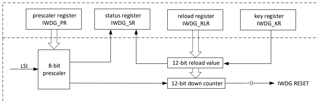
Figure 25-1 IWDG block diagram
