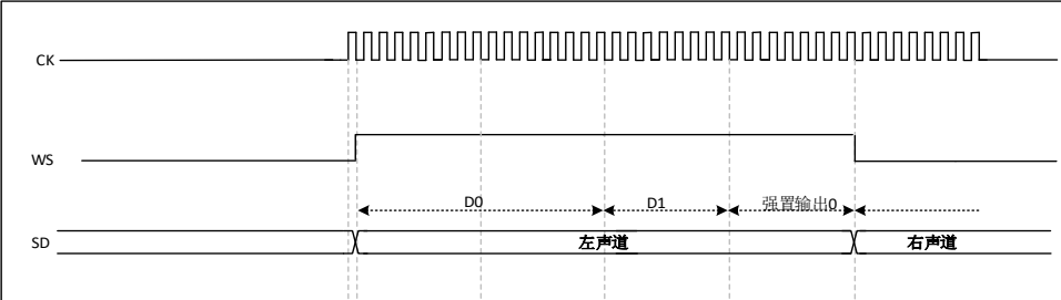
Figure 29-20 MSB-aligned standard, 16-bit extended to 32-bit, CPKOL = 0
