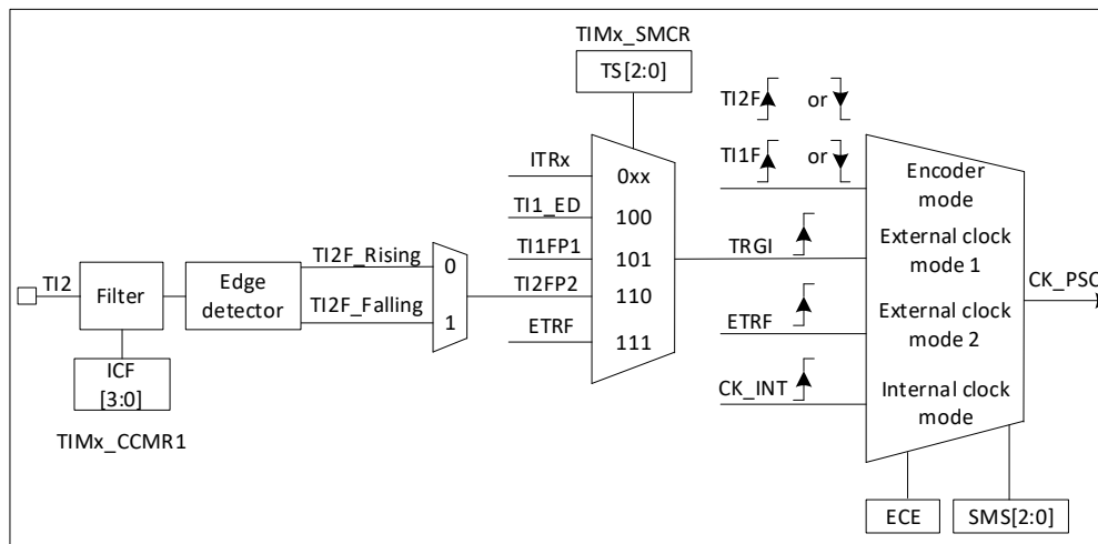
Figure 23-13 Example of TI2 external clock connection
