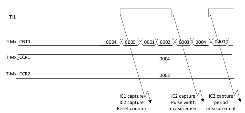
Figure 23-19 PWM input mode timing diagram
