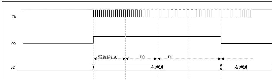
Figure 29-21 MSB-aligned standard, 16-bit extended to 32-bit, CPKOL = 1
