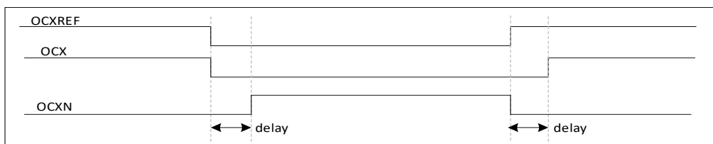
Figure 19-35 Complementary output with deadband insertion
