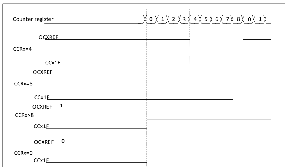
Figure 23-21 Edge-aligned PWM output, up-counting (ARR=8)
