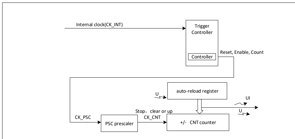
Figure 21-1 Block diagram of basic timer architecture
