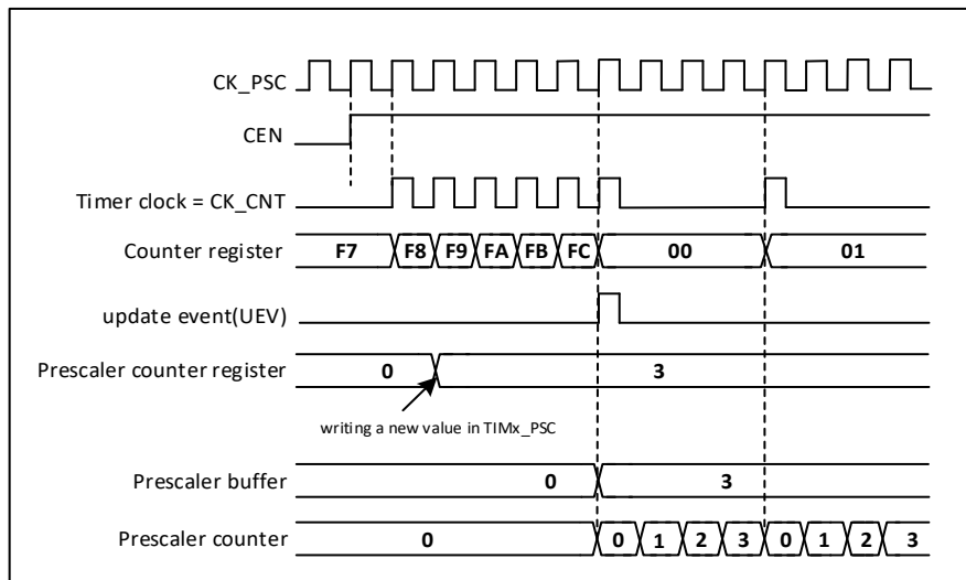
Figure 20-3 Timing diagram of the counter when the prescaler parameter is changed from 1 to 4
