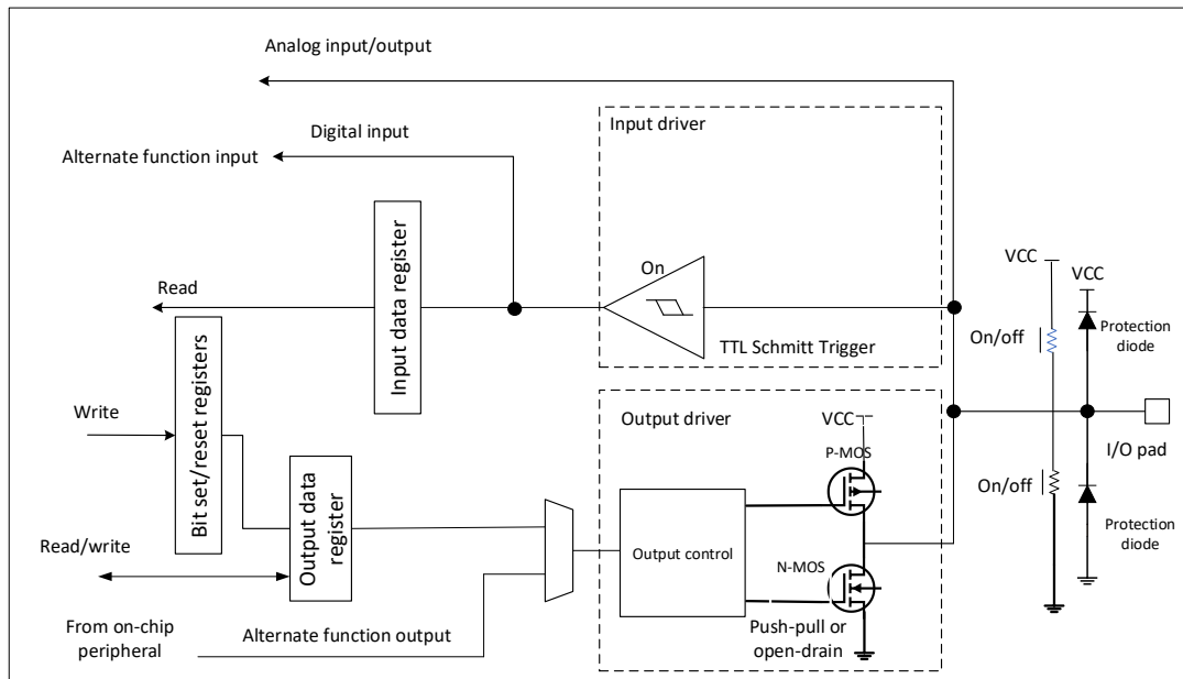
Figure 9-4 Multiplexing Function Configuration
