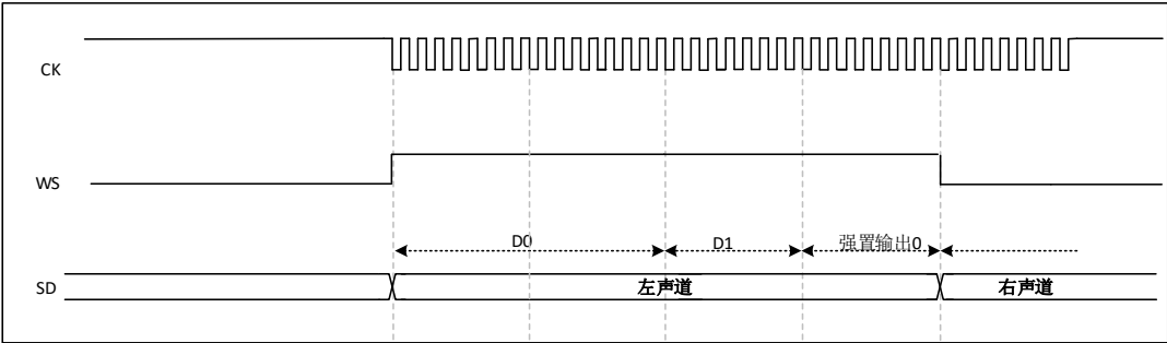
Figure 29-19 MSB-aligned 24-bit frame, CPKOL = 1
