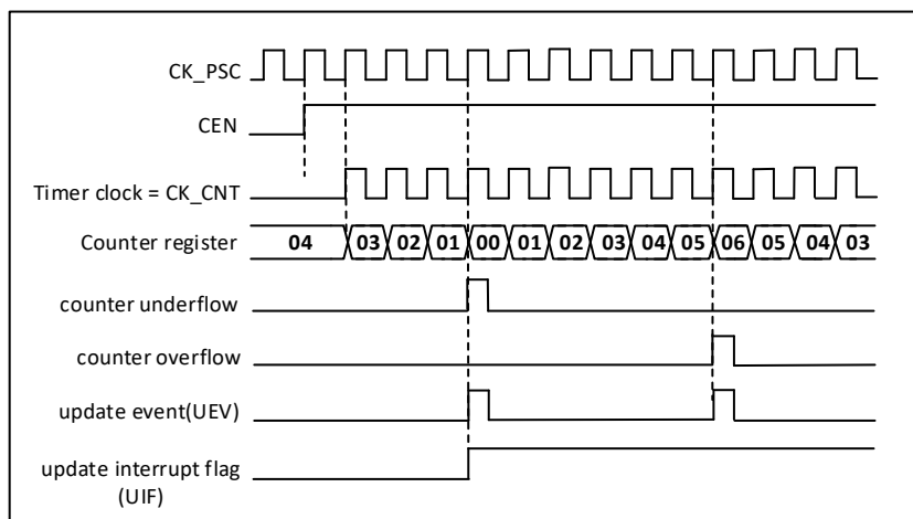
Figure 20-15 Counter timing diagram with internal clock divider factor of 1 and TIMx_ARR = 0x6
