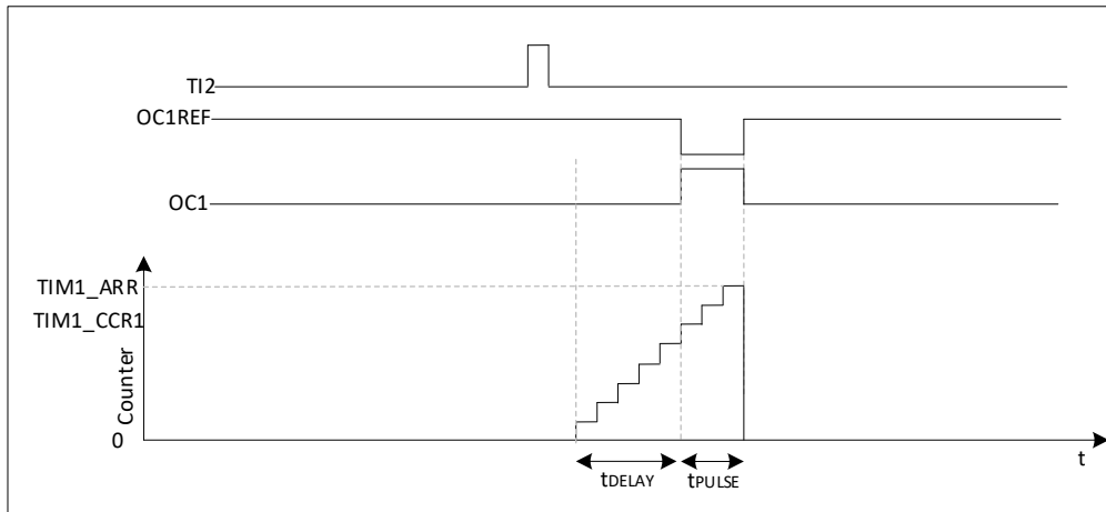
Figure 23-26 Example of Single Pulse Mode
