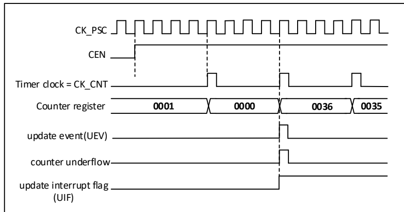
Figure 20-12 Timing diagram of the counter with internal clock divider factor of 4
