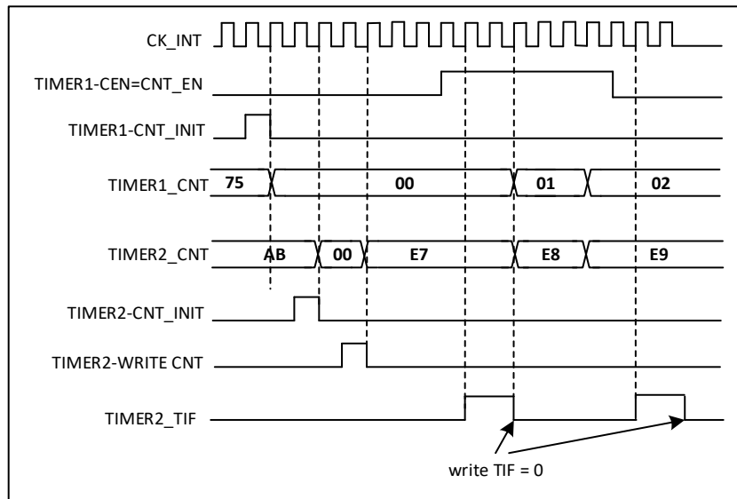
Figure 20-40 Timer 2 can be controlled by enabling Timer 1
