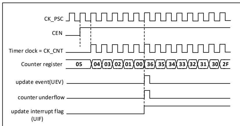
Figure 20-10 Timing diagram of the counter with internal clock division factor of 1
