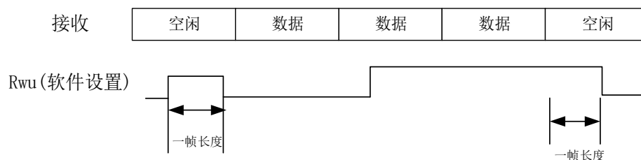
Figure 30-7 Silent Mode Using Idle Bus Detection
