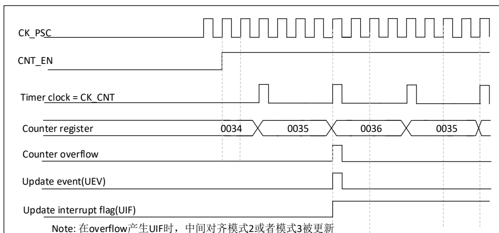
Figure 19-17 Counter timing diagram with internal clock divider factor of 4 and TIMx\_ARR = 0x36
