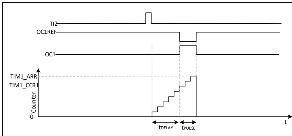
Figure 19-41 Example of single pulse mode
