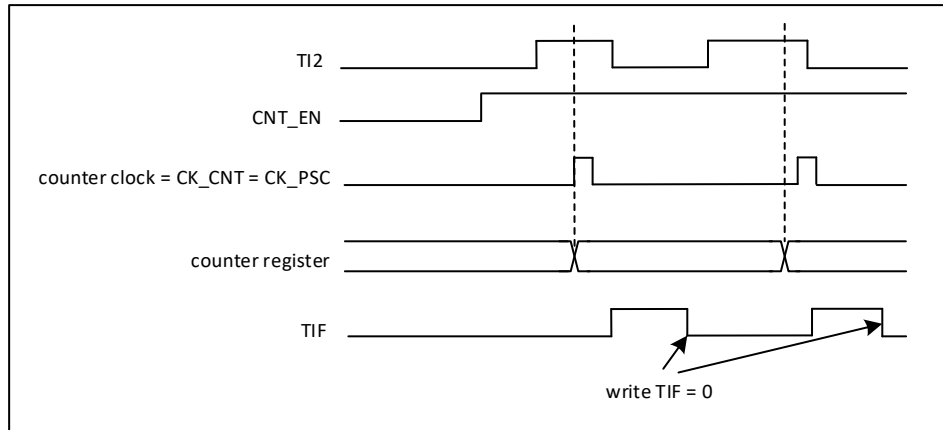
Figure 20-23 Control circuit in external clock mode 1
