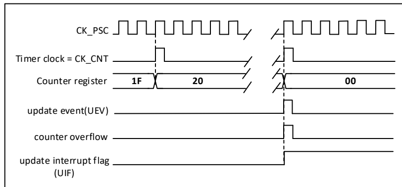
Figure 20-7 Timing diagram of the counter with internal clock dividing factor N
