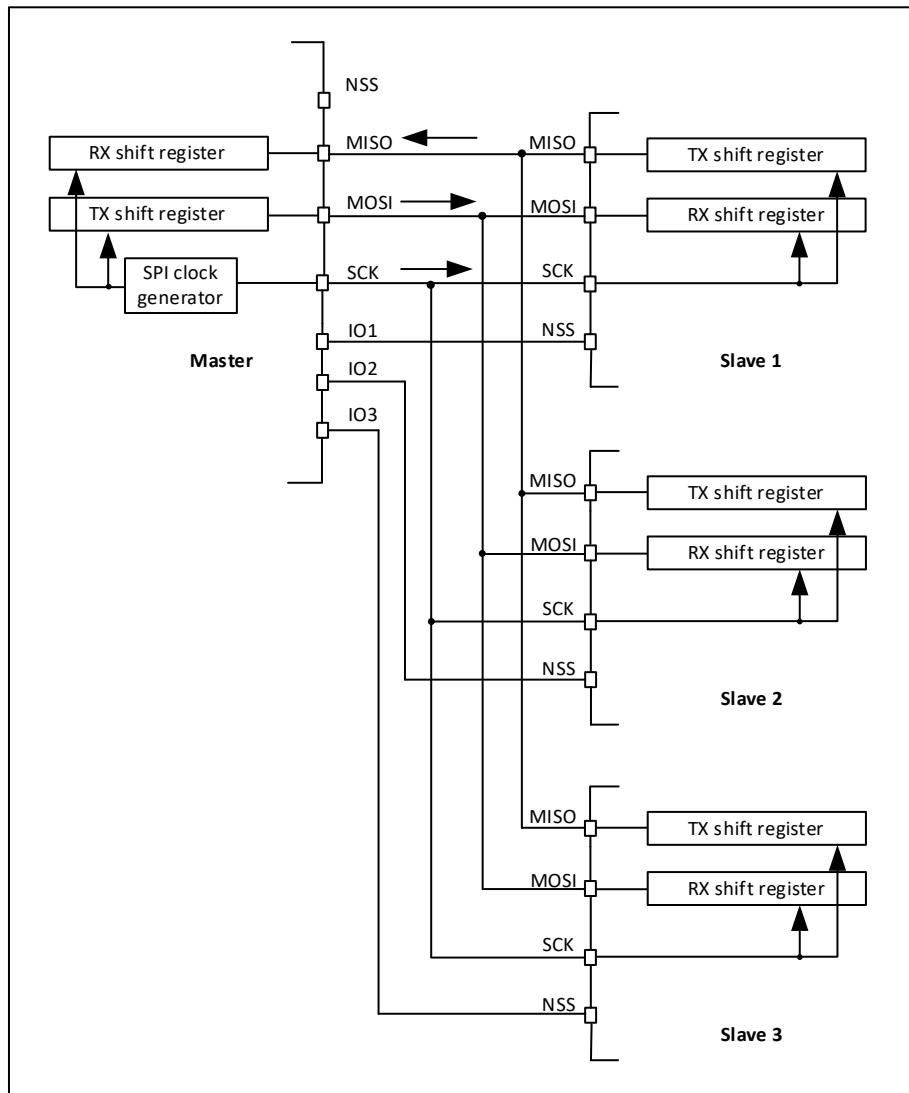
Figure 29-5 Master Communicating with Three Independent Slaves
