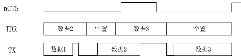
Figure 30-23 CTS flow control
