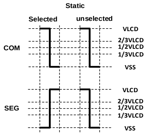
Figure 15-2 Static drive waveform
