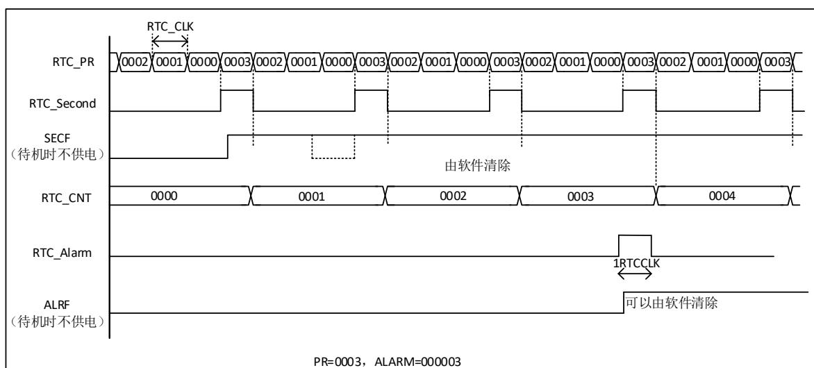
Figure 27-2 Example of RTC Second and Alarm Waveform, PR=0003, ALR=00003
