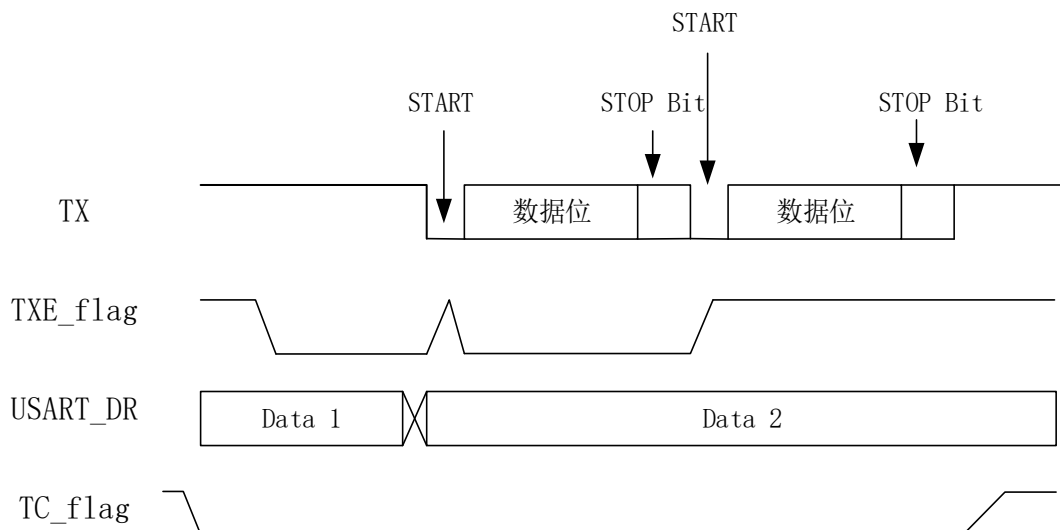
Figure 30-4 Changes in TC/TXE during USART transmission
