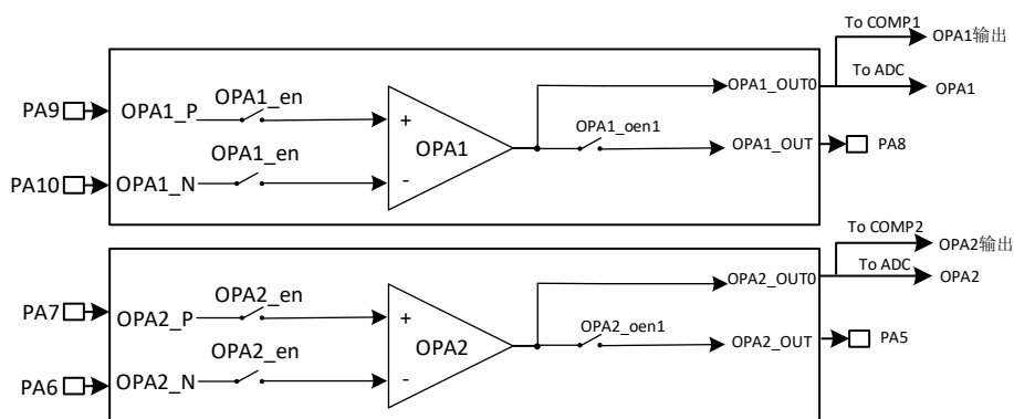
Figure 17-1 OPA Architecture Block Diagram
