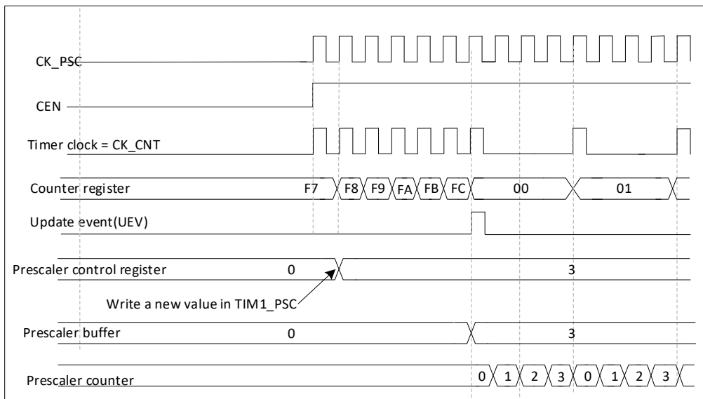
Figure 19-3 Timing diagram of the counter when the prescaler parameter is changed from 1 to 4
