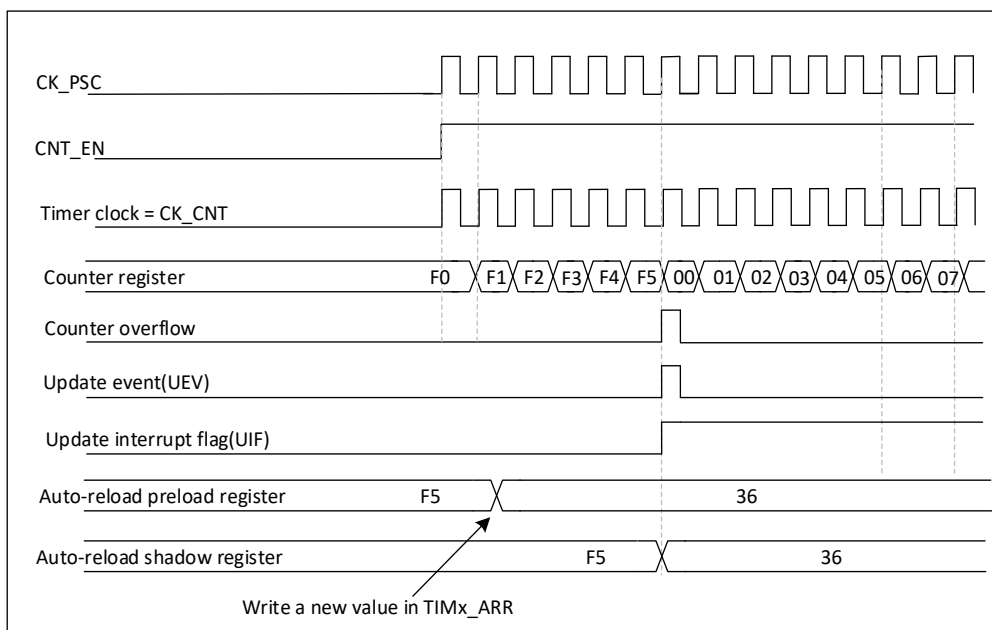
Figure 23-10 Counter timing diagram showing update events when ARPE=1 (TIMx_ARR preloaded)
