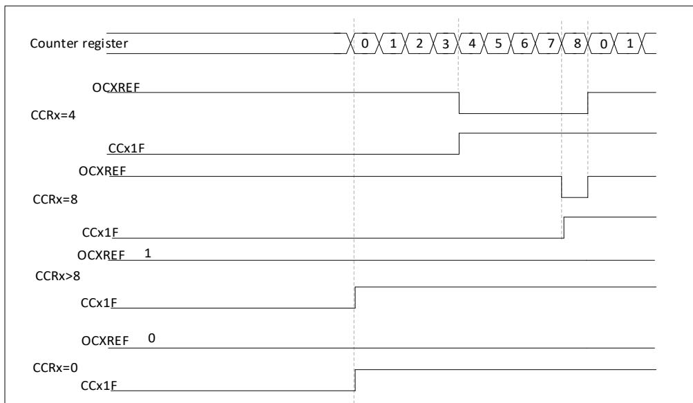
Figure 19-33 Edge-aligned PWM output, up (ARR=8)
