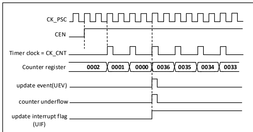
Figure 20-11 Timing diagram of the counter with internal clock divider factor of 2
