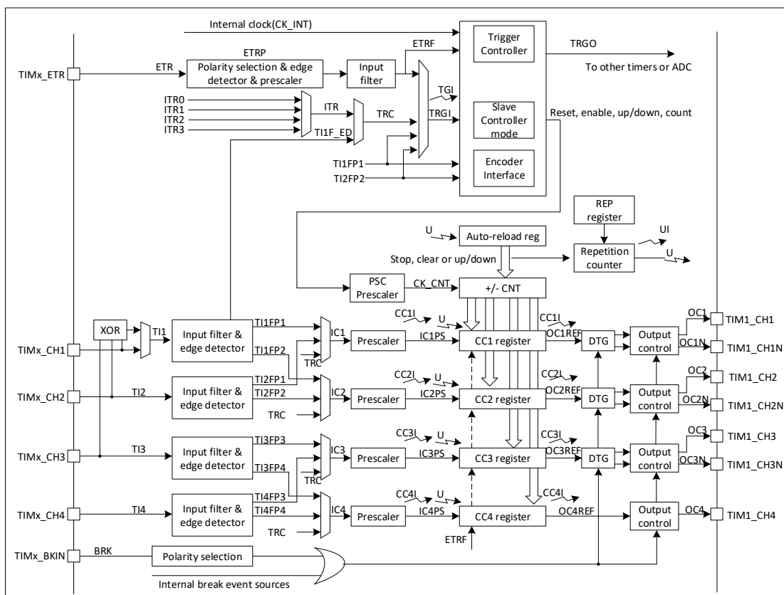
Figure 19-1 Advanced Control Timer Architecture Block Diagram
