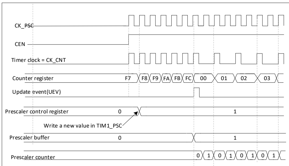
Figure 19-2 Timing diagram of the counter when the prescaler parameter is changed from 1 to 2
