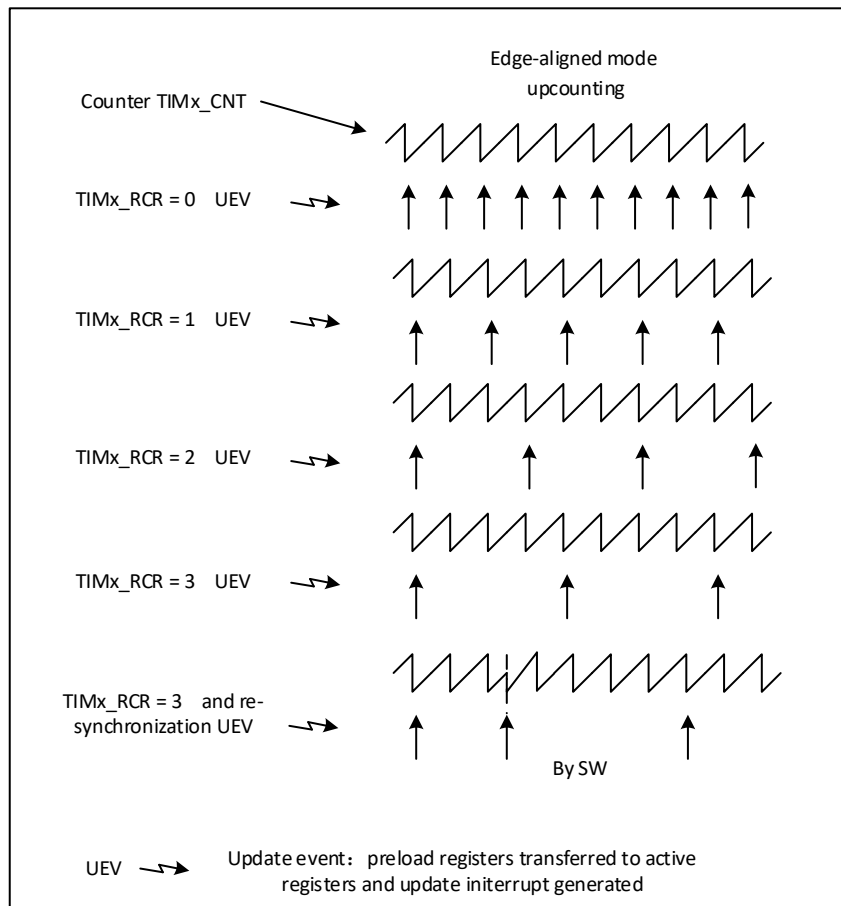
Figure 23-11 Example of update rates in different modes, and TIMx_RCR register settings
