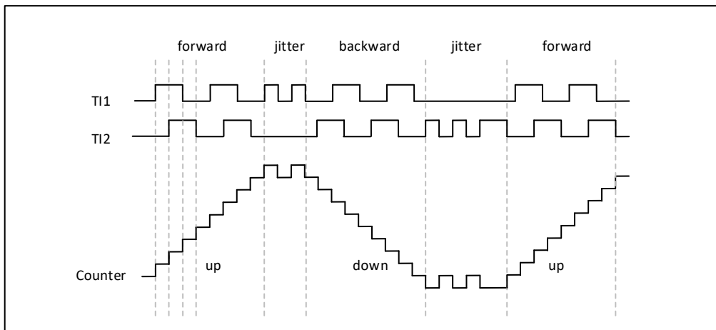
Figure 20-32 Example of counter operation in encoder mode
