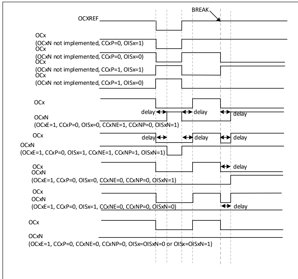
Figure 19-38 Output in response to braking
