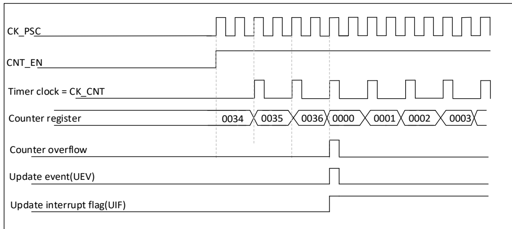
Figure 23-6 Counter timing diagram with internal clock division factor 2
