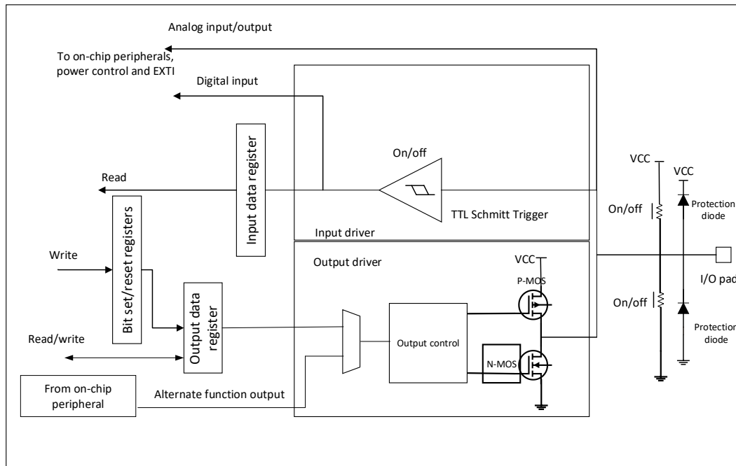
Figure 9-1 Basic structure of IO port bits
