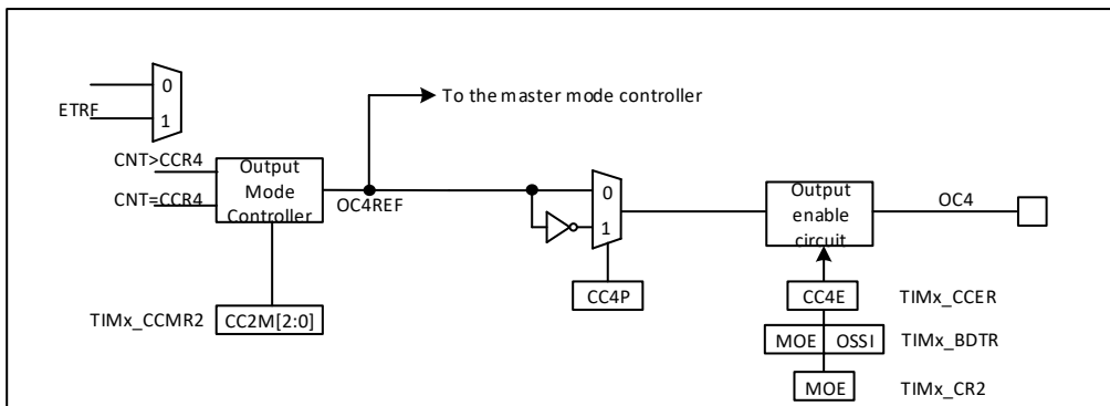
Figure 23-18 Output section of the capture/compare channel (Channel 4)
