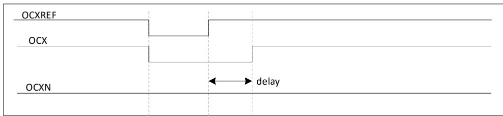
Figure 19-36 Deadband waveform delay greater than negative pulse
