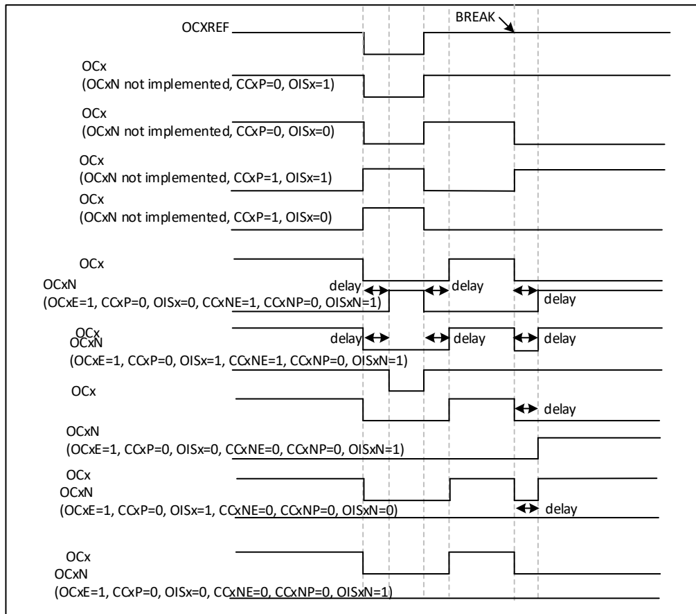
Figure 23-25 Output Response to Brake
