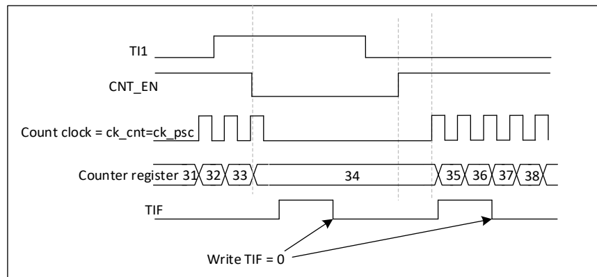
Figure 19-46 Control circuit in gated mode
