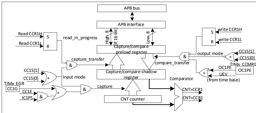
Figure 23-16 Main circuit of capture/compare channel 1
