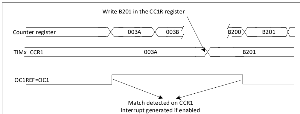
Figure 23-20 Output compare mode, toggle OC1
