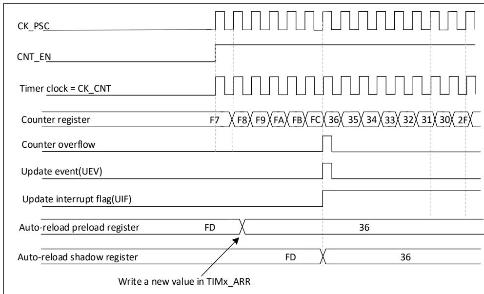
Figure 19-20 Counter timing diagram, update event at ARPE=1 (counter overflow)
