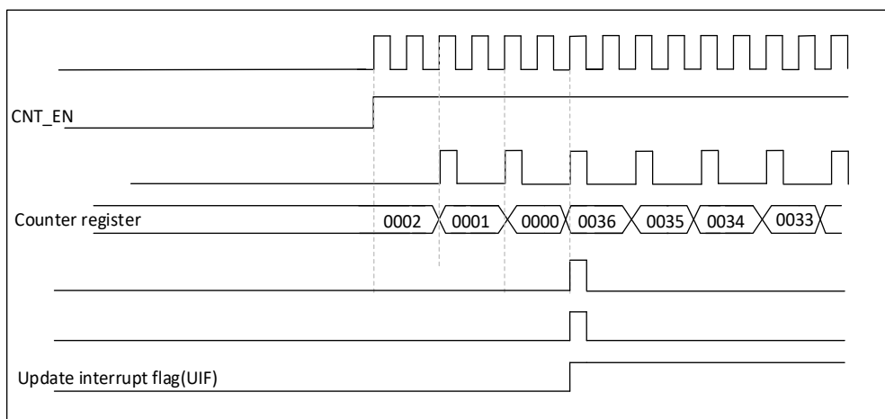
Figure 19-11 Timing diagram of the counter with internal clock divider factor of 2
