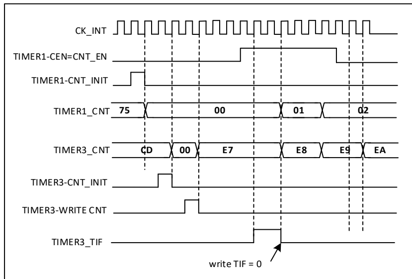
Figure 20-42 Trigger Timer 3 with Timer 1 Enable
