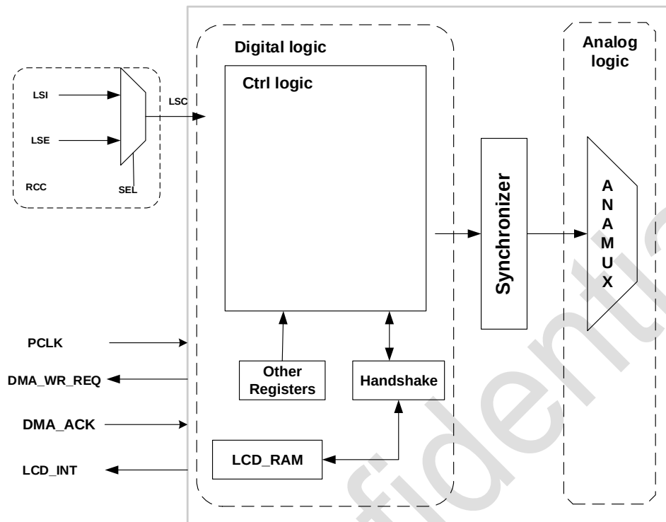
Figure 15-1 LCD Block Diagram
