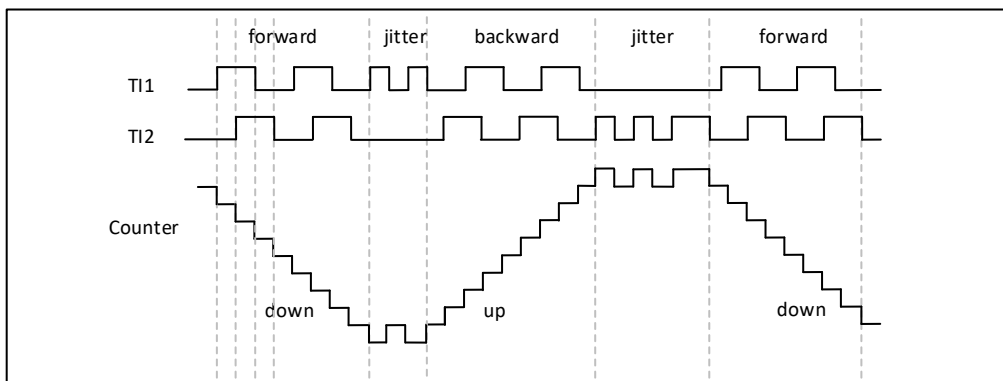
Figure 20-33 Example of encoder interface mode for IC1FP1 inversion
