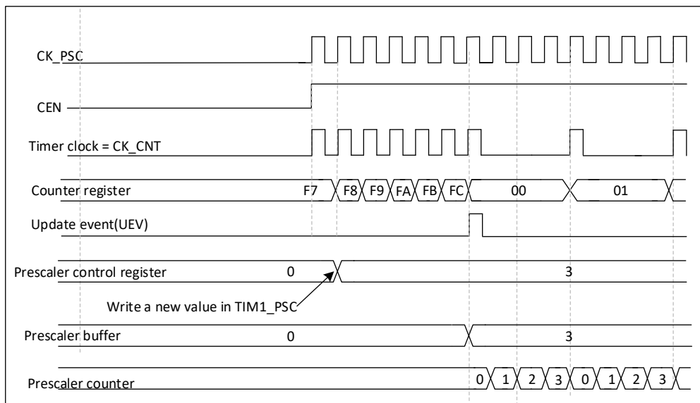
Figure 23-4 Timing diagram of the counter when the prescaler parameter changes from 1 to 4
