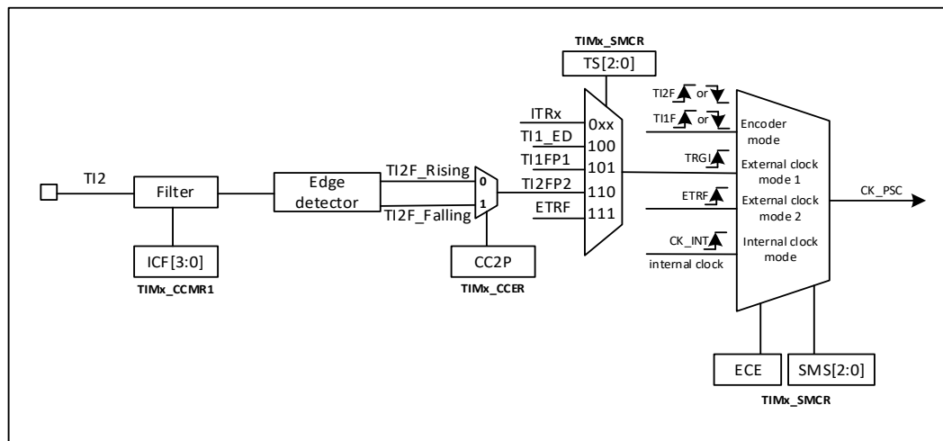
Figure 20-22 T12 Example of External Clock Connection
