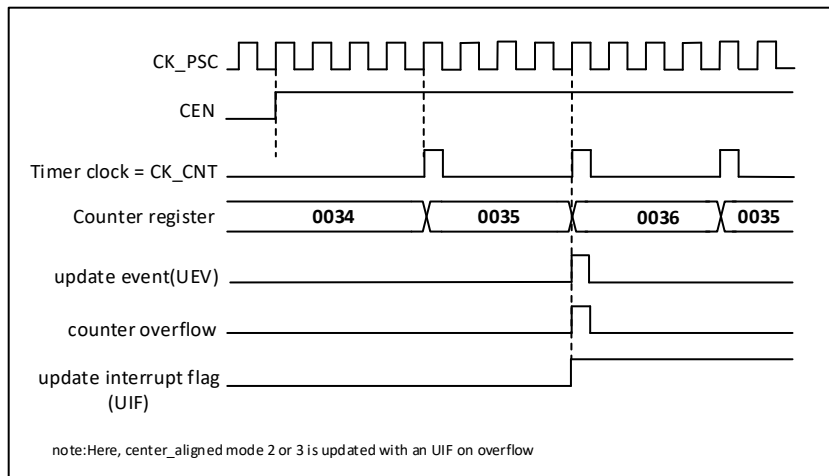
Figure 20-17 Counter timing diagram with internal clock divider factor of 4 and TIMx_ARR=0x36
