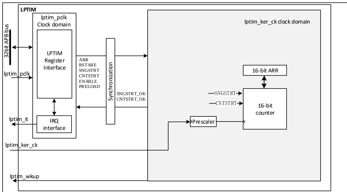
Figure 24-1 Low-power Timer Block Diagram
