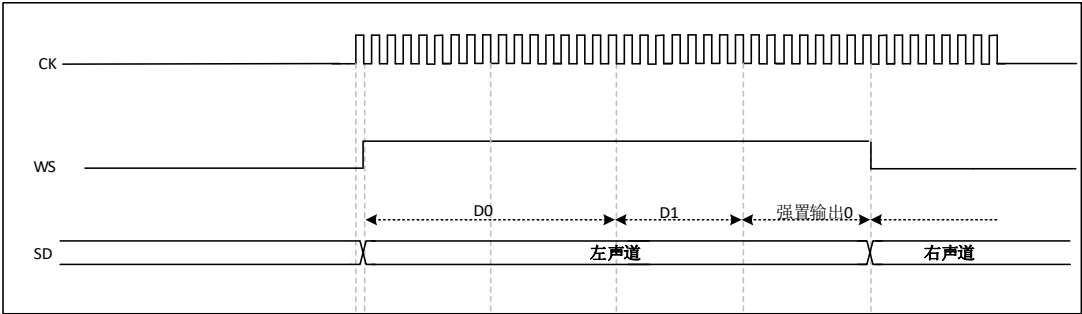
Figure 29-18 MSB-aligned 24-bit frame, CPKOL = 0
