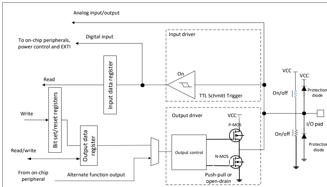
Figure 9-3 Output Configuration
