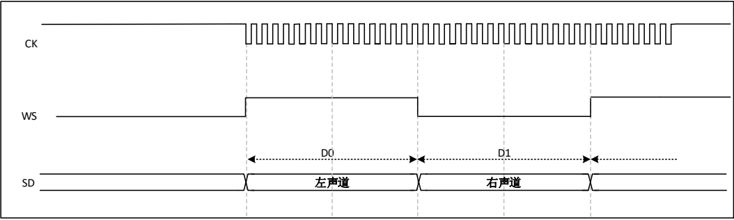
Figure 29-17 MSB-aligned 16-bit or 32-bit full precision, CPKOL = 1
