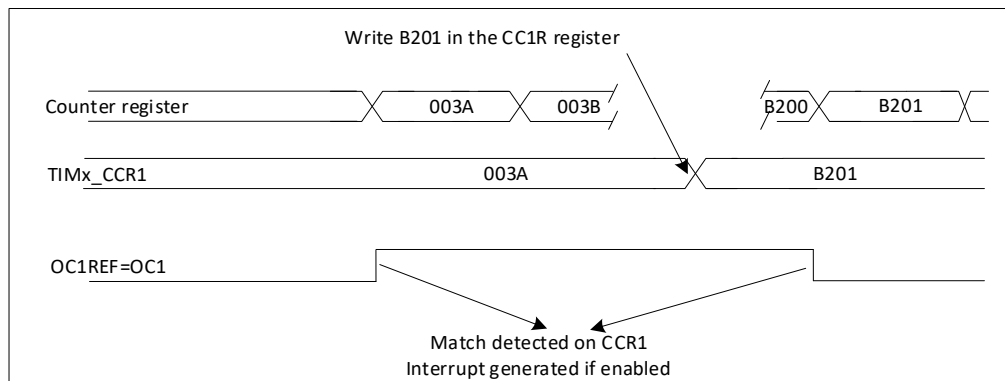
Figure 19-32 Output Compare Mode, Flip OC1
