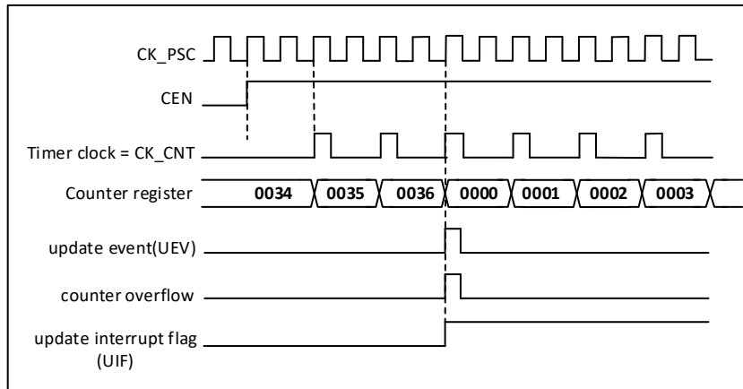
Figure 20-5 Timing diagram of the counter with internal clock division factor of 2
