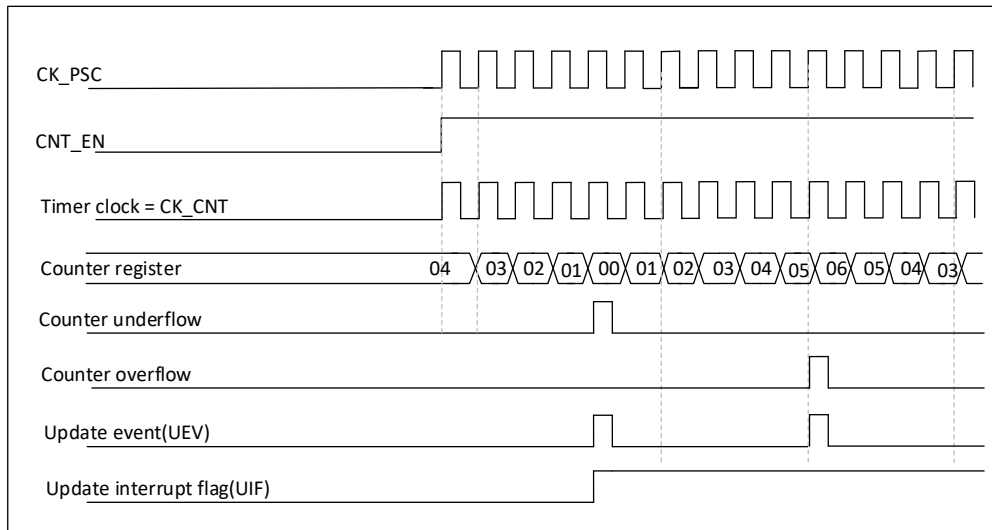
Figure 19-15 Counter timing diagram with internal clock divider factor of 1 and TIMx\_ARR = 0x6
