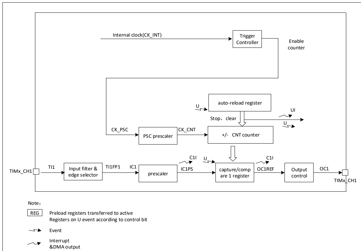
Figure 22-1 TIM14 Architecture Block Diagram
