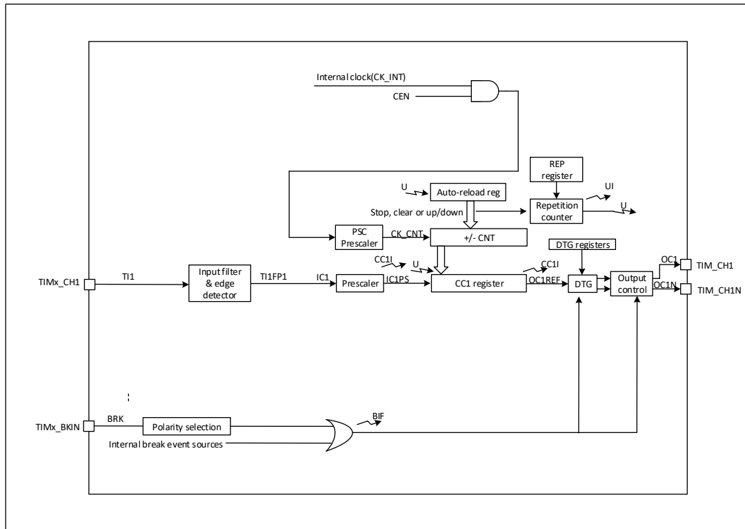
Figure 23-2 Block diagram of general-purpose control timer (TIM16_17) architecture
