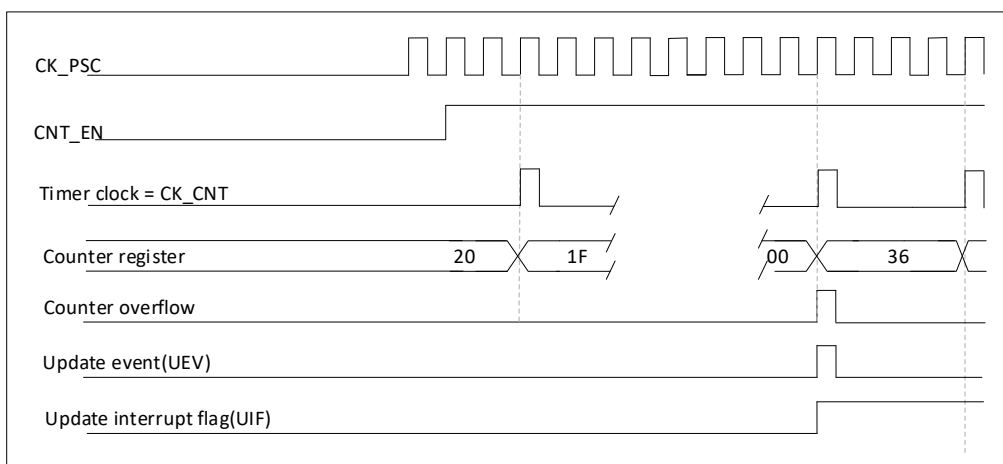
Figure 19-13 Timing diagram of the counter with internal clock dividing factor N
