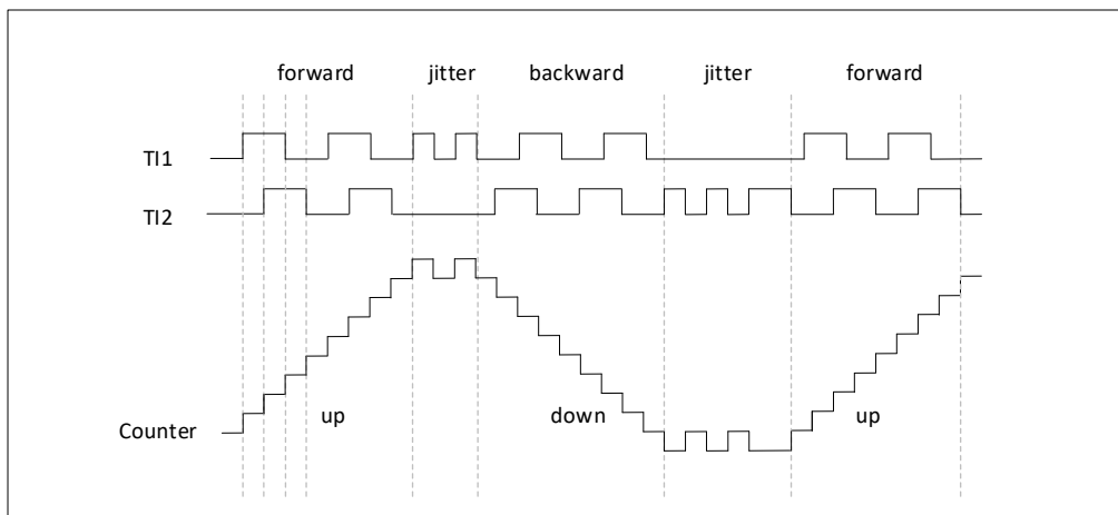
Figure 19-42 Example of counter operation in encoder mode
