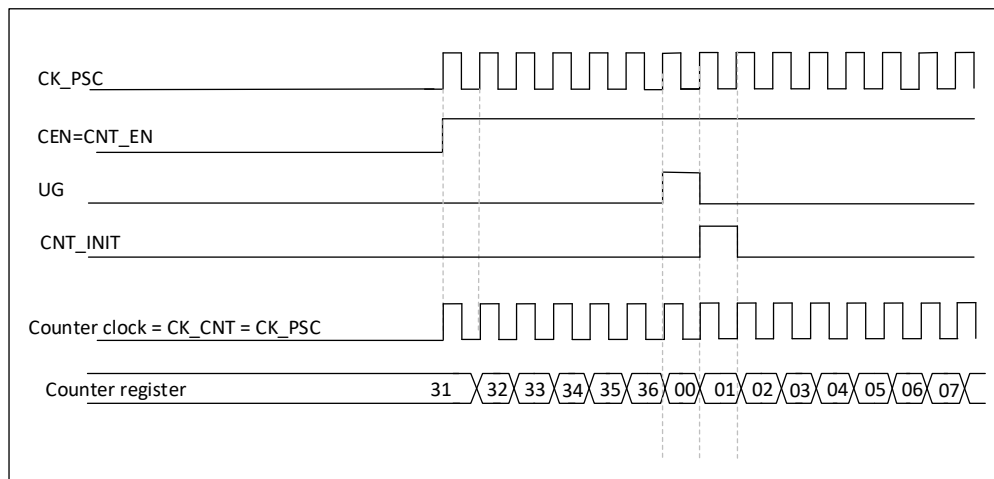
Figure 19-22 Control circuit in general mode with internal clock division factor of 1
