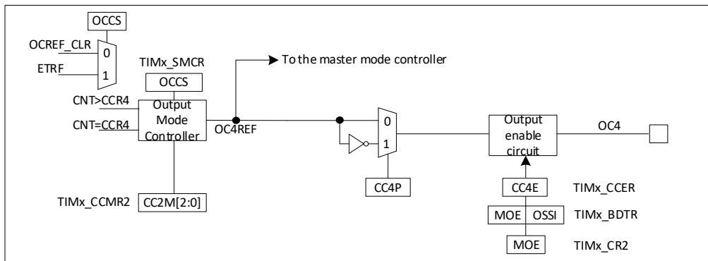
Figure 19-30 Output section of capture/compare channel (channel 4)
