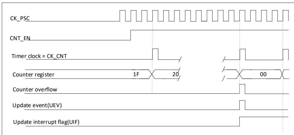
Figure 23-8 Counter timing diagram with internal clock division factor N
