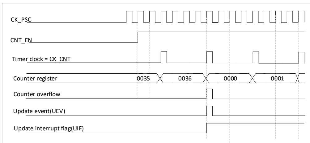
Figure 19-6 Timing diagram of the counter with internal clock divider factor of 4
