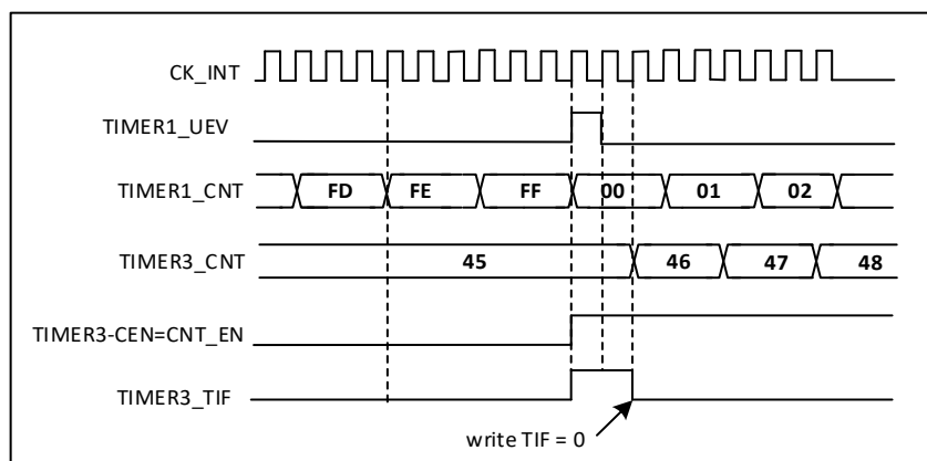
Figure 20-41 Trigger Timer 3 using Timer 1 update
