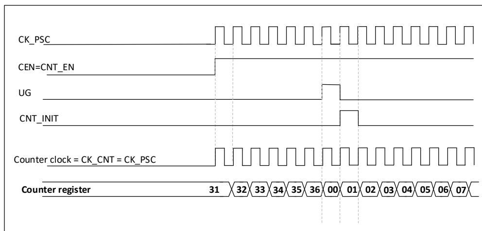
Figure 22-10 Control circuit in general mode with internal clock division factor of 1
