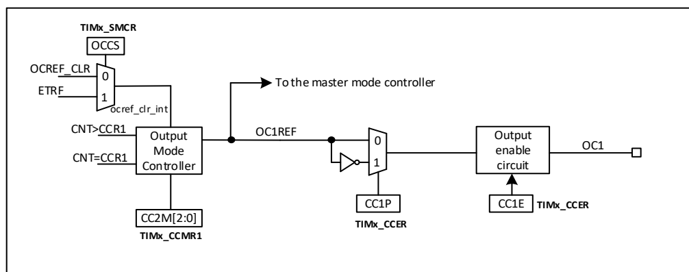
Figure 20-26 Output section of capture/compare channel (channel 1)
