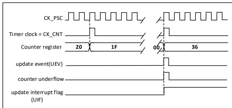
Figure 20-13 Timing diagram of the counter with internal clock dividing factor N
