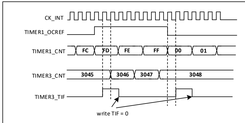
Figure 20-39 OC1REF of Timer 1 Controls Timer 3
