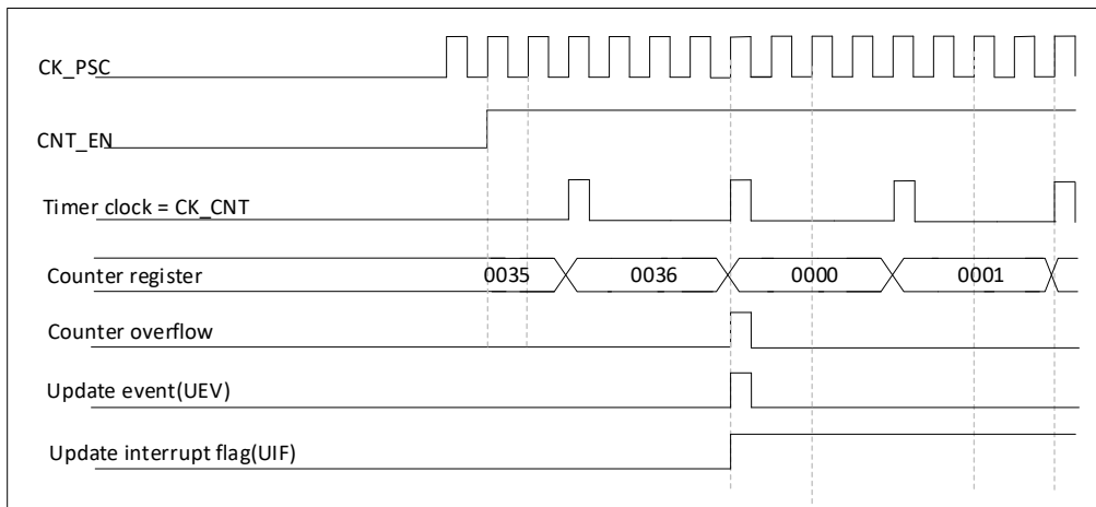
Figure 22-6 Timing diagram of the counter with internal clock divider factor of 4
