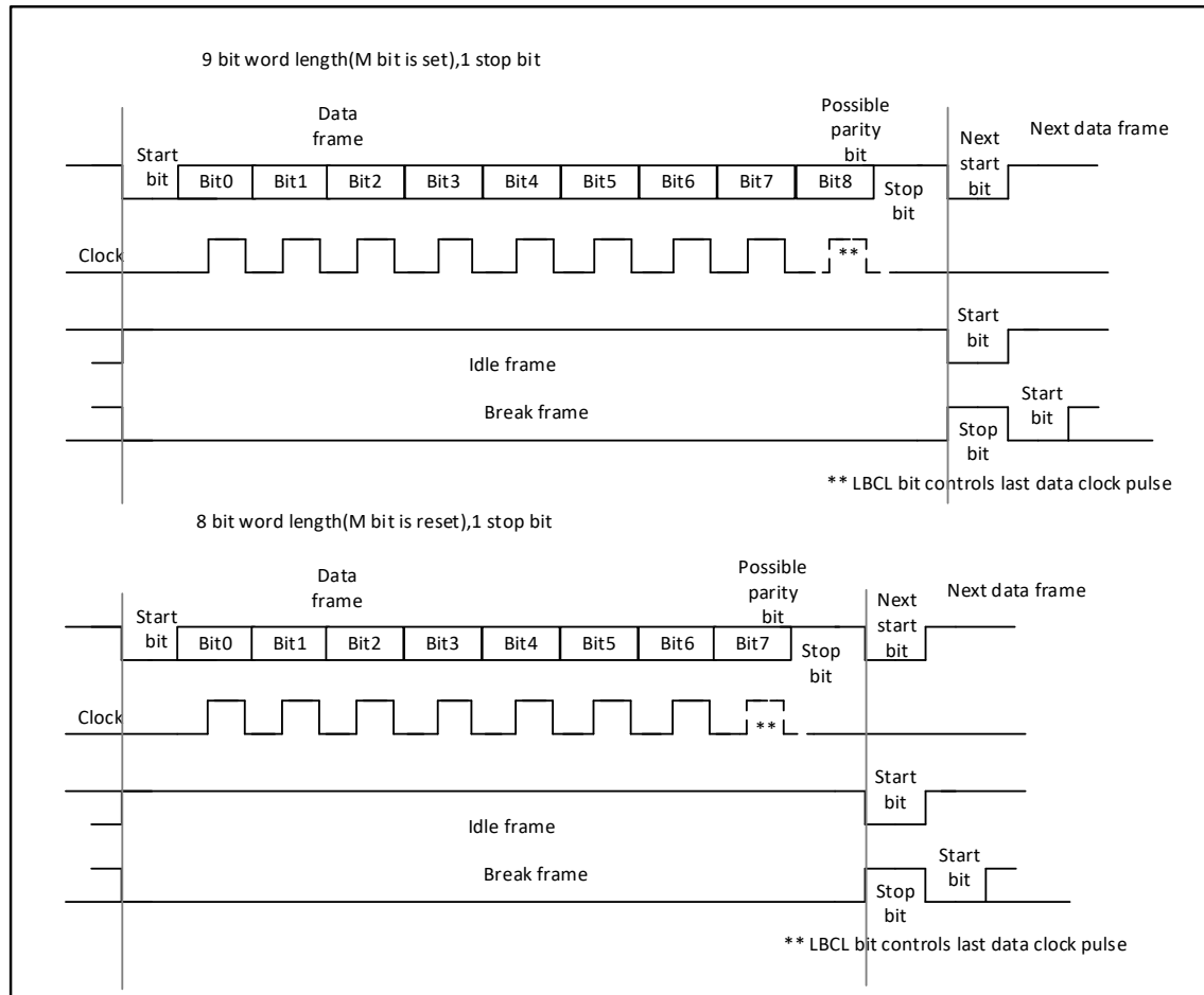
Figure 30-2 Word length setting
