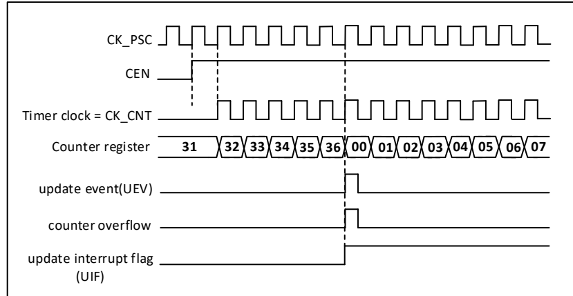
Figure 20-4 Timing diagram of the counter with internal clock division factor of 1
