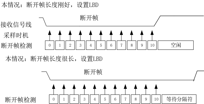
Figure 30-10 Case where the break frame length is sufficient in LIN mode
