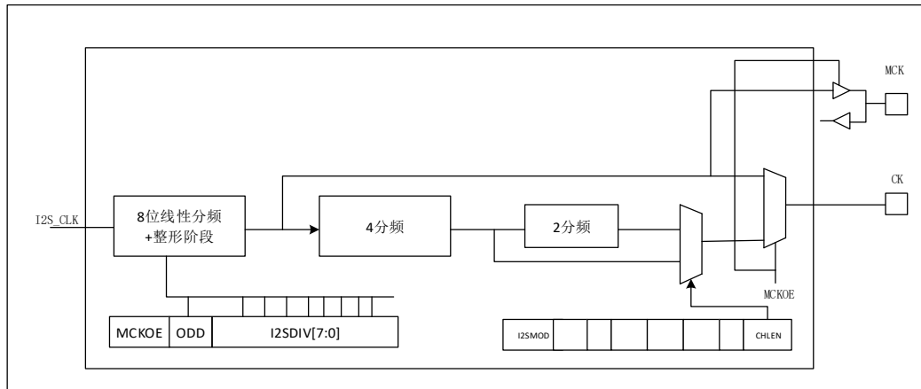
Figure 29-33 I2S Clock Generator Structure
