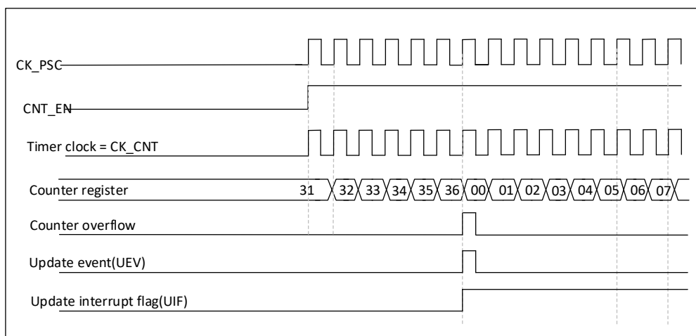
Figure 19-4 Timing diagram of the counter with internal clock division factor of 1
