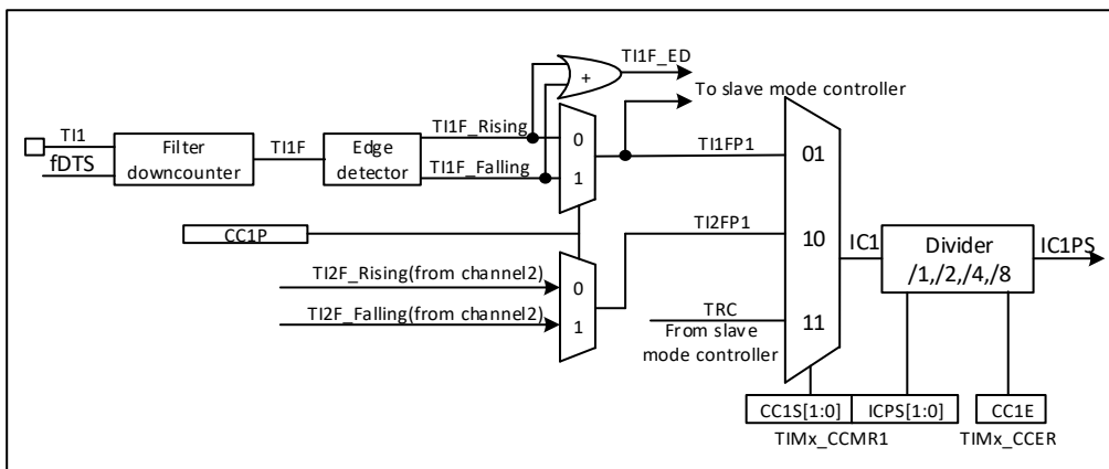
Figure 23-15 Capture/compare channel (e.g., input section of Channel 1)
