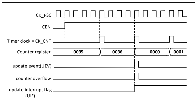
Figure 20-6 Timing diagram of the counter with internal clock divider factor of 4
