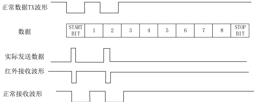
Figure 30-19 IrDA data modulation (3/16) - Normal mode
