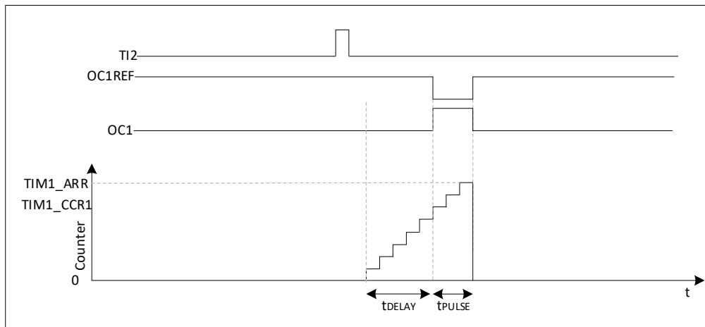
Figure 22-14 Example of single-pulse mode
