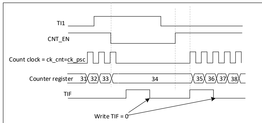
Figure 23-28 Control circuit in gated mode
