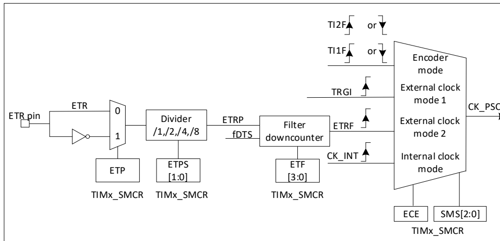
Figure 19-25 TI2 External Trigger Input Block Diagram
