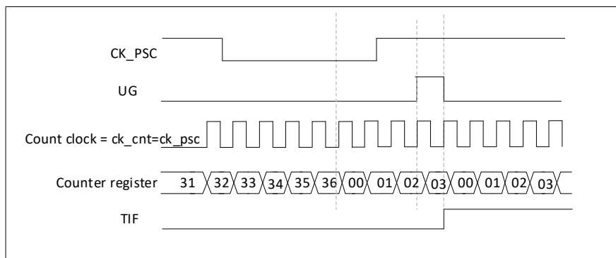
Figure 23-27 Control circuit in reset mode
