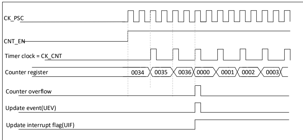
Figure 19-5 Timing diagram of the counter with internal clock divider factor of 2
