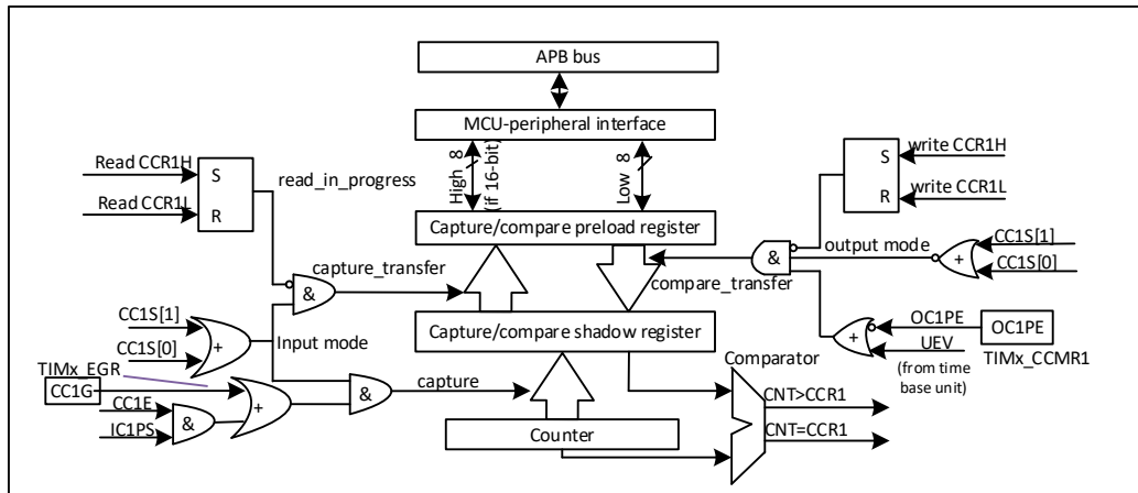
Figure 20-25 Capture/Compare Channel 1 Main Circuitry
