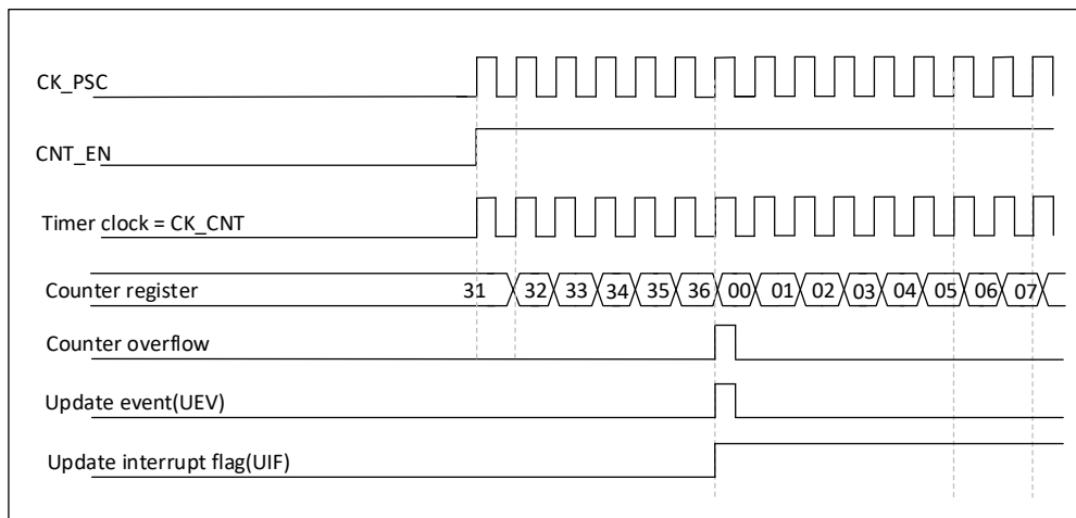
Figure 23-5 Counter timing diagram with internal clock division factor 1
