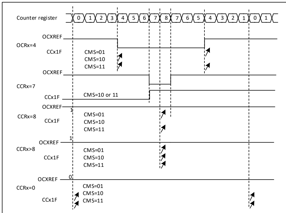
Figure 20-30 Centrally aligned PWM waveform (APR=8)
