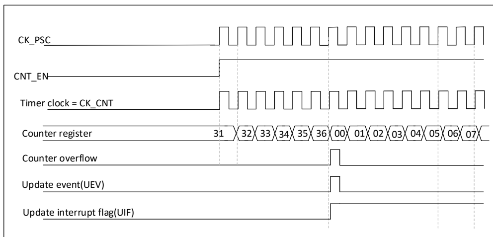
Figure 22-4 Timing diagram of the counter with internal clock division factor of 1
