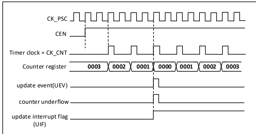
Figure 20-16 Timing diagram of the counter with internal clock divider factor of 2
