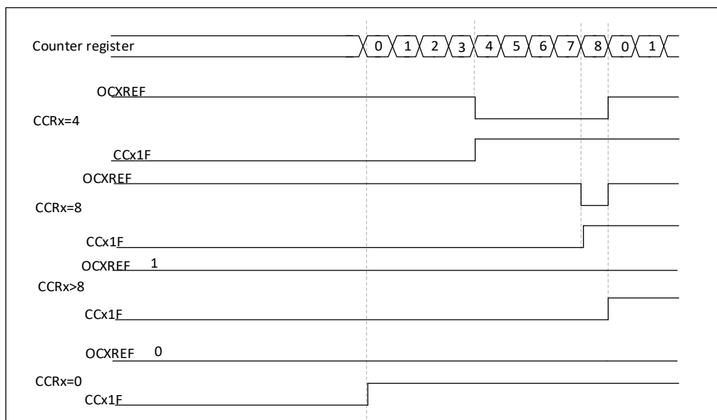
Figure 22-13 Edge-aligned PWM waveform (ARR=8)
