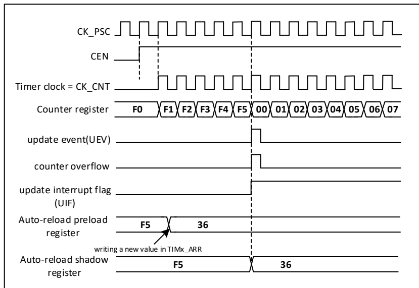
Figure 20-9 Counter timing diagram, update event when ARPE=1 (preloaded with TIMx_ARR)
