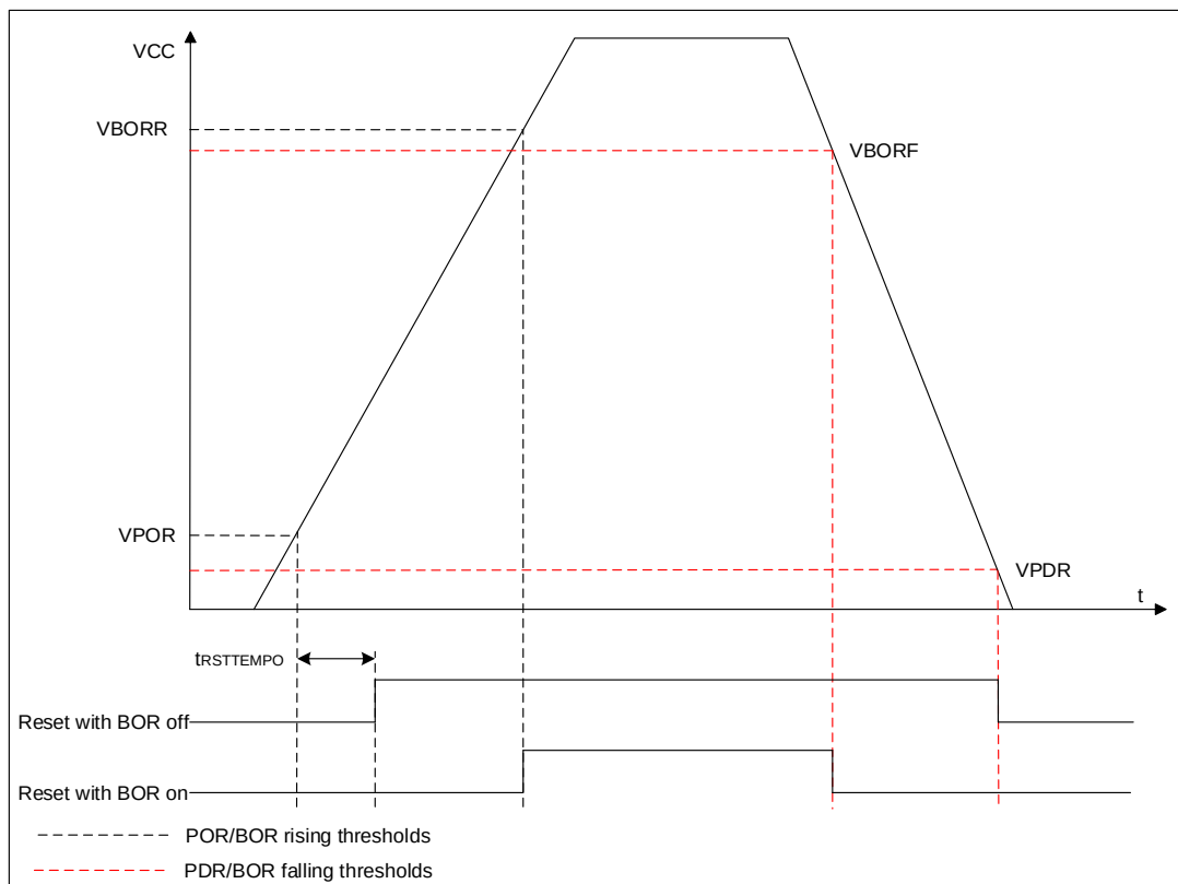
Figure 5-2 POR/PDR/BOR thresholds
