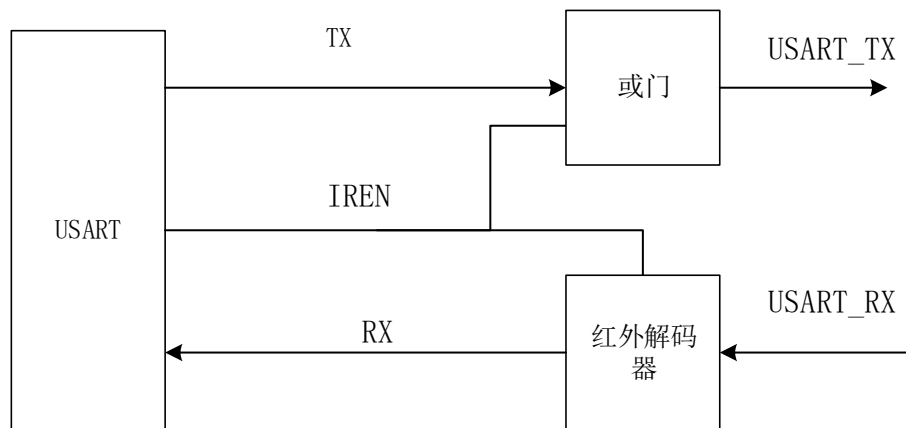
Figure 30-18 IrDA SIR ENDEC block diagram
