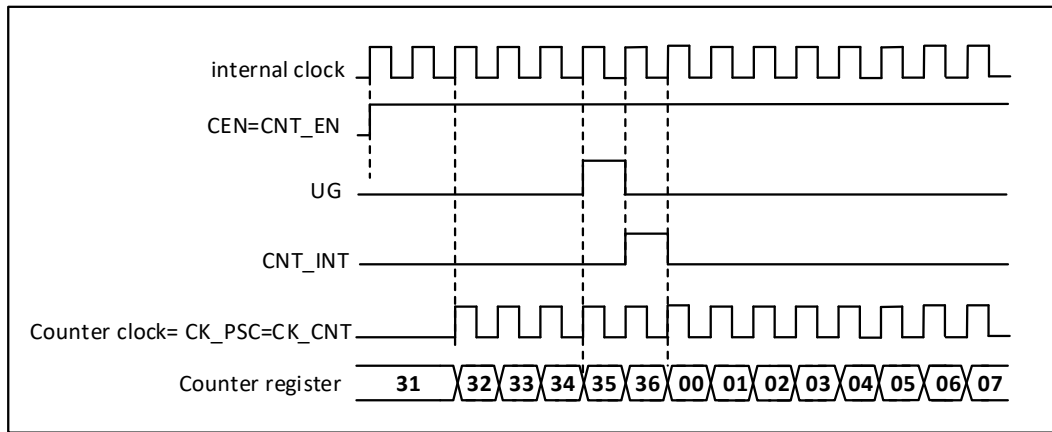
Figure 20-21 Control circuit in general mode with internal clock division factor of 1
