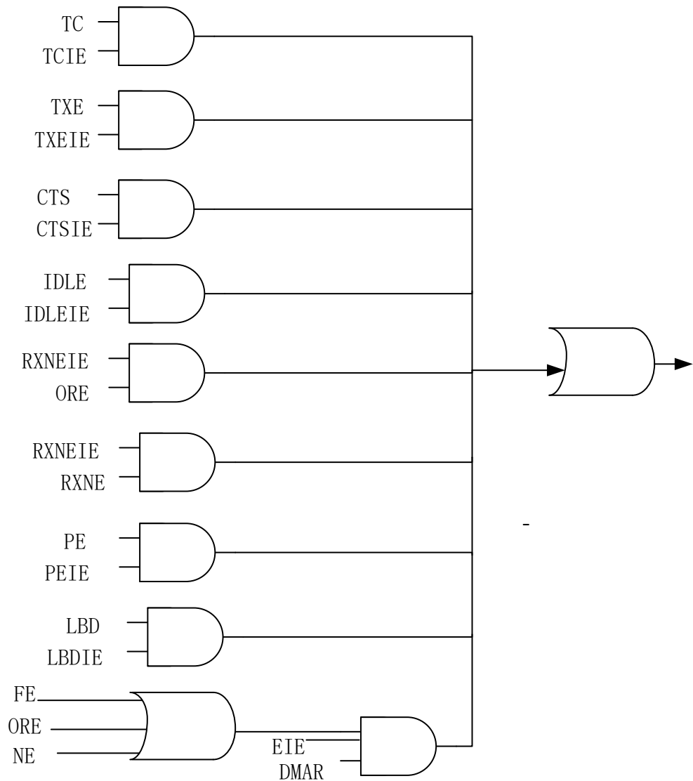
Figure 30-24 USART Interrupt Mapping Diagram
