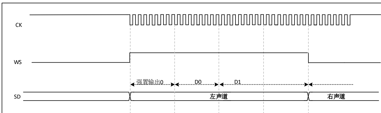
Figure 29-25 LSB-aligned 24-bit data, CKPOL=1
