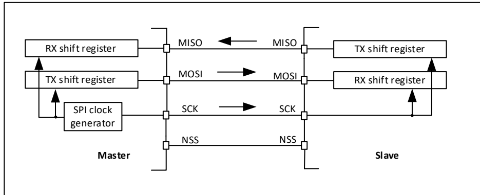
Figure 29-2 Full-duplex single master/single slave application
