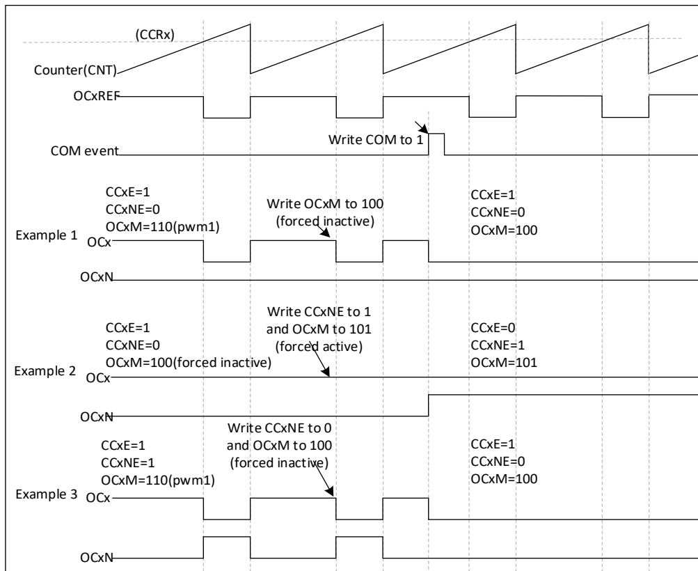
Figure 19-40 Six-step generation, COM example (OSSR=1)
