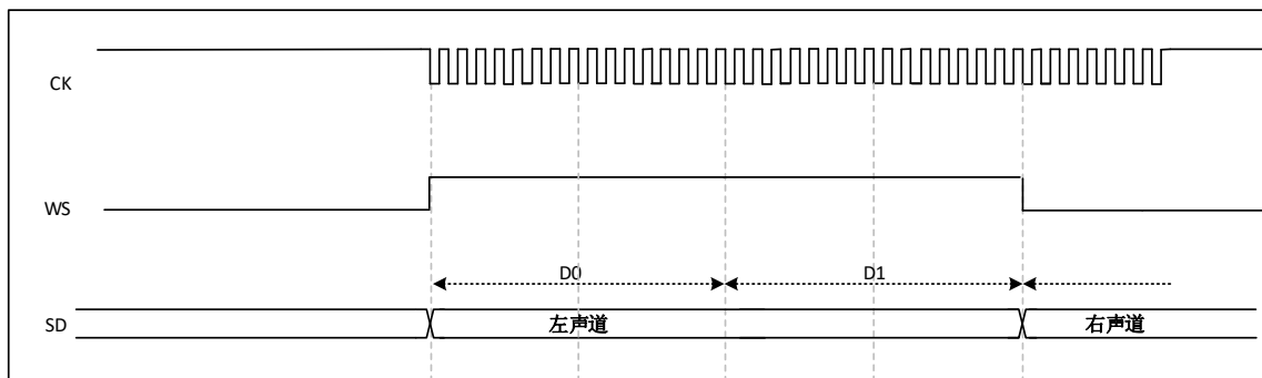
Figure 29-16 MSB-aligned 16-bit or 32-bit full precision, CPKOL = 0
