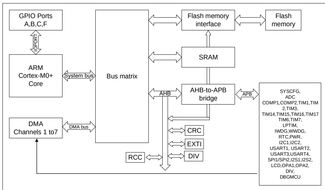
Figure 3-1 System Architecture
