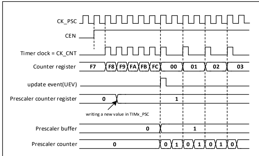
Figure 20-2 Timing diagram of the counter when the prescaler parameter is changed from 1 to 2
