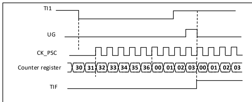
Figure 20-34 Control circuit in reset mode
