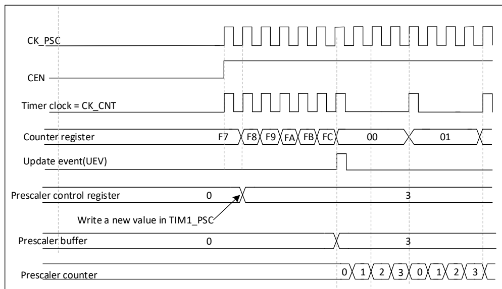
Figure 22-3 Timing diagram of the counter when the prescaler parameter is changed from 1 to 4
