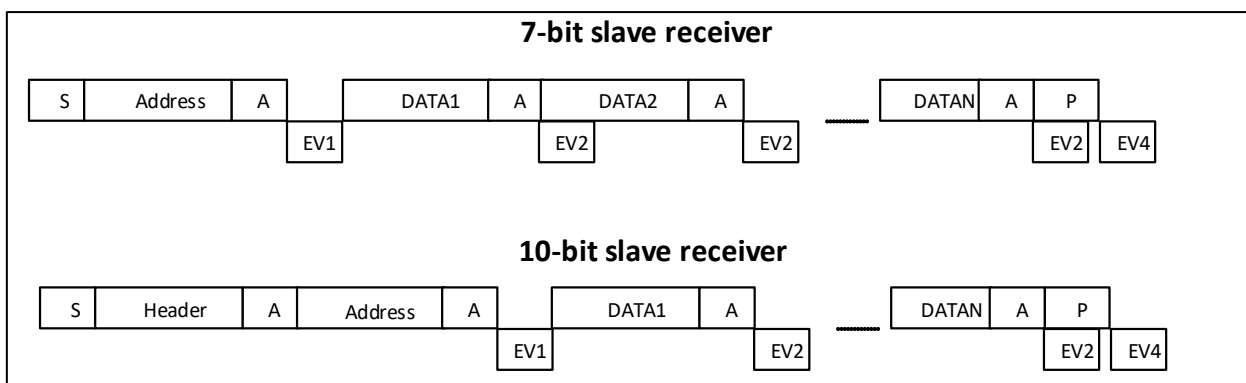
Figure 28-4 Transmission sequence diagram from the receiver
