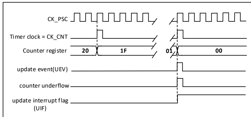
Figure 20-18 Timing diagram of the counter with internal clock dividing factor N
