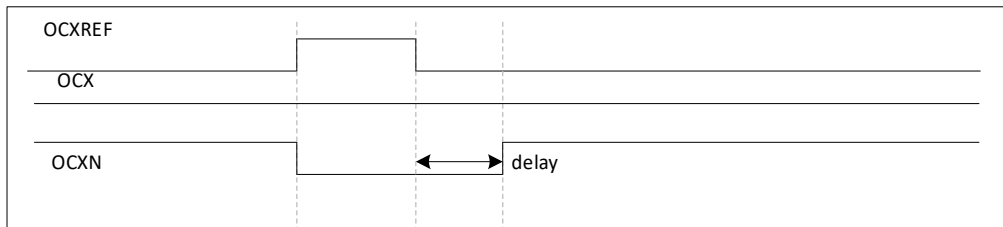
Figure 23-24 Dead-time waveform with delay greater than positive pulse
