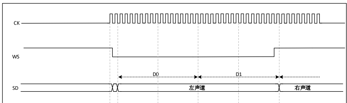
Figure 29-11 I2S Philips protocol waveform (16/32-bit full precision, CKPOL = 0)
