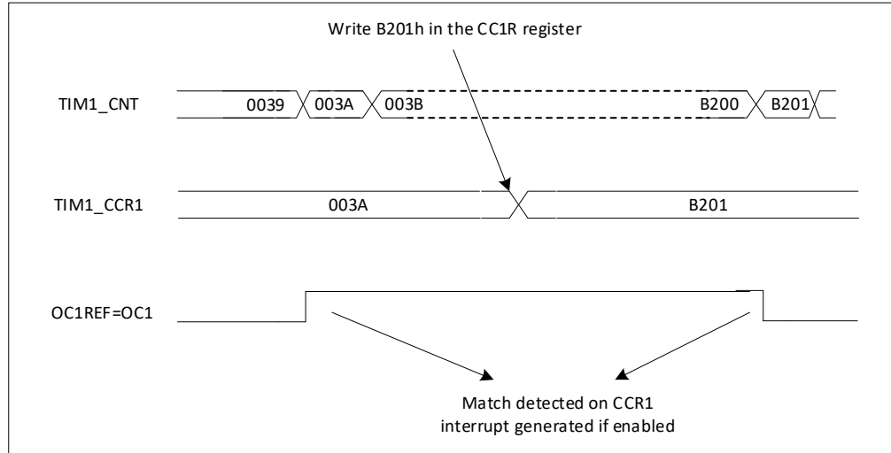
Figure 22-12 Output Compare Mode, Flip OC1
