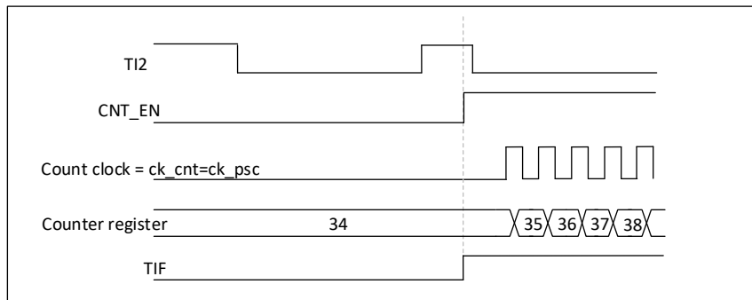
Figure 23-29 Control circuit in trigger mode
