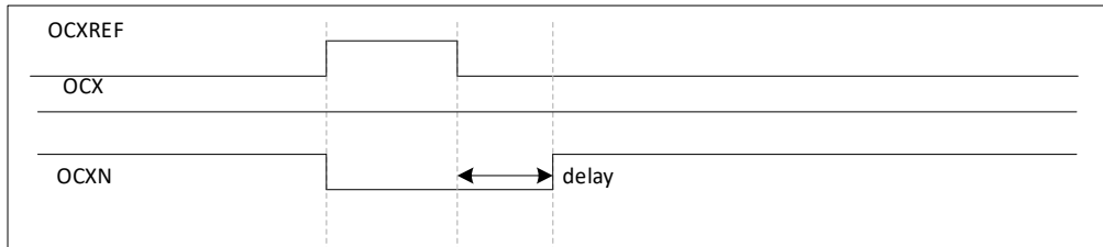
Figure 19-37 Deadband waveform delay is greater than positive pulse
