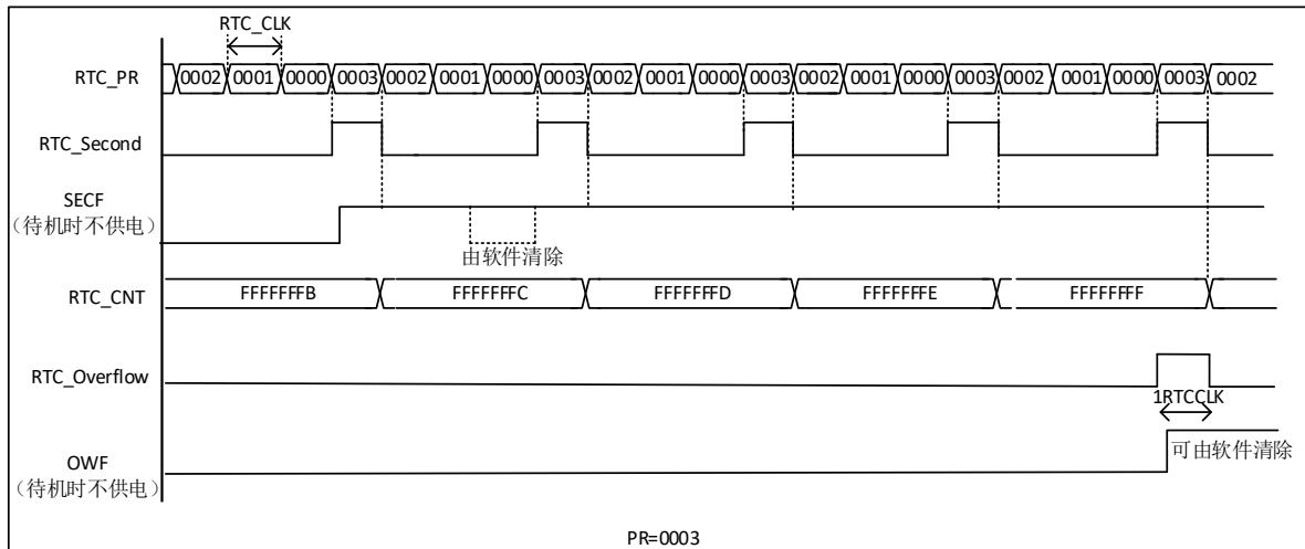
Figure 27-3 Example of RTC Overflow Waveform, PR=0003
