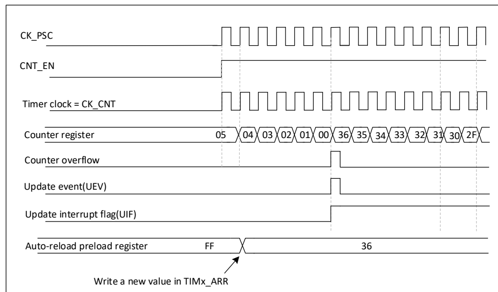
Figure 19-14 Counter Timing Diagram, Update Events When Cycle Counter is Not Used
