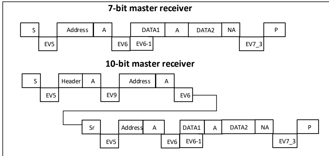
Figure 28-8 Method 2: Timing diagram for master mode transmission when N=2
