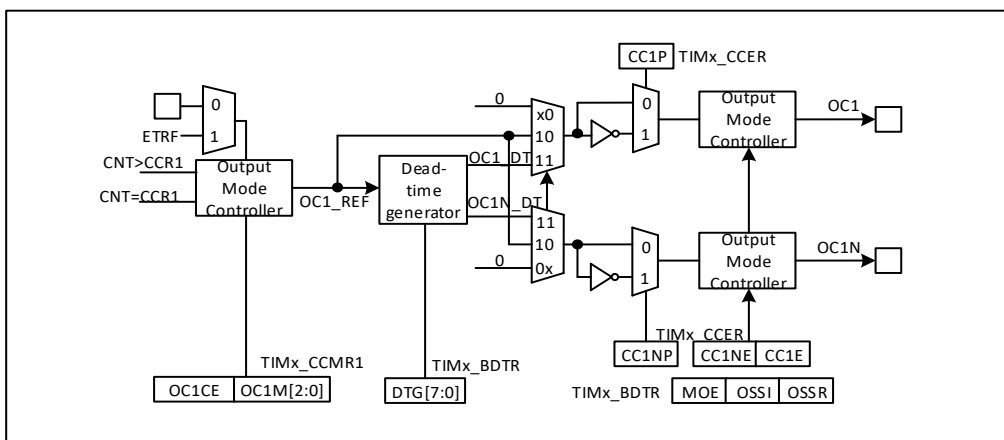
Figure 23-17 Output section of the capture/compare channel (Channels 1 to 3)
