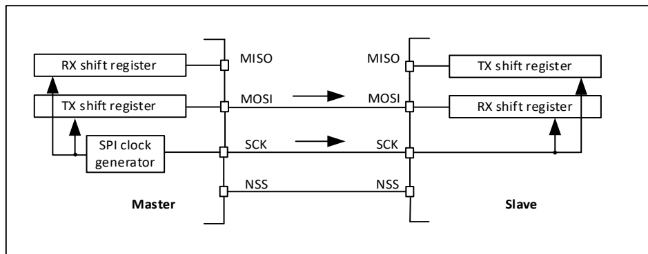
Figure 29-4 Simplex Single Slave/Single Master Application (Master is in transmit-only mode/Slave is in receive-only mode)
