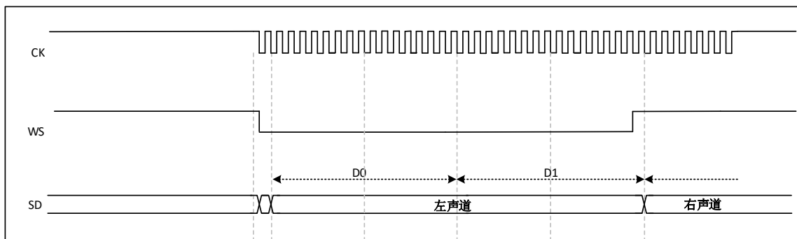
Figure 29-12 I2S Philips protocol waveform (16/32-bit full precision, CKPOL = 0)
