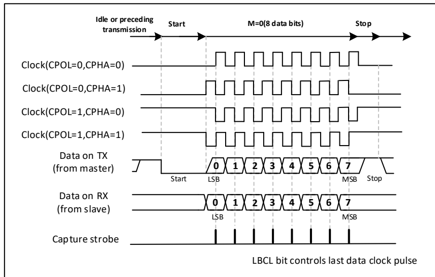
Figure 30-13 Example of USART data clock timing (M=0)
