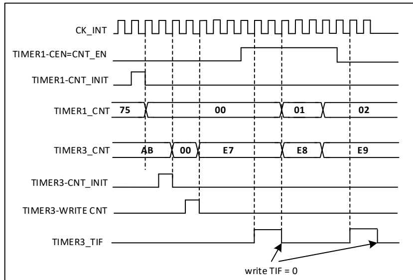
Figure 23-37 Timer 2 can be controlled by enabling Timer 1
