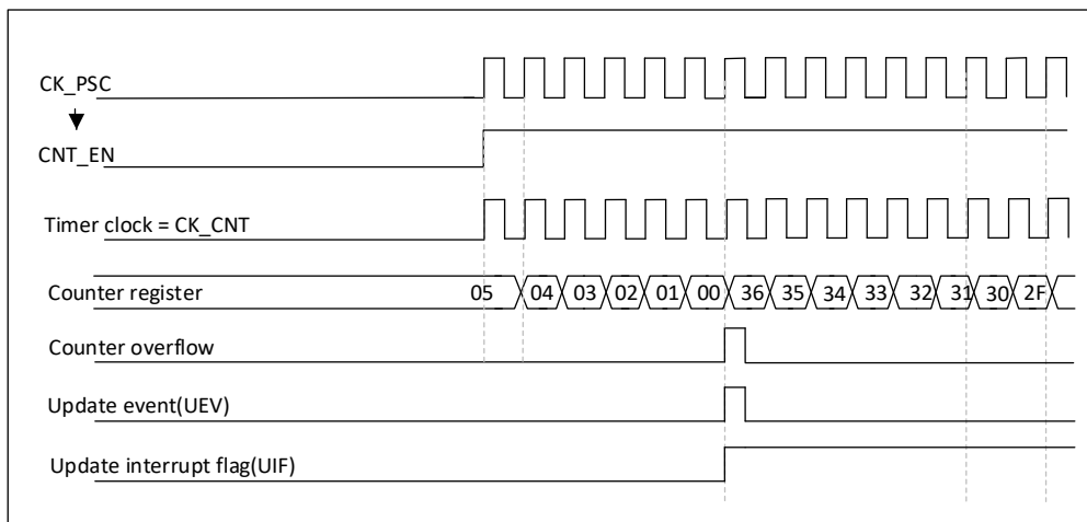
Figure 19-10 Timing diagram of the counter with internal clock division factor of 1
