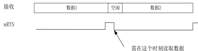
Figure 30-22 RTS flow control
