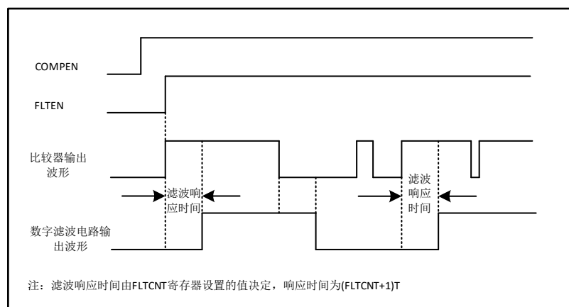
Figure 16-3 Comparator Filtering
