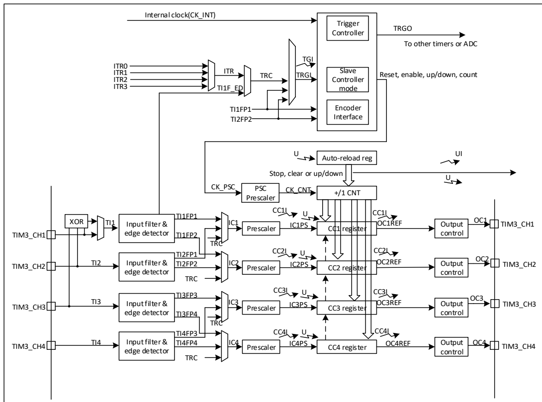
Figure 20-1 General Purpose Timer Architecture
