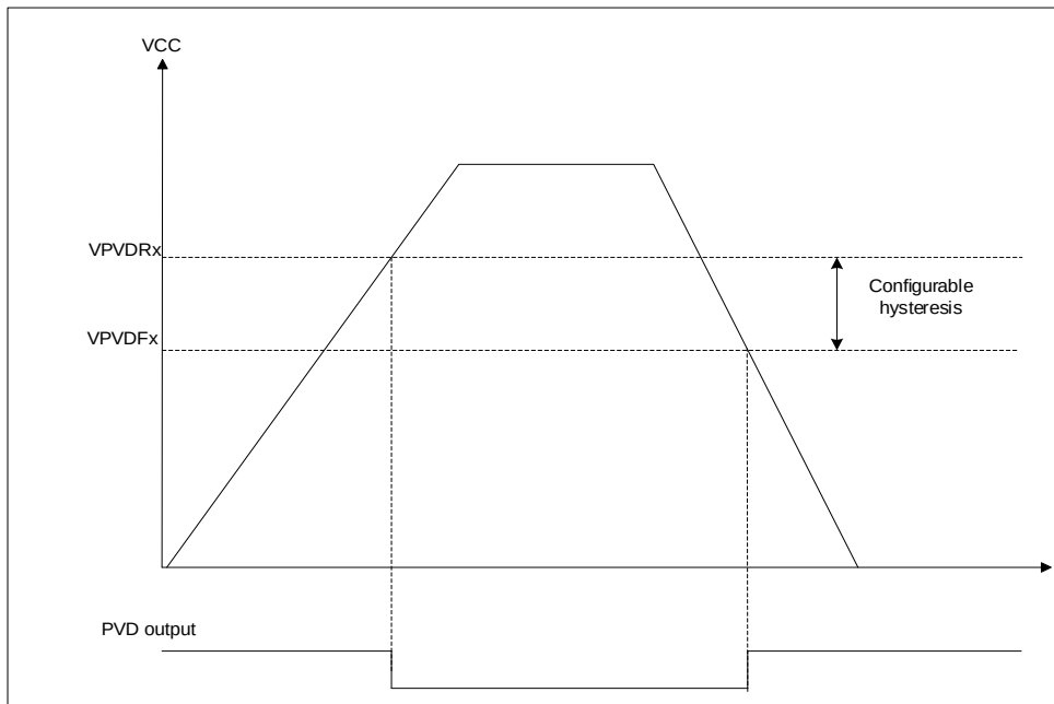
Figure 5-3 PVD Threshold
