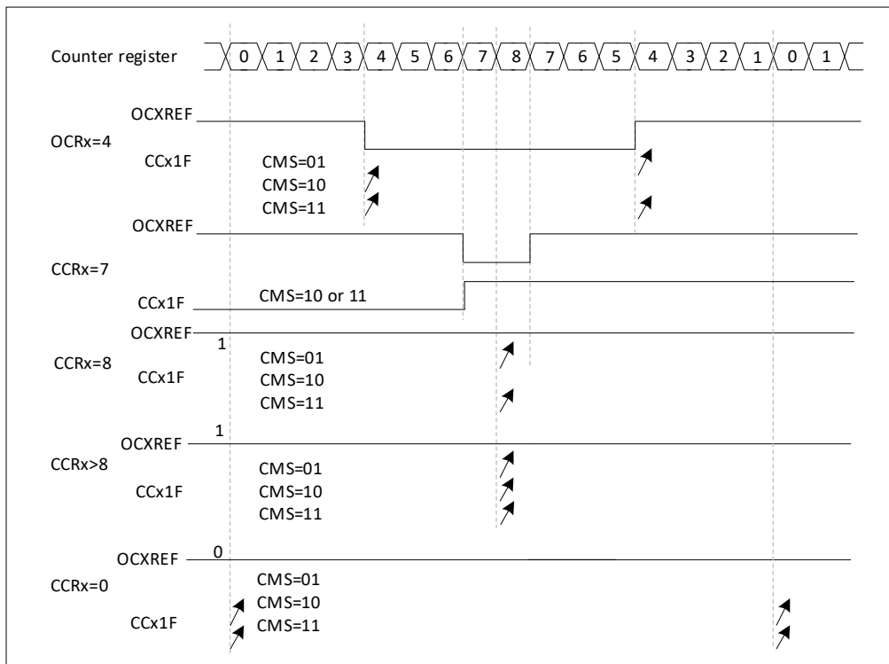
Figure 19-34 Centrally aligned PWM waveform (APR=8)
