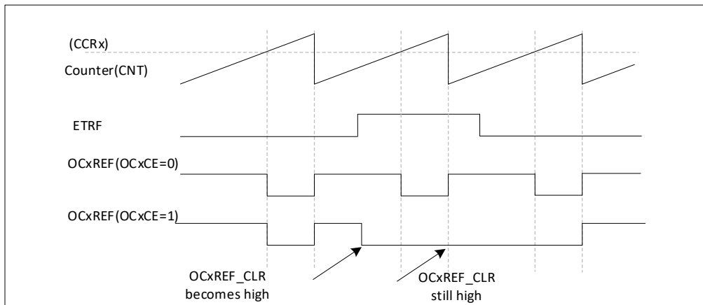
Figure 19-39 Clear OCxREF of TIM1
