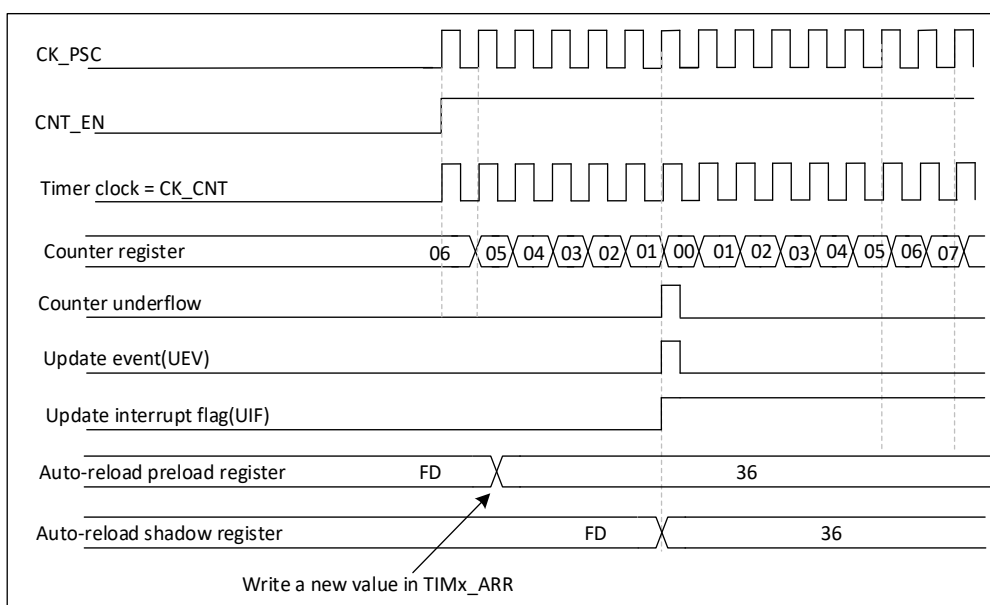
Figure 19-19 Counter timing diagram, update event at ARPE=1 (counter underflow)
