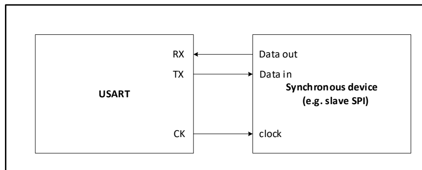
Figure 30-12 Example of USART synchronous transmission
