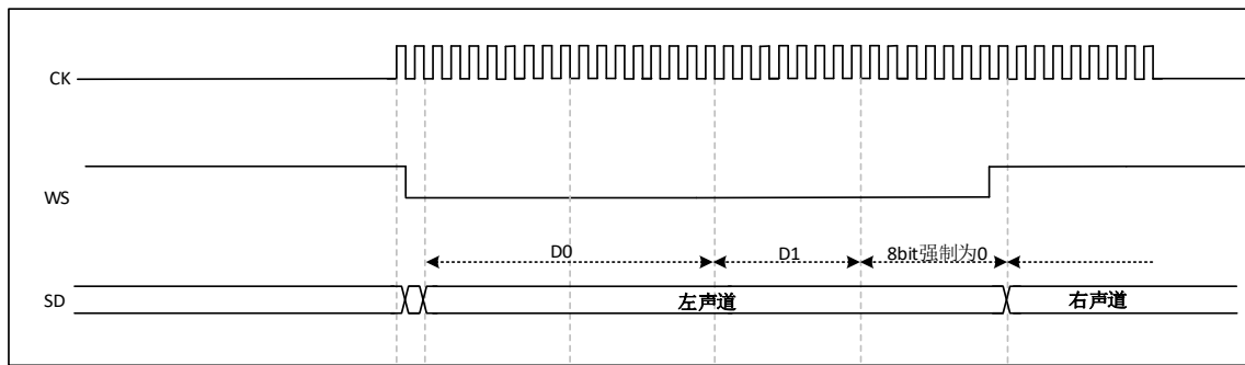
Figure 29-13 I2S Philips protocol standard waveform (24-bit frame, CKPOL = 0)
