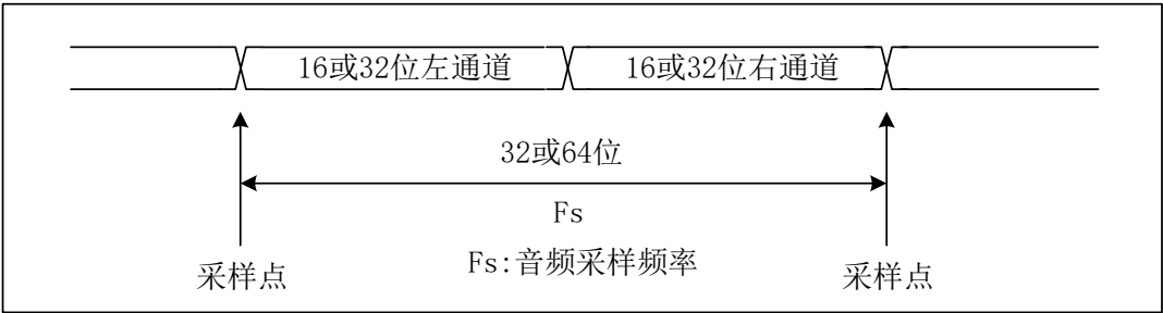
Figure 29-32 Audio Sampling Definition
