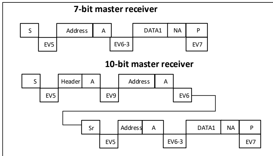
Figure 28-9 Method 2: Timing for master transmission when N=1
