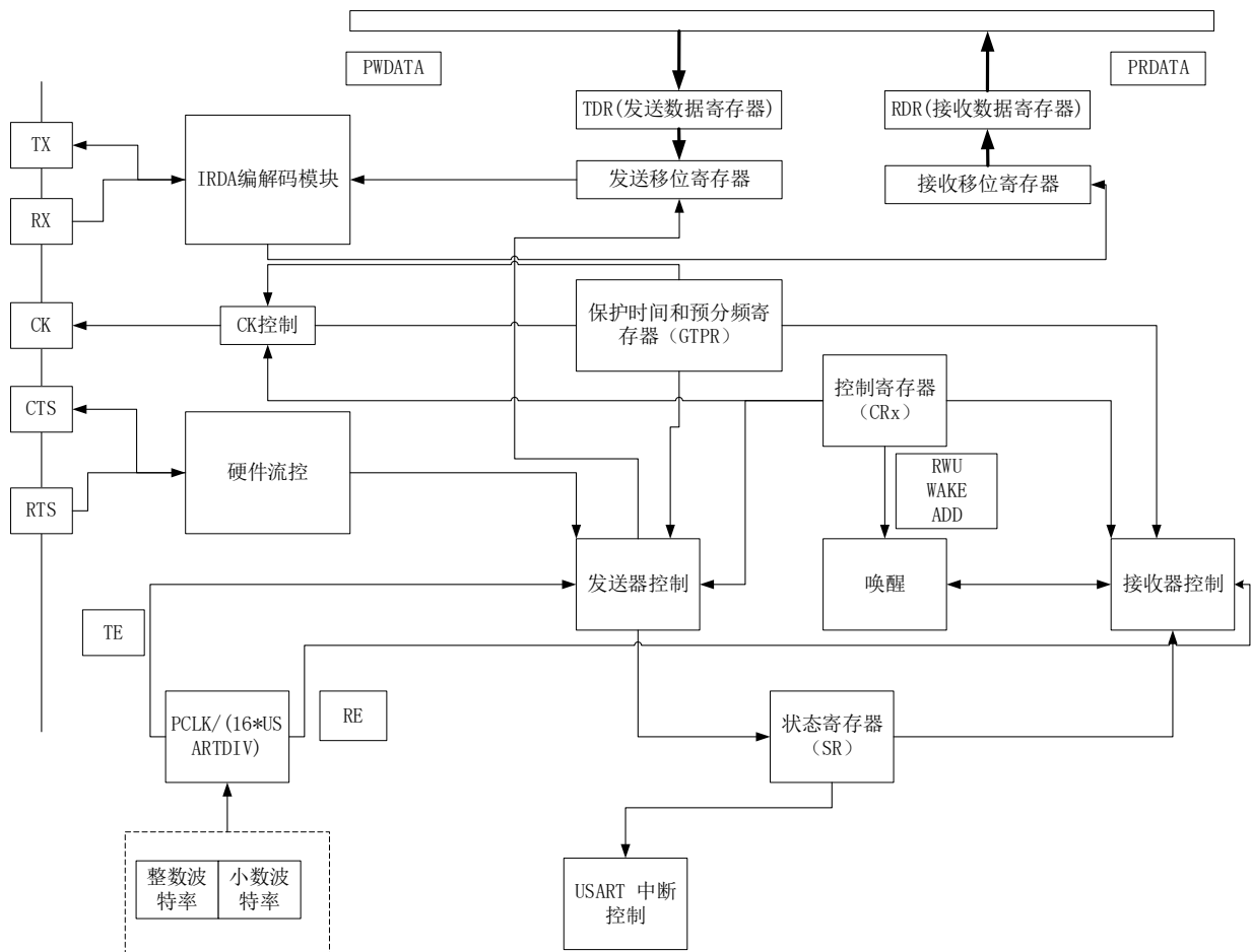
Figure 30-1 USART block diagram
