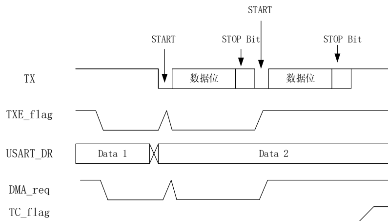
Figure 30-20 Using DMA for transmission
