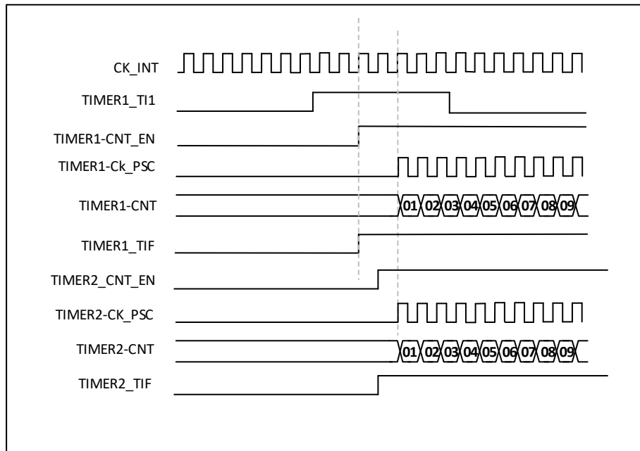
Figure 23-40 Using timer 1's TI1 input to trigger timer 1 and timer 2
