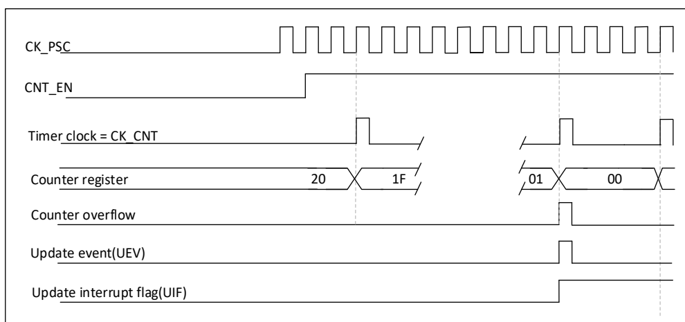
Figure 19-18 Timing diagram of the counter with internal clock dividing factor N
