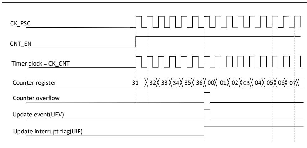
Figure 23-9 Counter timing diagram showing update events when ARPE=0 (TIMx_ARR not preloaded)
