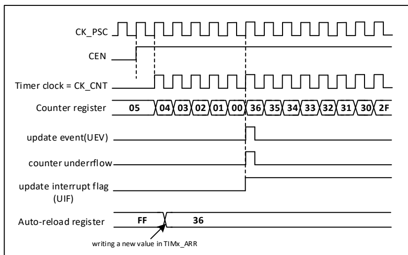
Figure 20-14 Counter Timing Diagram, Update Events When Cycle Counter is Not Used
