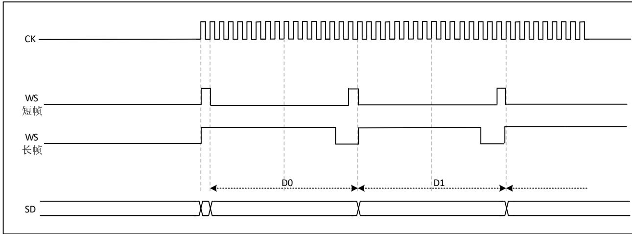
Figure 29-28 PCM standard waveform (16-bit, CKPOL=0)
