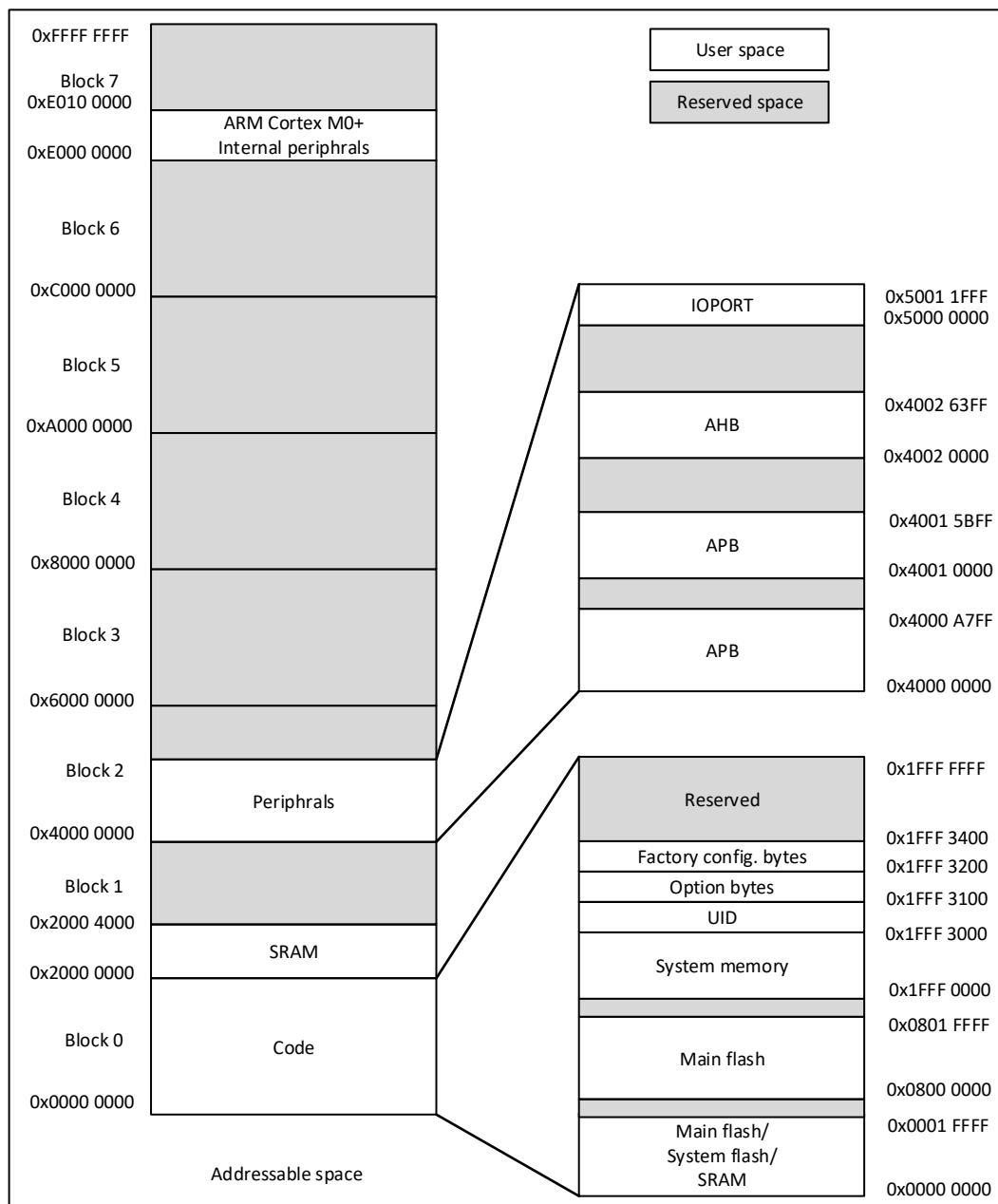
Figure 3-2 Memory mapping
