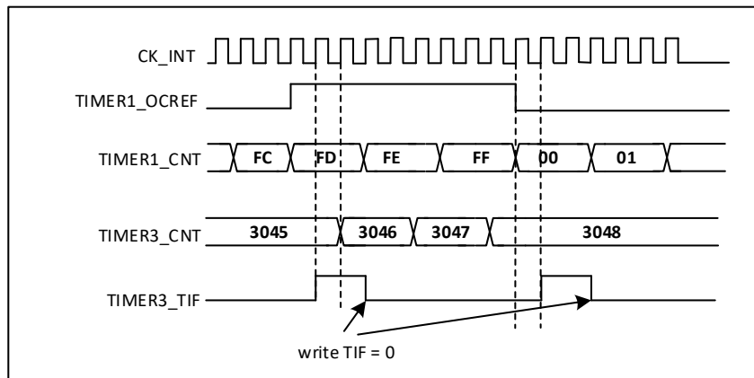
Figure 23-36 Timer 1's OC1REF controls Timer 2
