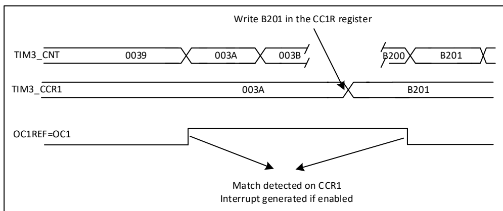
Figure 20-28 Output Compare Mode, Flip OC1
