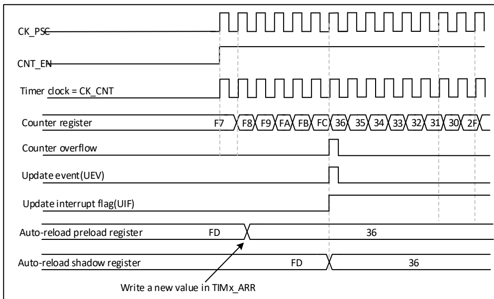
Figure 20-20 Counter timing diagram, update event at ARPE=1 (counter overflow)
