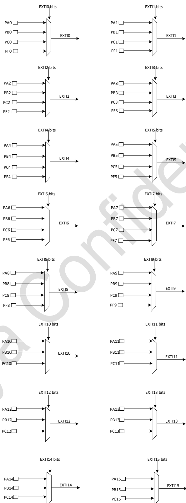
Figure 12-2 External Interrupt/Event GPIO Image
