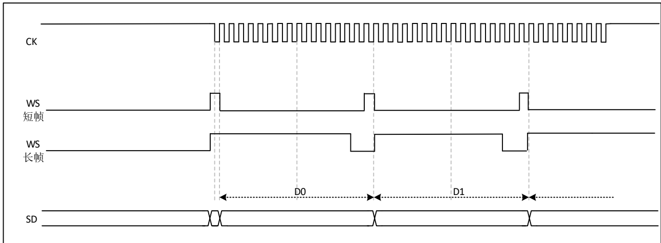
Figure 29-29 PCM Standard Waveform (16-bit, CKPOL=1)
