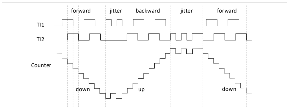
Figure 19-43 TI1FP1 Inverted Encoder Interface Mode Example
