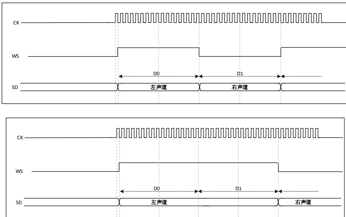
Figure 29-16 MSB-aligned 16-bit or 32-bit full precision, CPKOL = 0
