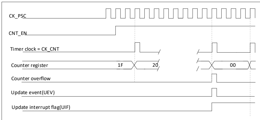
Figure 21-7 Timing diagram of the counter with internal clock dividing factor N
