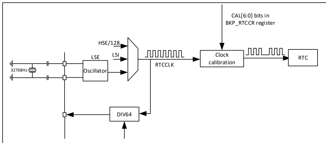
Figure 27-4 RTC Calibration Diagram
