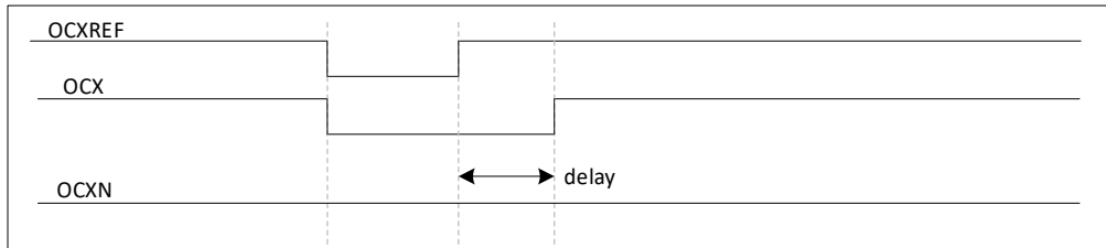
Figure 23-23 Dead-time waveform with delay greater than negative pulse
