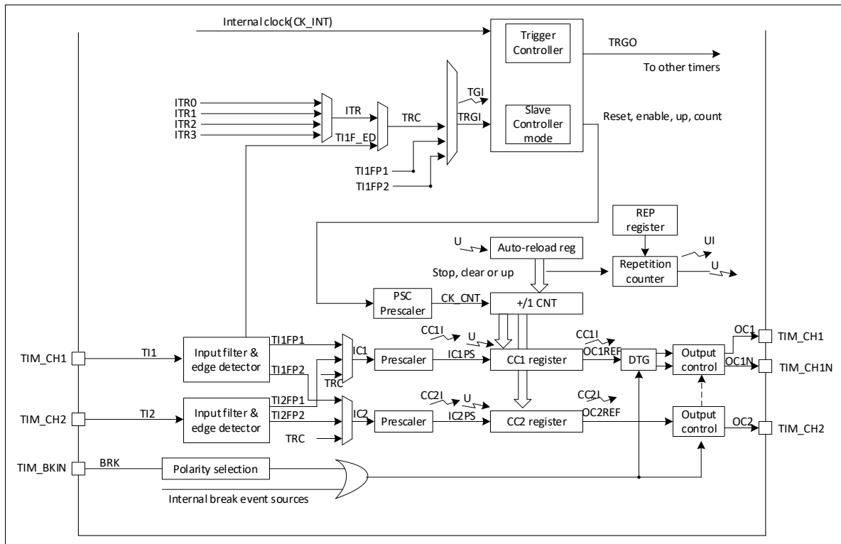
Figure 23-1 Block diagram of general-purpose control timer (TMI15) architecture
