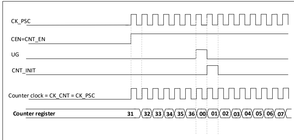
Figure 21-10 Control circuit in general mode with internal clock division factor of 1
