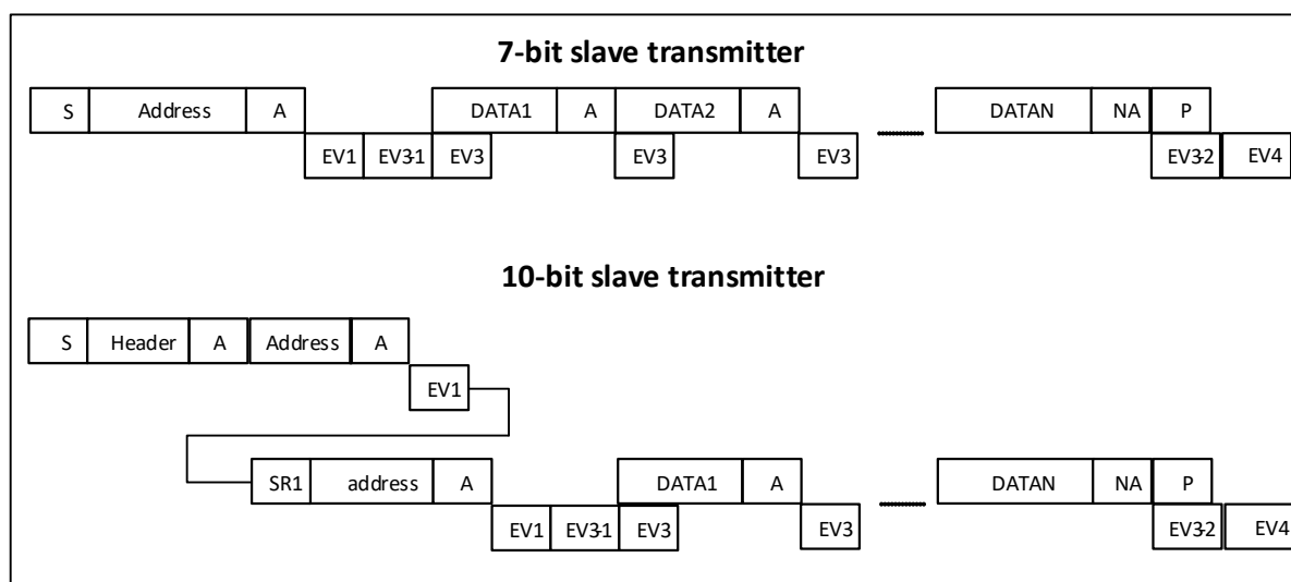
Figure 28-3 Transmission sequence diagram from transmitter
