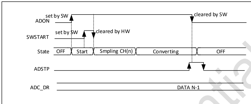
Figure 14-3 Stop timing
