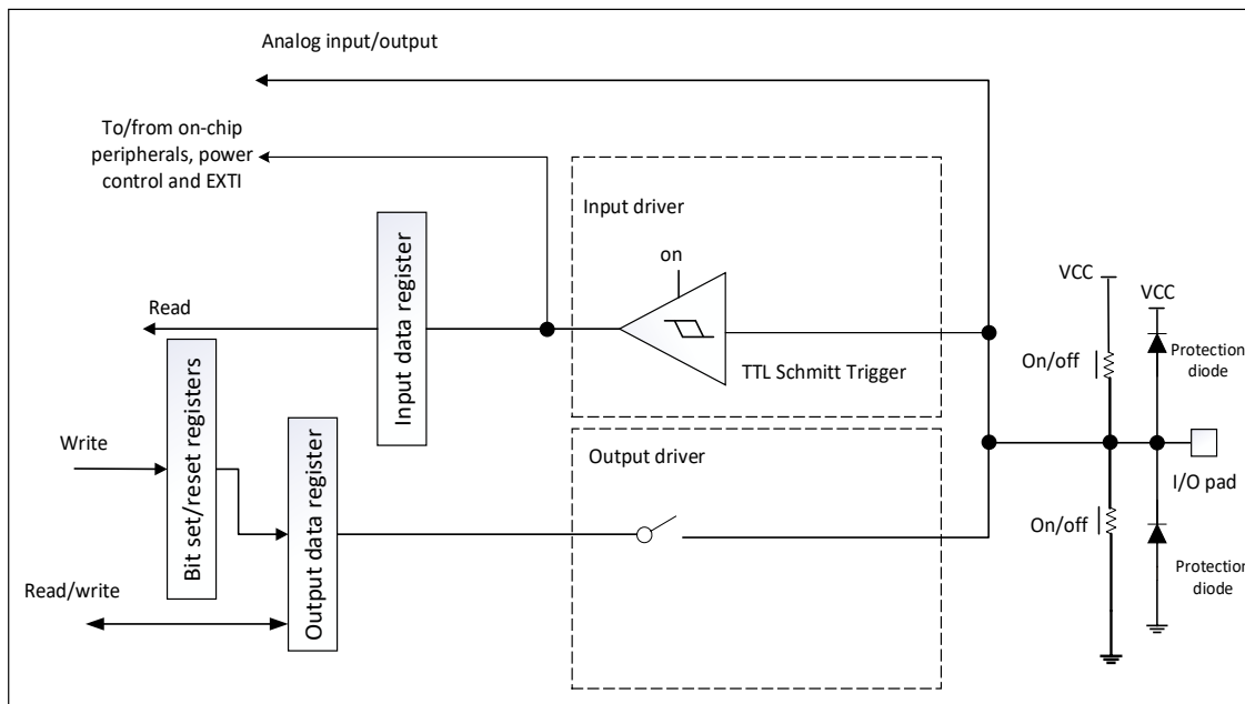
Figure 9-2 Input float/pull-up/pull-down configurations
