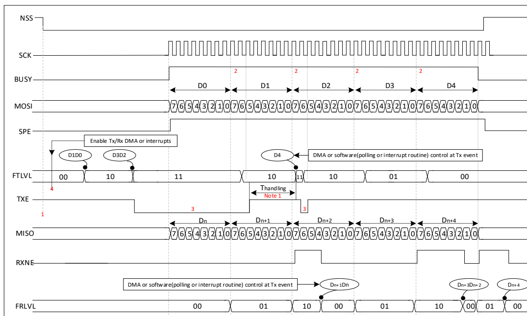
Figure 29-9 Master full-duplex communication timing (data width=8, FRXTH=0)
