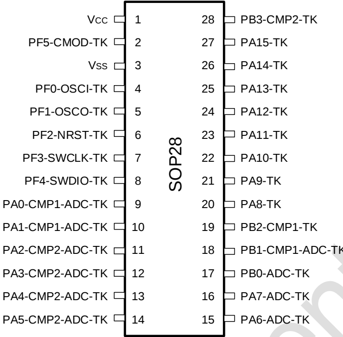
图 3-3 SOP28 Pinout1 PY32T020G1xS7-B (Top view)
