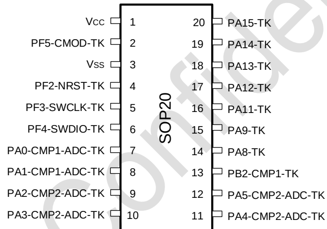
Figure 3-8 SOP20 Pinout1 PY32T020F1xS7-B(Top view)
