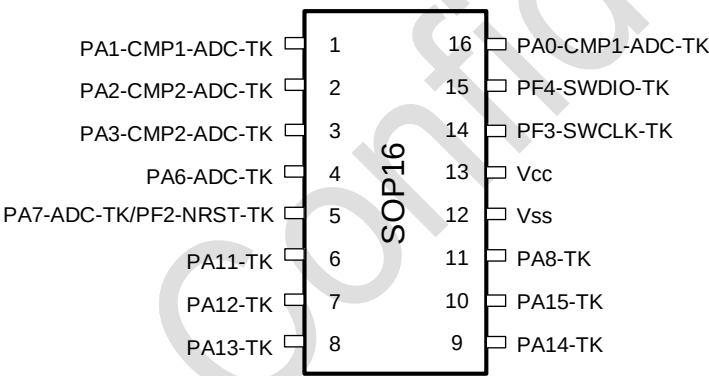
Figure 3-11 SOP16 Pinout2 PY32T020W2xS7-B(Top view)
