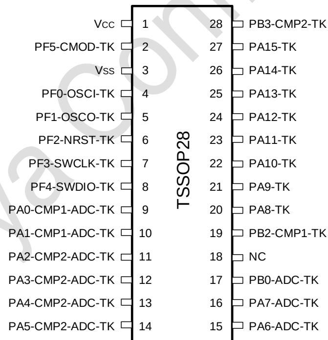
Figure 3-2 TSSOP28 Pinout4 PY32T020G4xP7-B (Top view)
