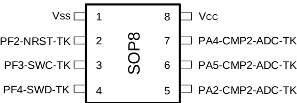
Figure 3-12 SOP8 Pinout1 PY32T020L1xS7-B(Top view)
