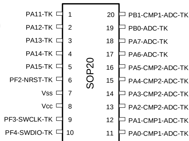
Figure 3-9 SOP20 Pinout2 PY32T020F2xS7-B(Top view)
