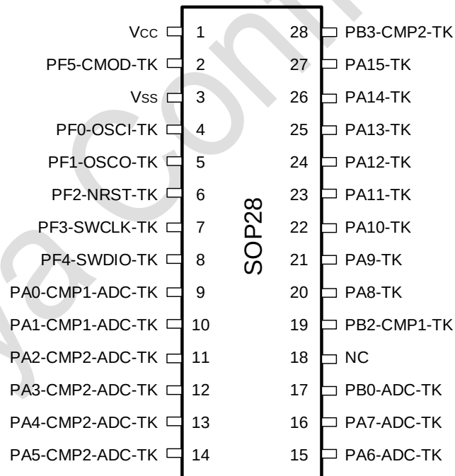
Figure 3-6 SOP28 Pinout4 PY32T020G4xS7-B (Top view)
