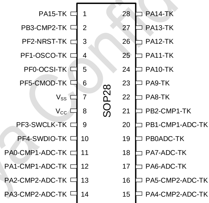
Figure 3-4 SOP28 Pinout2 PY32T020G2xS7-B(Top view)
