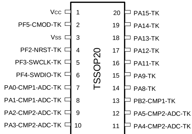
Figure 3-7 TSSOP20 Pinout1 PY32T020F1xP7-B(Top view)
