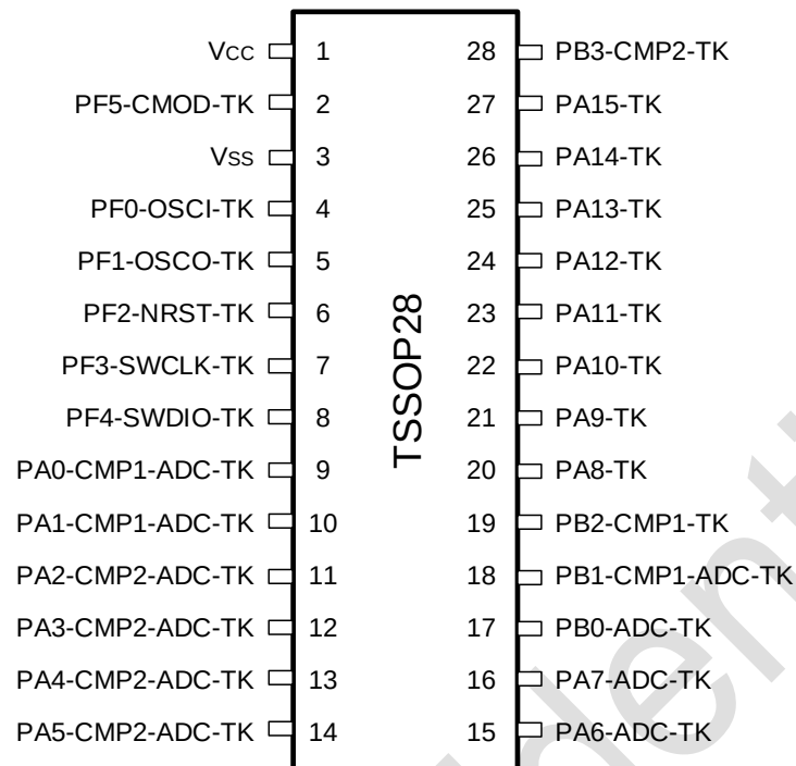
Figure 3-1 TSSOP28 Pinout1 PY32T020G1xP7-B(Top view)
