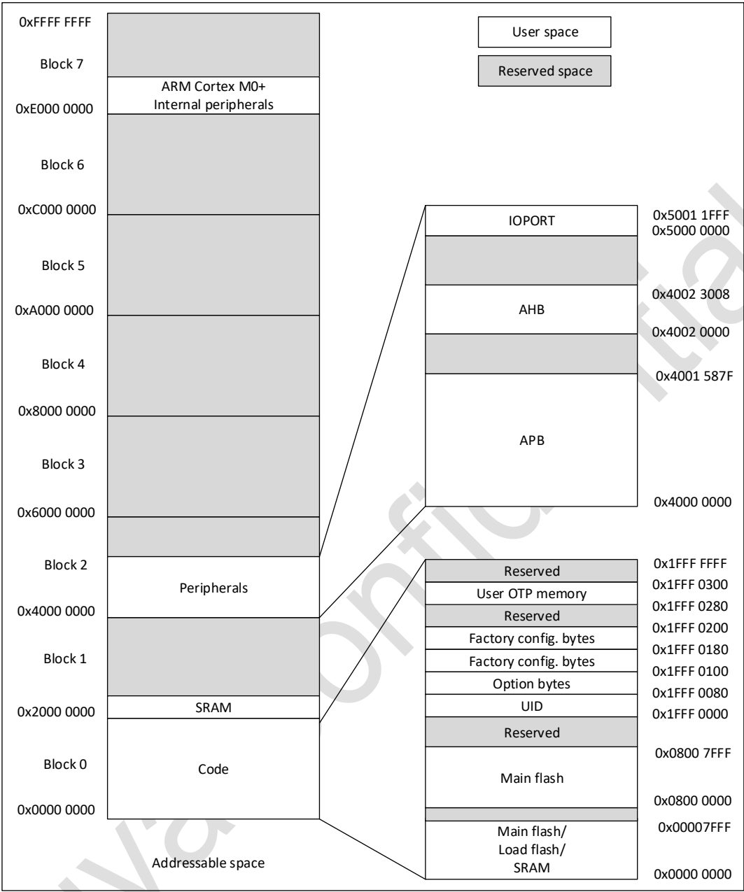
Figure 4-1 Memory map
