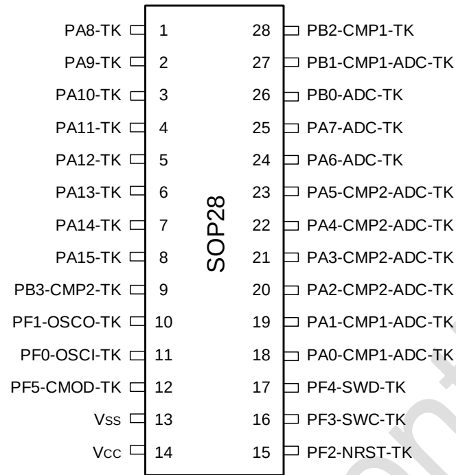
Figure 3-5 SOP28 Pinout3 PY32T020G3xS7-B(Top view)
