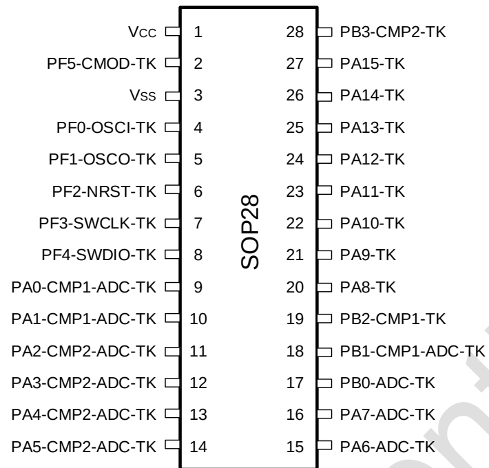
Figure 3-3 SOP28 Pinout1 PY32T020G1xS7-B(Top view)
