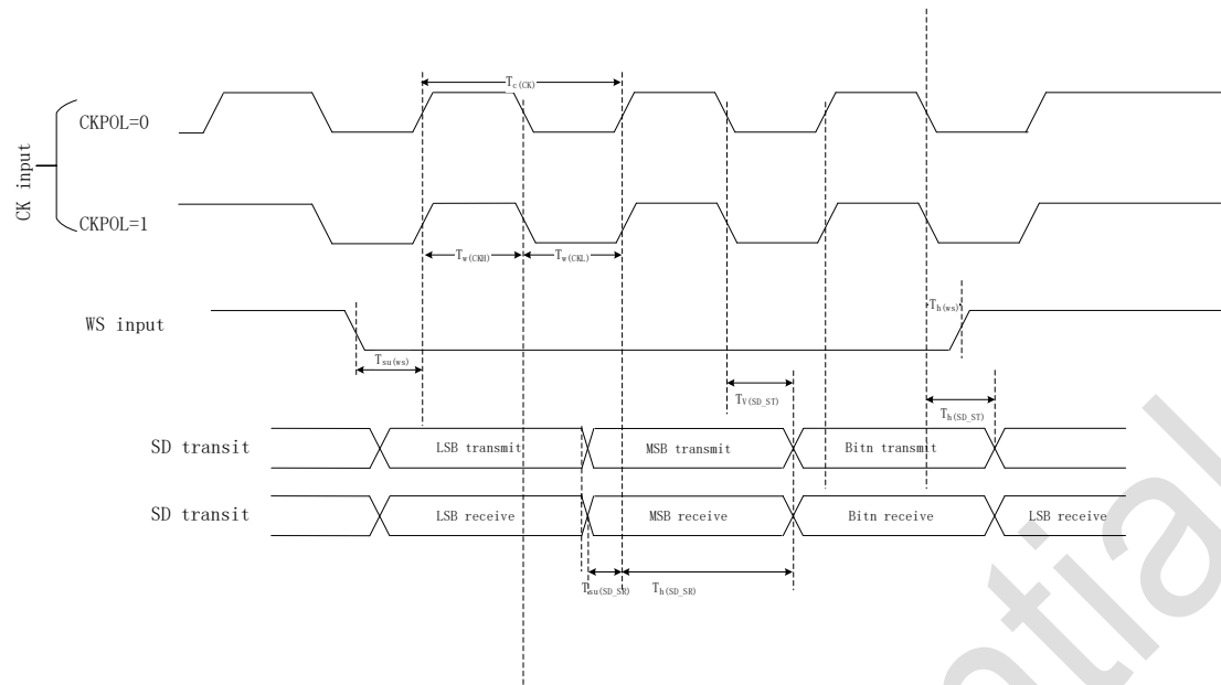
Figure 5-8 I²S timing diagram – Slave mode(Philips protocol)
