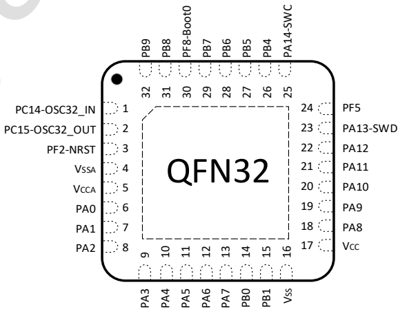
Figure3-5 QFN32(4*4) PY32F071K3xU7-E Pinout3 (Top view)
