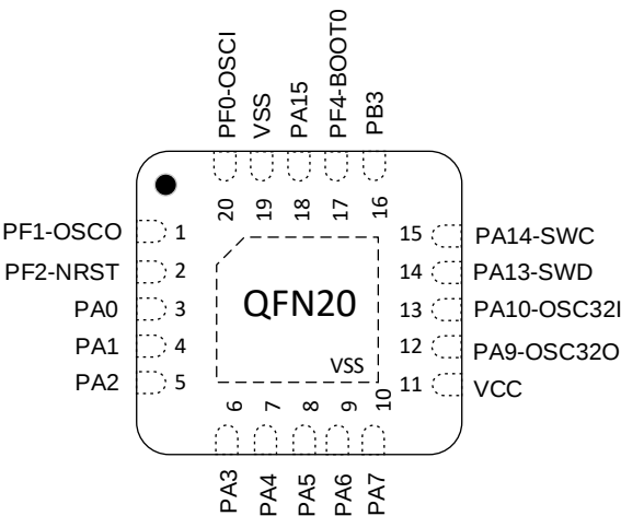
图 3-7 QFN20 Pinout2 PY32F032F2xU7 (Top view)
