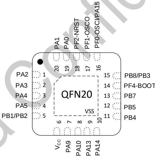
图 3-6 QFN20 Pinout1 PY32F032F1xU7 (Top view)
