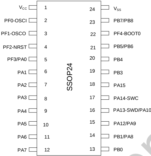
图 3-3 SSOP24 Pinout2 PY32F032E2xM7 (Top view)
