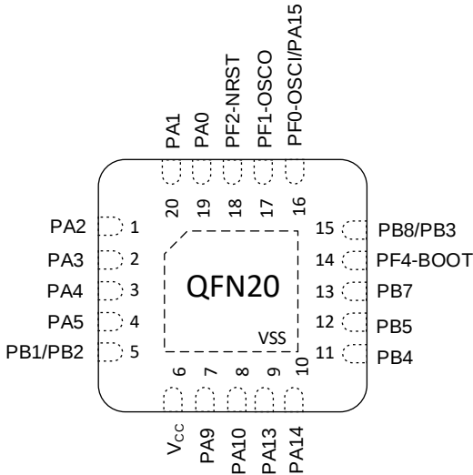
图 3-3 QFN20 Pinout1 PY32F032F1xU7(Top view)
