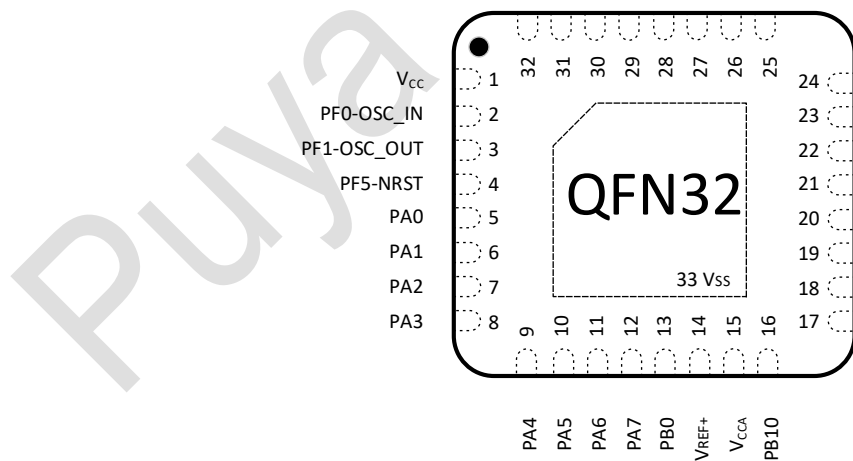
图 3-5 QFN32 Pinout1 PY32E407K1EU7 (Top view)
