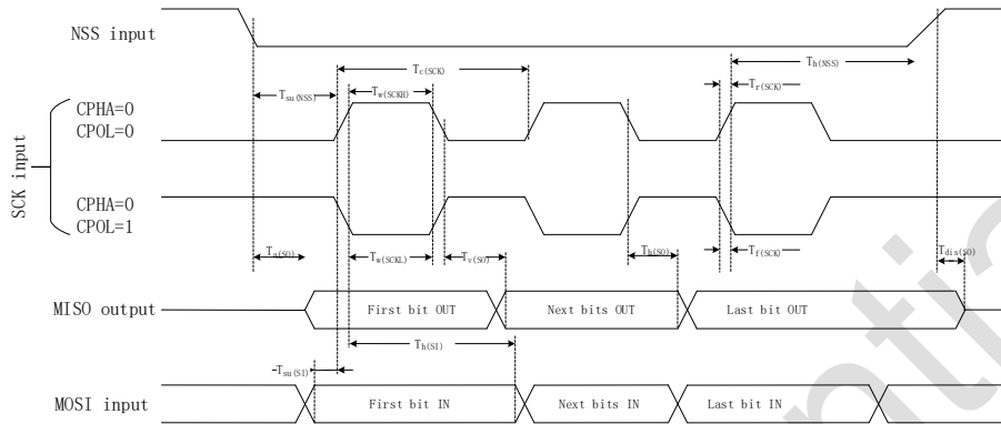
Figure 5-5 SPI timing diagram – slave mode and CPHA=0
