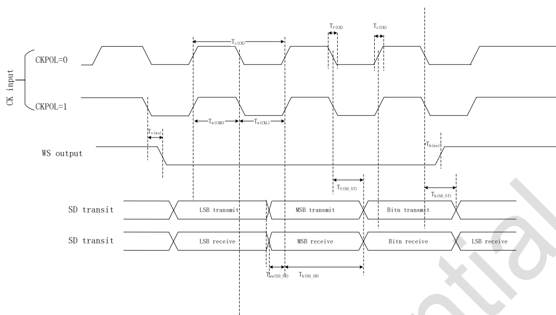
Figure 5-9 I²S master timing diagram (Philips protocol)
