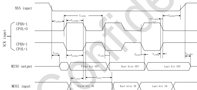
Figure 5-6 SPI timing diagram – slave mode and CPHA = 1 (1)
