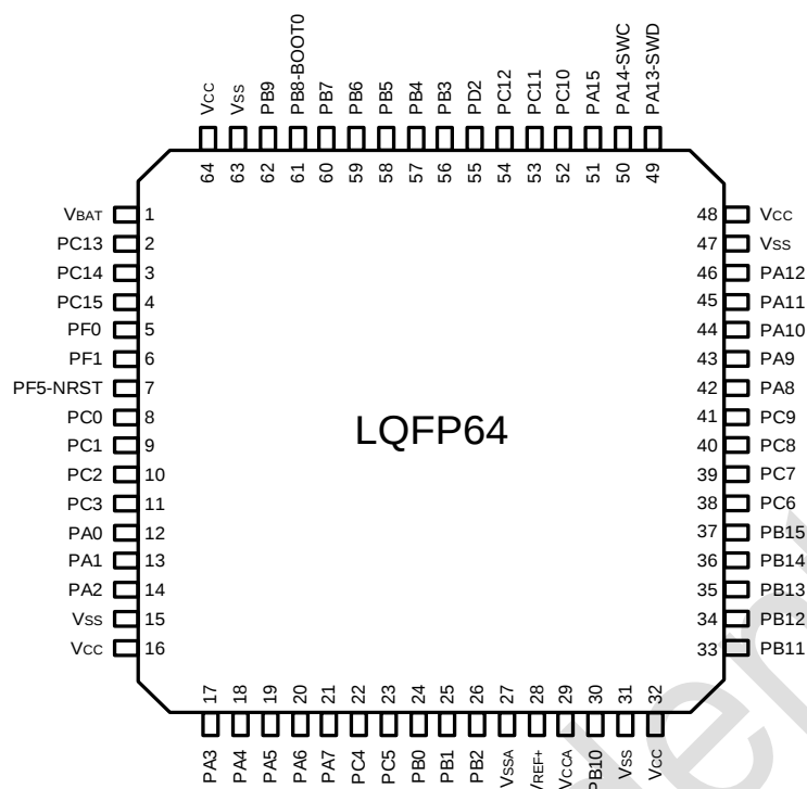
Figure 3-2 LQFP64 Pinout1 PY32E407R1ET7(Top view)
