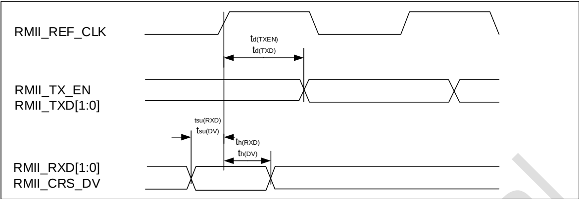
Figure 5-12 RMII timing
