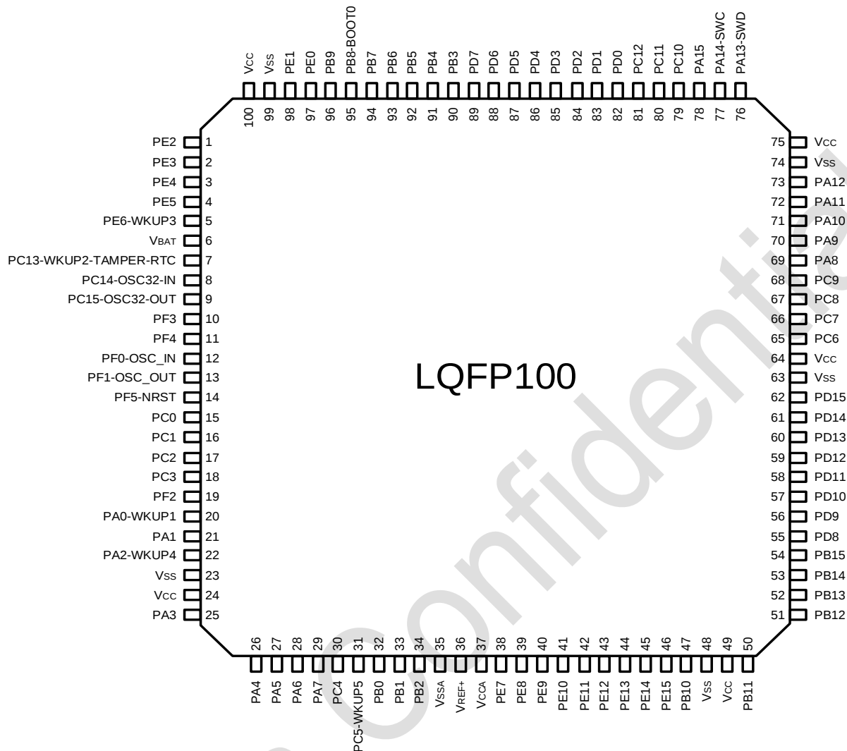
Figure 3-1 LQFP100 Pinout1 PY32E407V1ET7(Top view)
