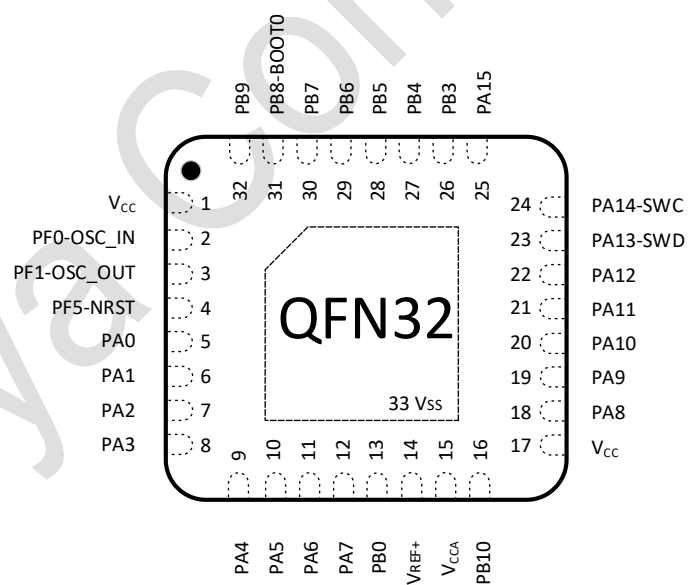
Figure 3-5 QFN32 Pinout1 PY32E407K1EU7 (Top view)
