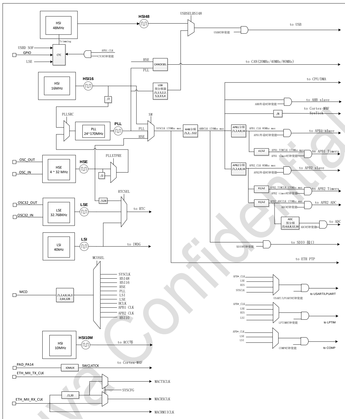
Figure 2-1 System clock structure diagram
