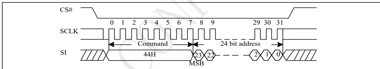
Figure 10-25 Erase Security Registers (ERSCUR) Sequence (Command 44H)
