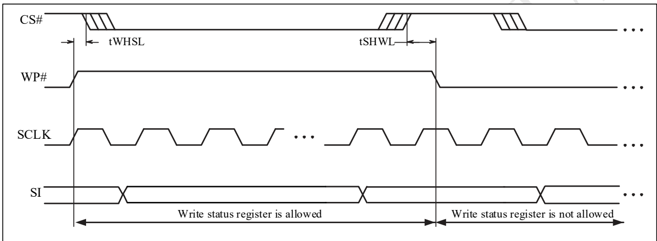
Figure 5-7 WP Timing
