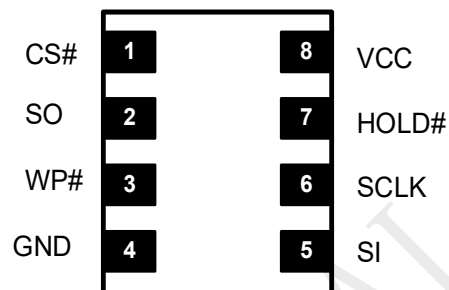
8-Pad USON (3x2/1.5x1.5mm) and WSON(6x5mm)
