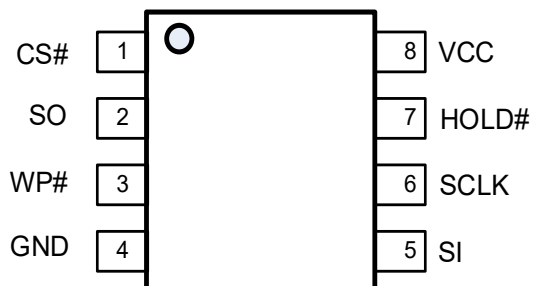
8-Lead SOP (150mil/208mil) and TSSOP
