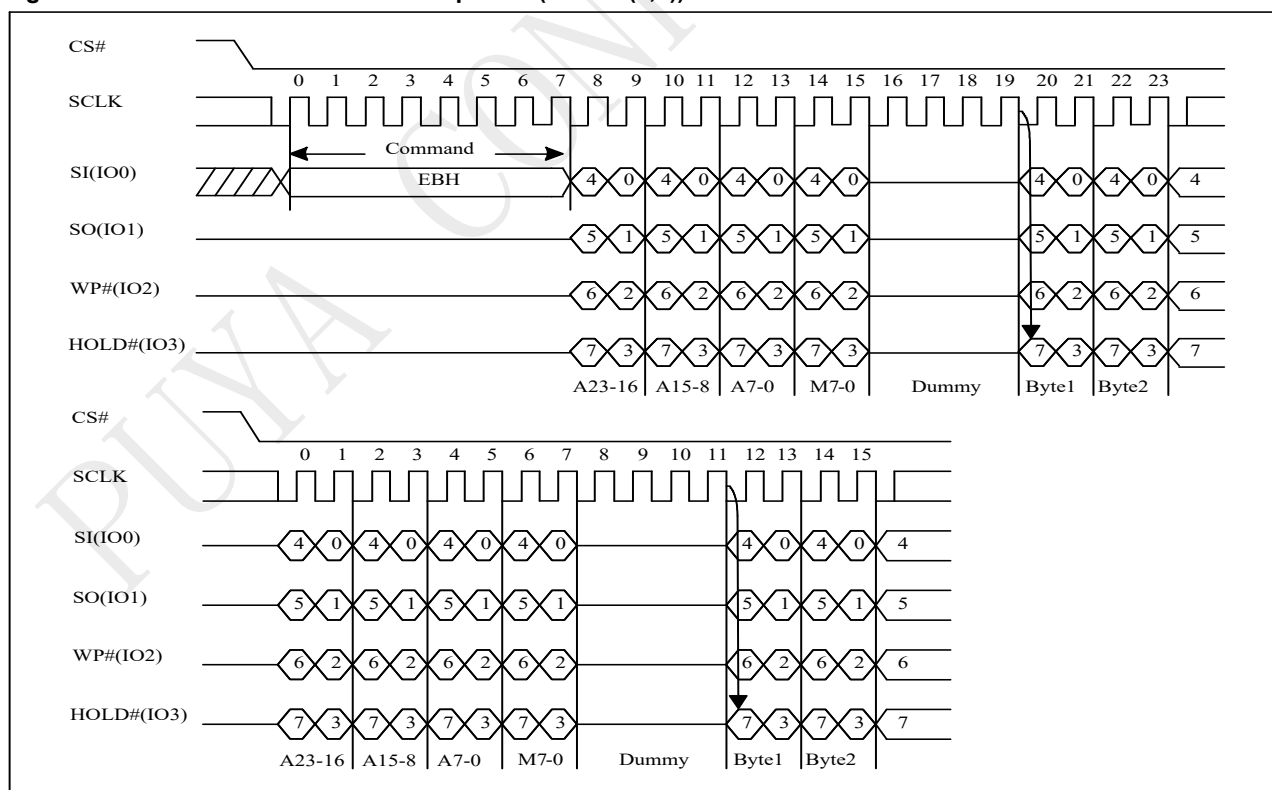
Figure 10-12b 4IO Continuous Read Sequence (M5-4 = (1,0))
