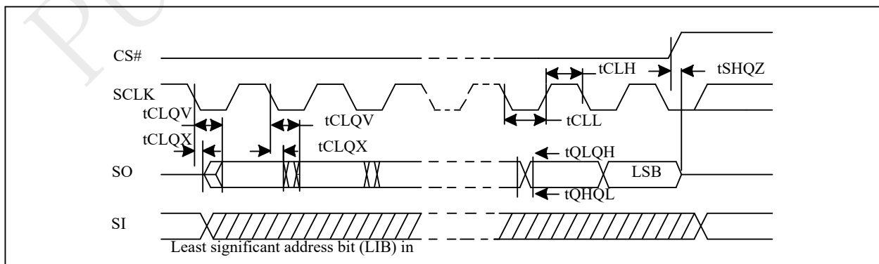
Figure 5-5 Output Timing
