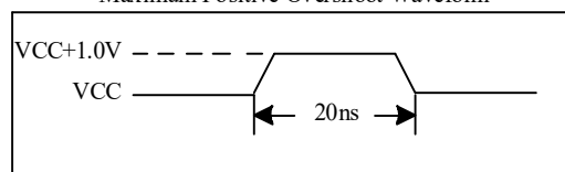
Maximum Positive Overshoot Waveform
