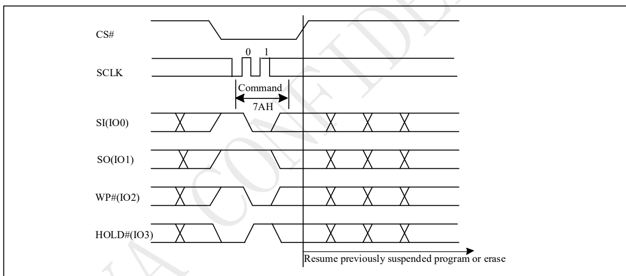
Figure 10-36a Resume to Read Latency (QPI)
