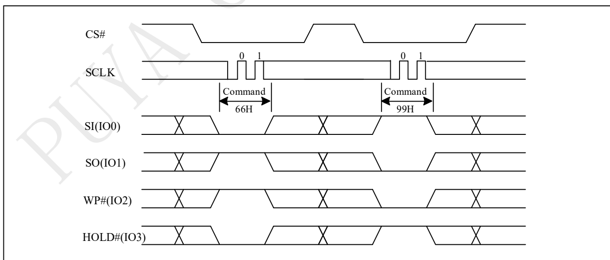
Figure 10-38b Reset Sequence (QPI)
