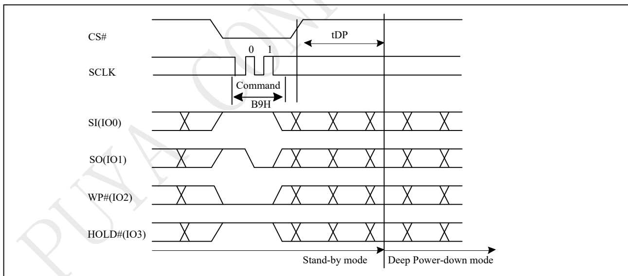
Figure 10-28a Deep Power-down (DP) Sequence (QPI)
