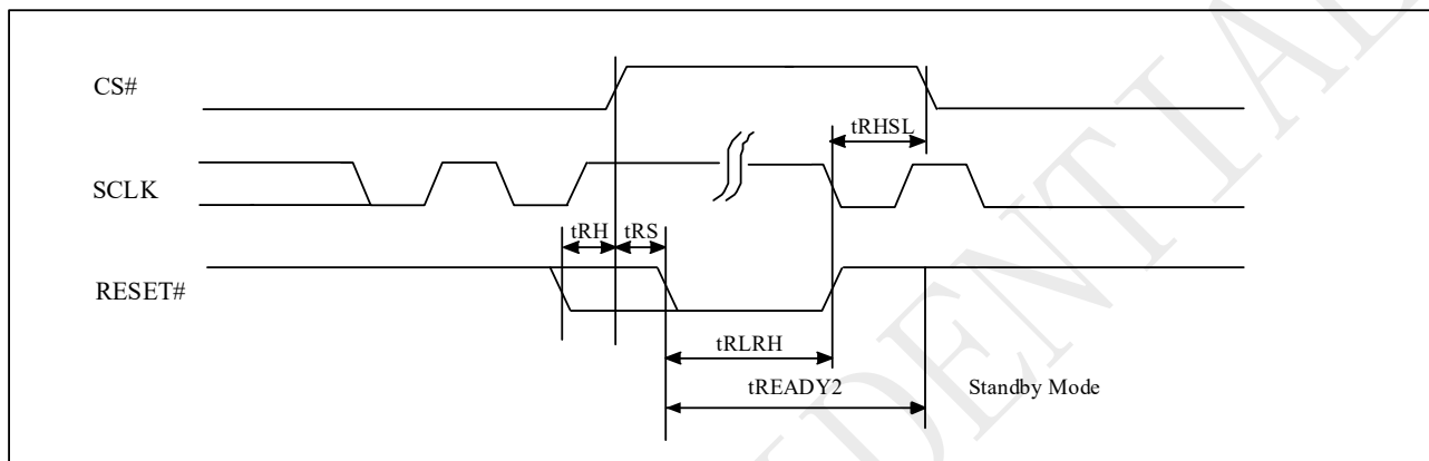
Figure 10-68 RESET Timing
