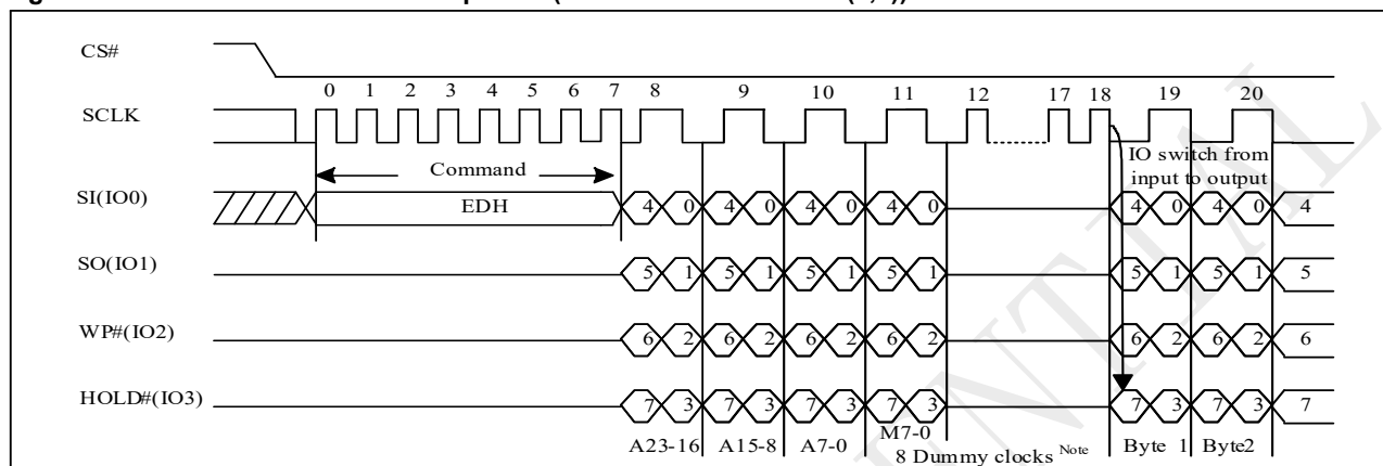
Figure 10-27 DTR 4IO Read Mode Sequence (Command EDH M5-4 ≠ (1,0))
