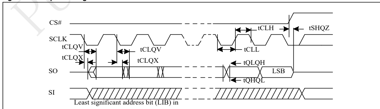
Figure 5-5 Output Timing
