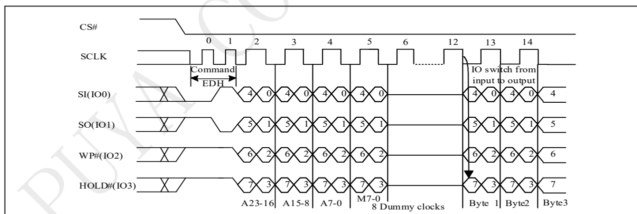
Figure 10-27b DTR 4IO Read Mode Sequence (QPI EDH M5-4 \neq (1,0))
