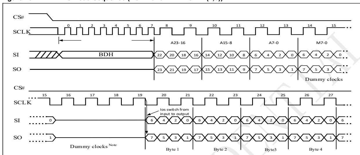
Figure 10-21 DTR 2IO Read Sequence (Command BDH M5-4 ≠ (1,0))
