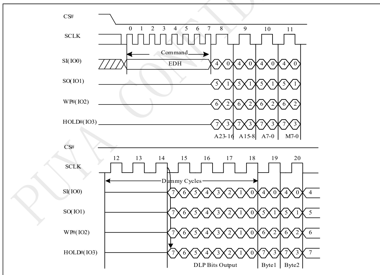
Figure 10-33e DTR 4IO Read with DLP bits output Sequence
