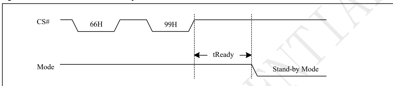
Figure 10-67a Reset Sequence
