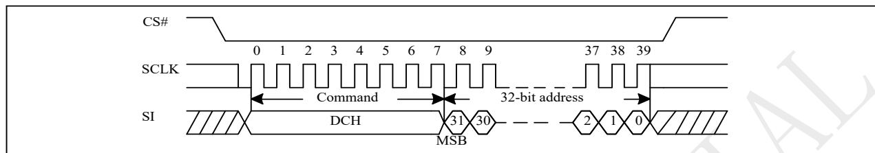
Figure 10-41 Block Erase with 4-Byte Address Sequence (Command DCH)
