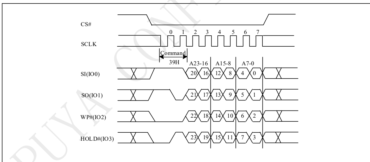
Figure 10-63a Individual Block Unlock (QPI)
