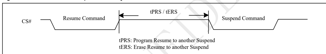
Figure 10-58 Resume to Suspend Latency
