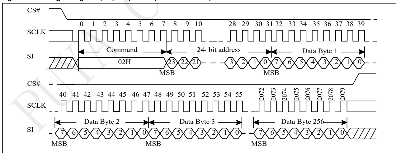
Figure 10-43 Page Program (PP) Sequence (Command 02H)
