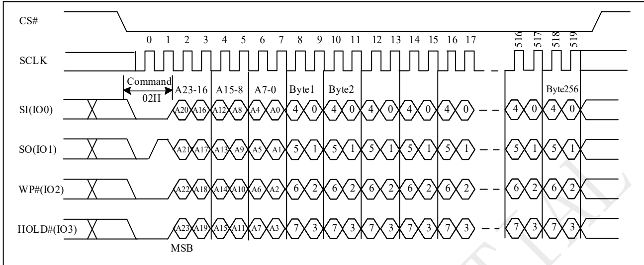
Figure 10-43a Page Program (PP) Sequence (QPI)
