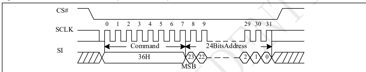
Figure 10-61 Individual Block Lock (Command 36H)
