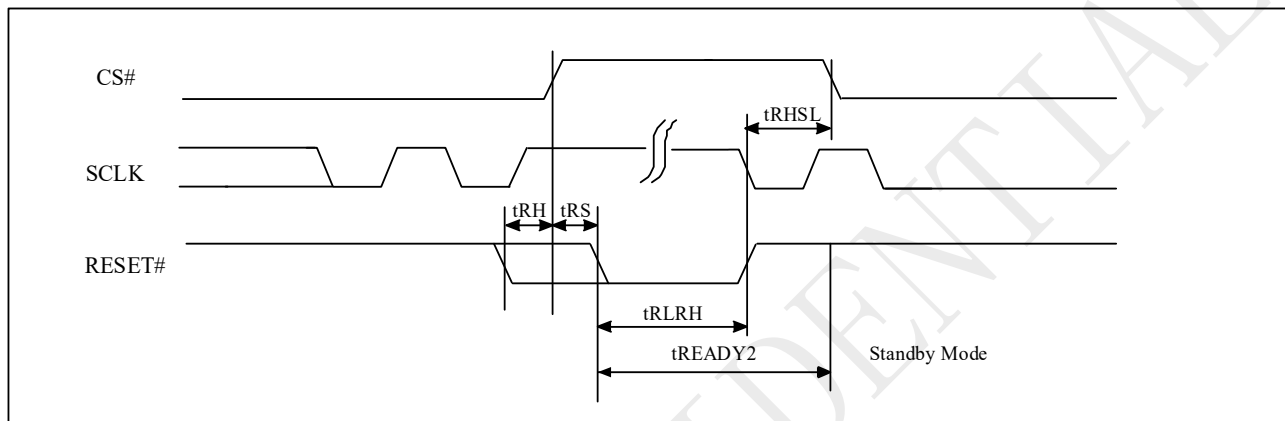
Figure 10-67 RESET Timing
