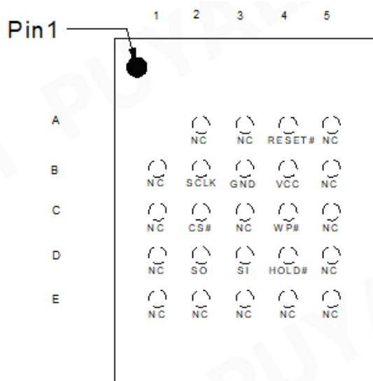
24-Ball TFBGA (5x5 Array)
