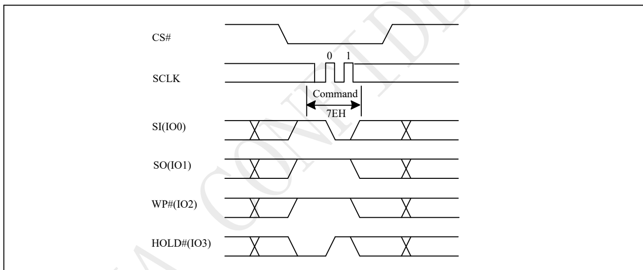
Figure 10-64a Global Block Lock (QPI)
