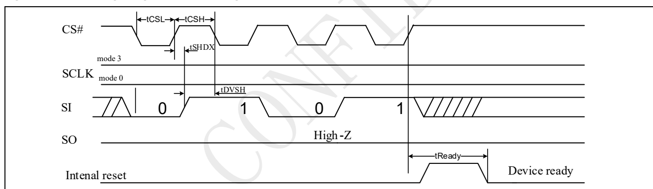
Figure 10-68 Timing Diagram and Timing Parameters
