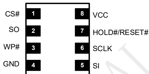
8-Pad WSON (6x5mm/8x6mm)
