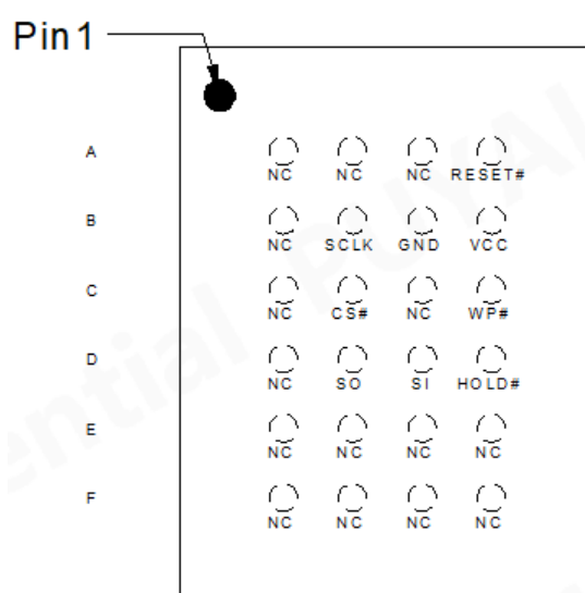
24-Ball TFBGA (4x6 Array)
