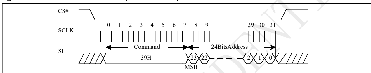
Figure 10-62 Individual Block Unlock (Command 39H)
