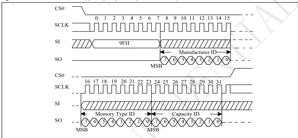
Figure 10-57 Read Identification (RDID) Sequence (Command 9FH)
