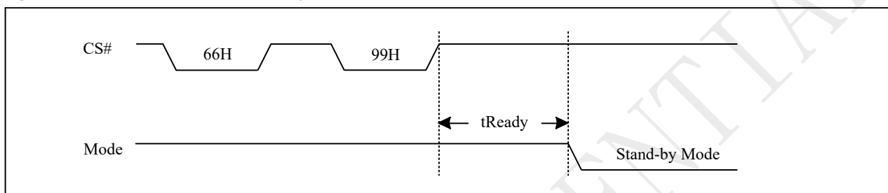
Figure 10-66a Reset Sequence
