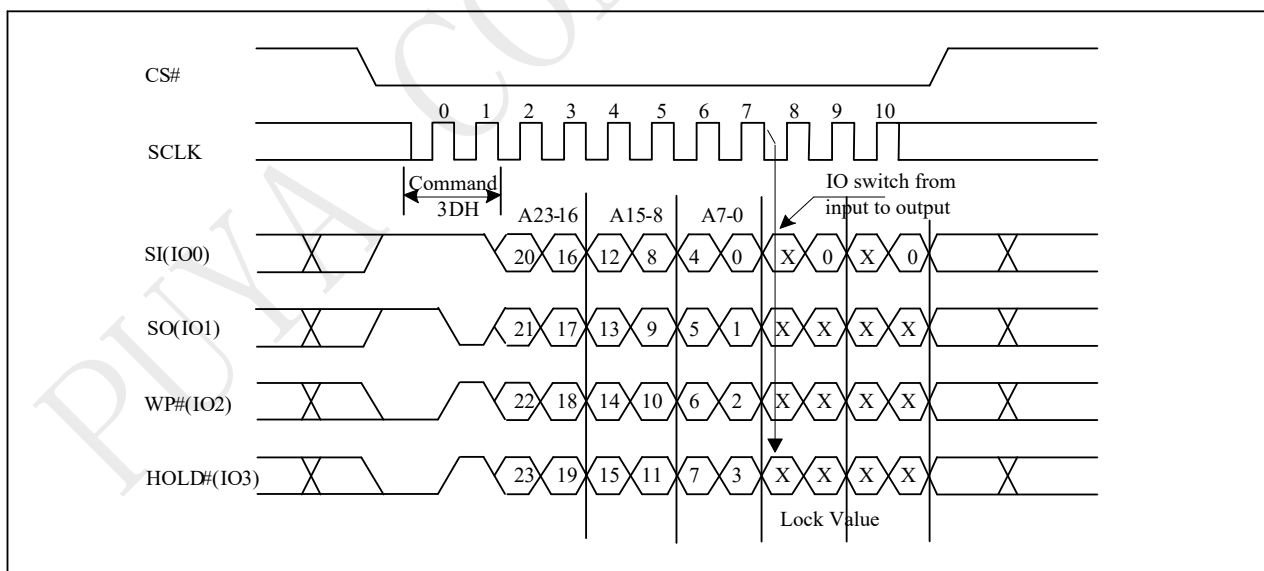
Figure 10-63a Read Block Lock Status (QPI)
