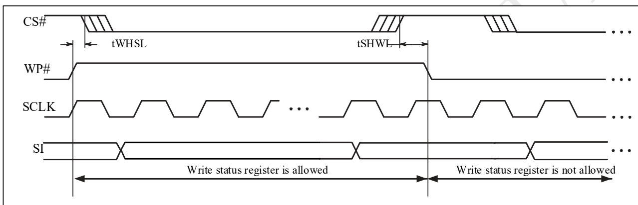
Figure 5-7 WP Timing
