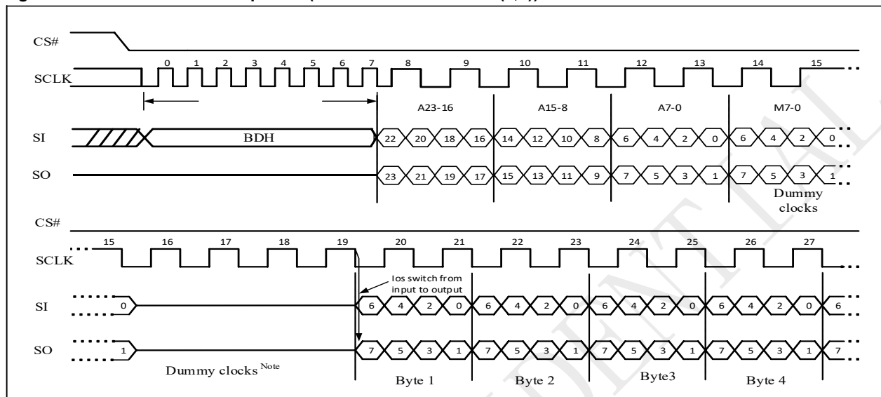
Figure 10-21 DTR 2IO Read Sequence (Command BDH M5-4 ≠ (1,0))
