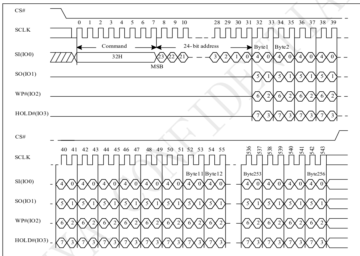
Figure 10-45 Quad Page Program (QPP) Sequence (Command 32H)
