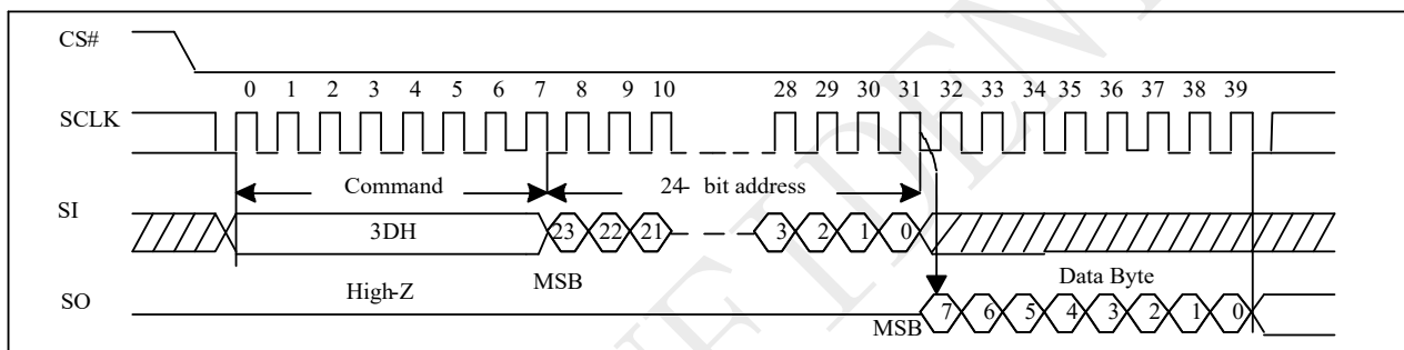
Figure 10-63 Read Block Lock Status (Command 3DH)
