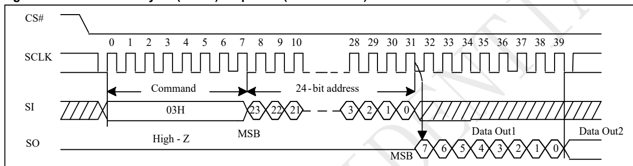
Figure 10-13 Read Data Bytes (READ) Sequence (Command 03)
