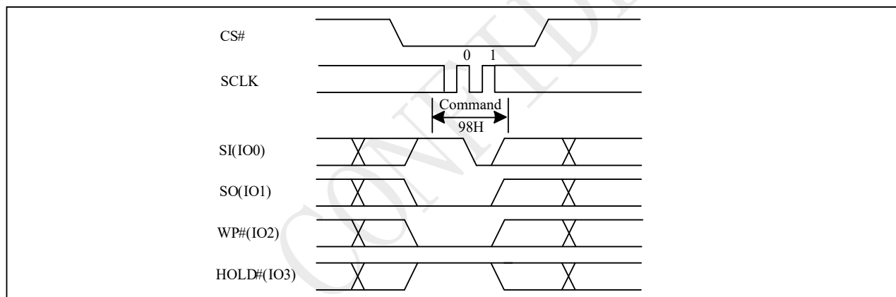
Figure 10-65a Global Block Unlock (QPI)
