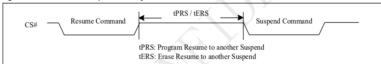
Figure 10-58 Resume to Suspend Latency
