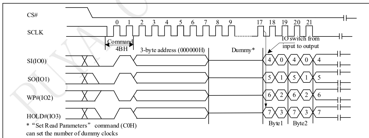
Figure 10-69a Read Unique ID (RUID) Sequence (QPI 4BH)
