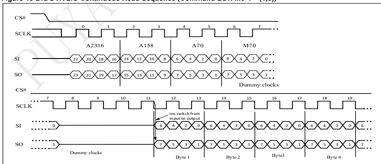
Figure 10-21a DTR 2IO Continuous Read Sequence (Command BDH M5-4 = (1,0))
