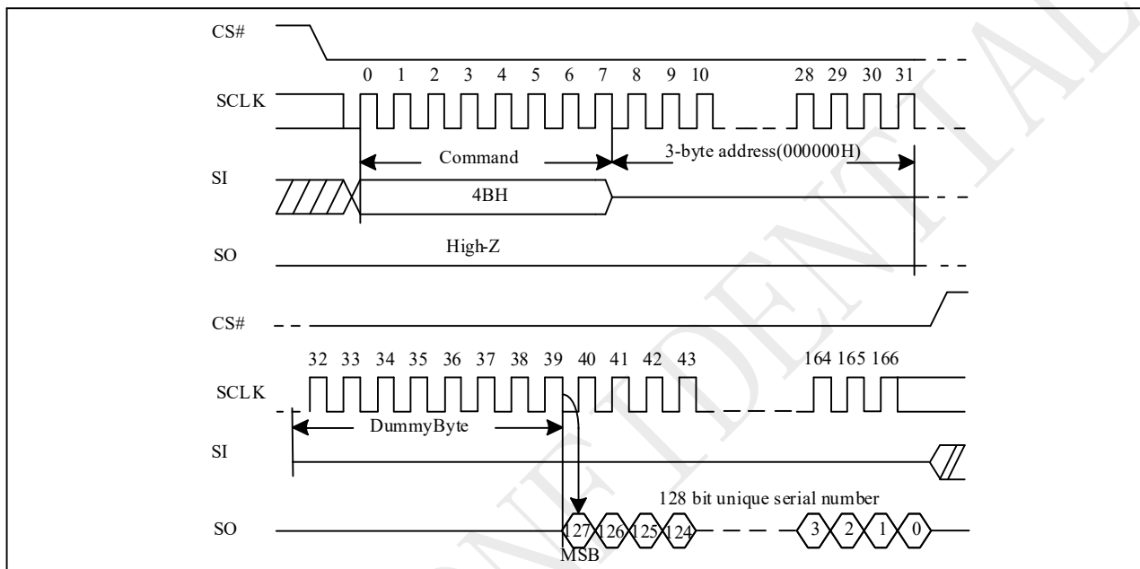
Figure 10-69 Read Unique ID (RUID) Sequence (Command 4BH)
