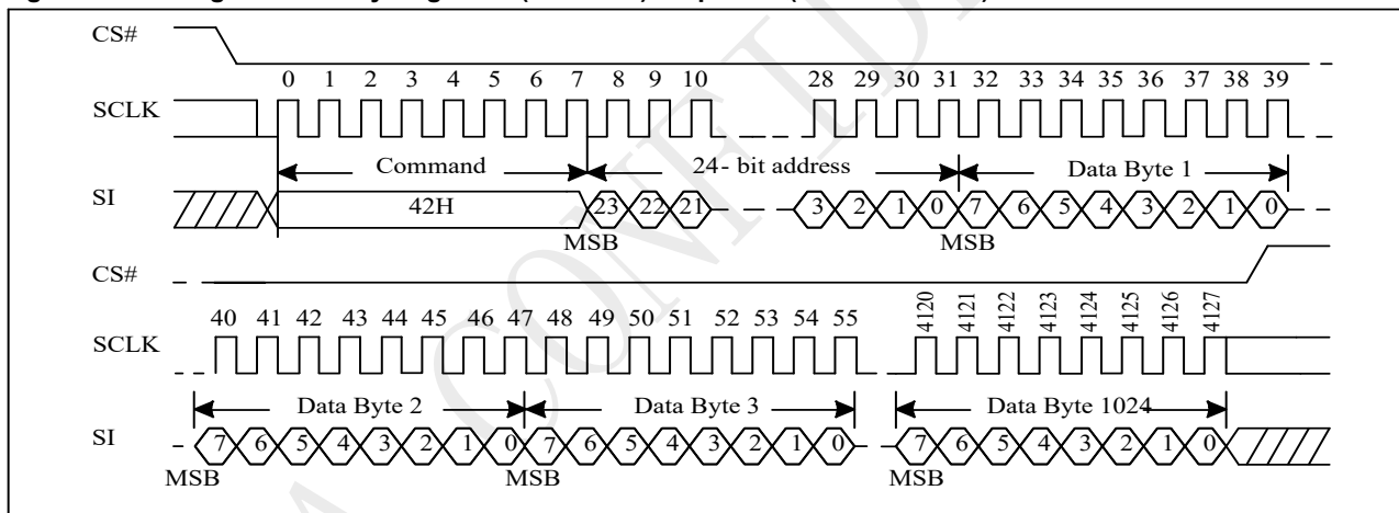
Figure 10-50 Program Security Registers (PRSCUR) Sequence (Command 42H)
