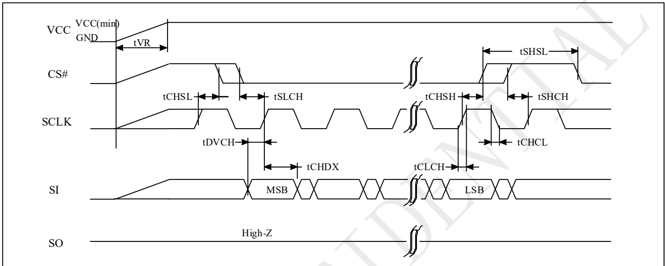
Figure 5-9 Power-up Timing
