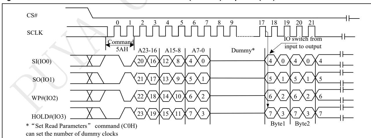
Figure 10-70a Read Serial Flash Discoverable Parameter (RDSFDP) Sequence (QPI)
