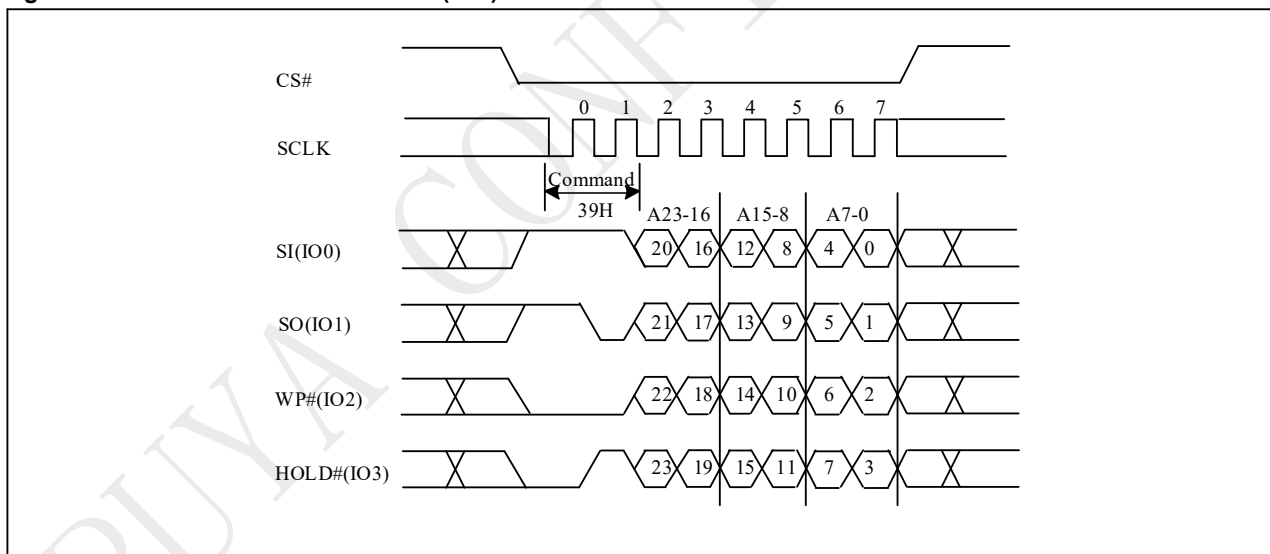
Figure 10-62a Individual Block Unlock (QPI)
