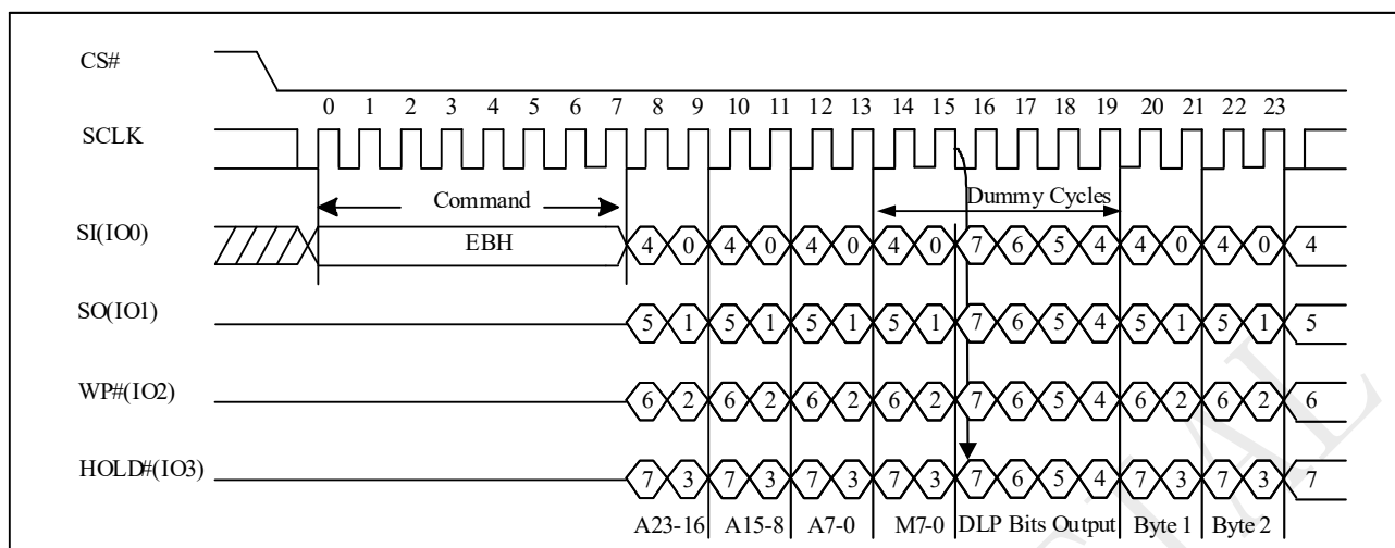
Figure 10-33b 4IO Read with DLP bits output Sequence
