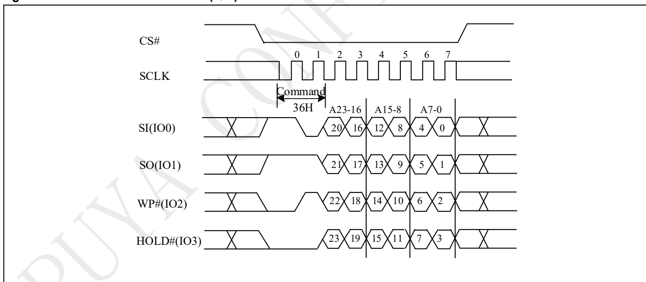
Figure 10-61a Individual Block Lock(QPI)
