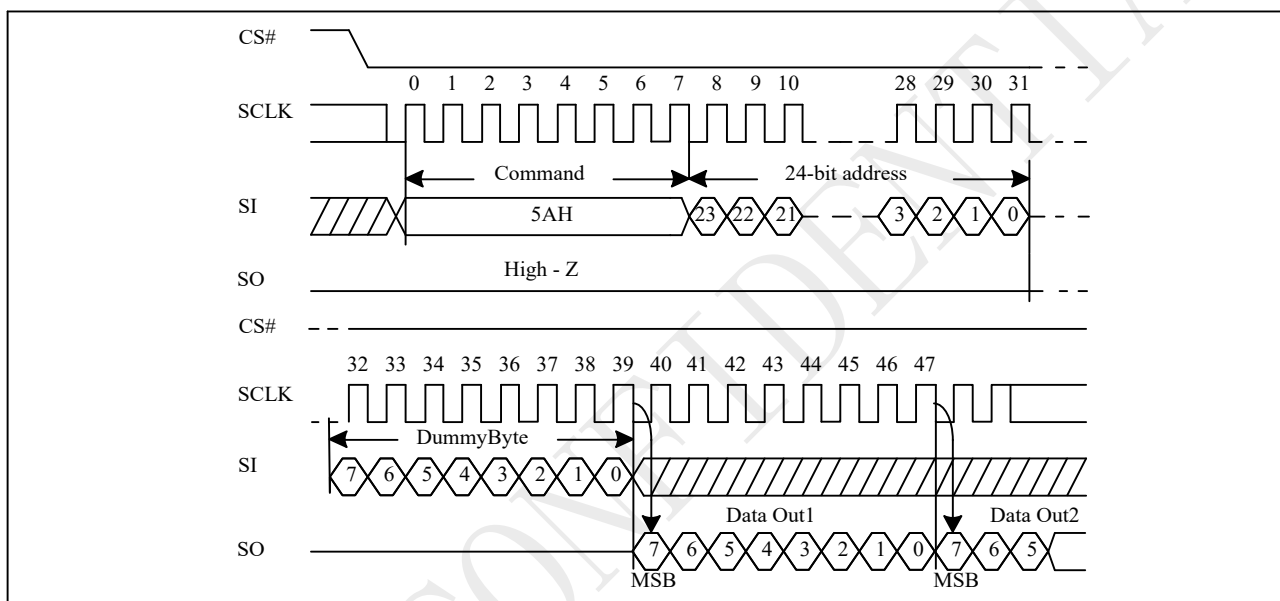
Figure 10-70 Read Serial Flash Discoverable Parameter (RDSFDP) Sequence
