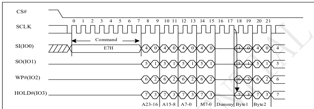
Figure 10-16 4IO Word Read Sequence ( M5-4 ≠ (1,0) )
