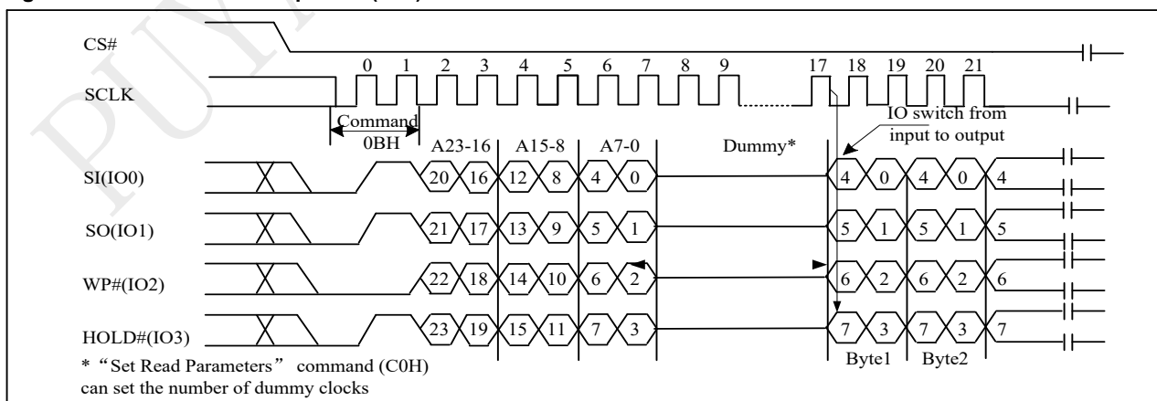
Figure 10-10a Fast Read Sequence (QPI)
