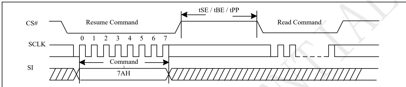
Figure 10-44 Resume to Read Latency
