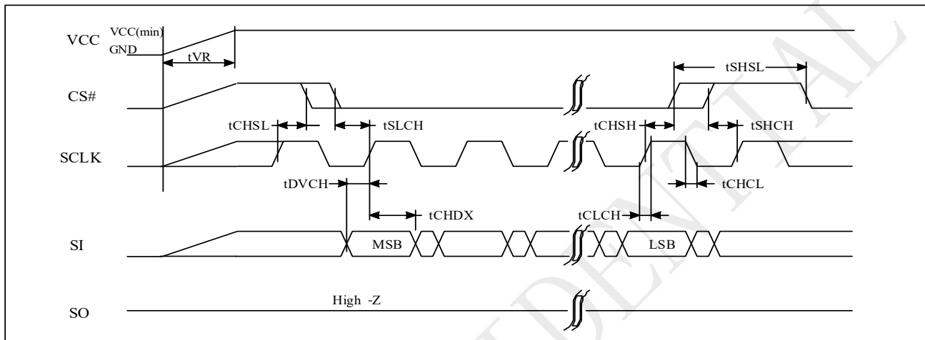
Figure 5-8 AC Timing at Device Power-Up
