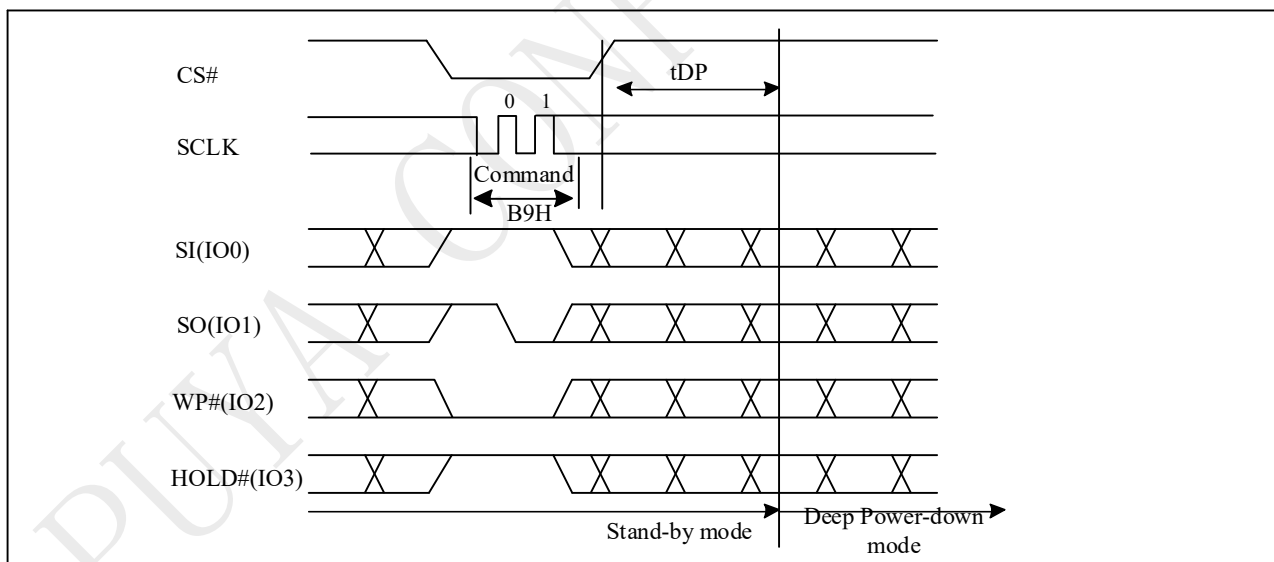
Figure 10-36a Deep Power-down (DP) Sequence (QPI)
