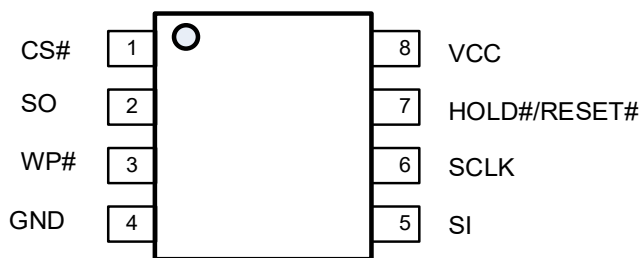
8-Lead SOP (150mil) and TSSOP
