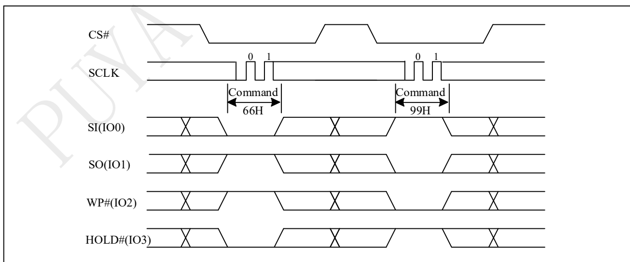
Figure 10-51b Reset Sequence(QPI)
