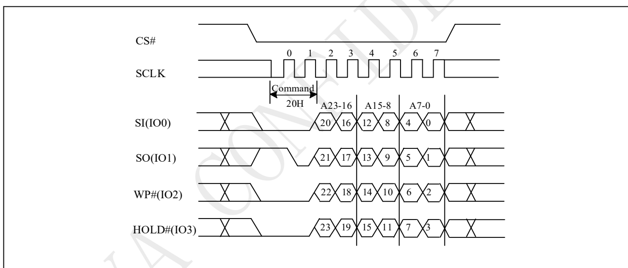
Figure 10-22a Sector Erase (SE) Sequence (QPI)
