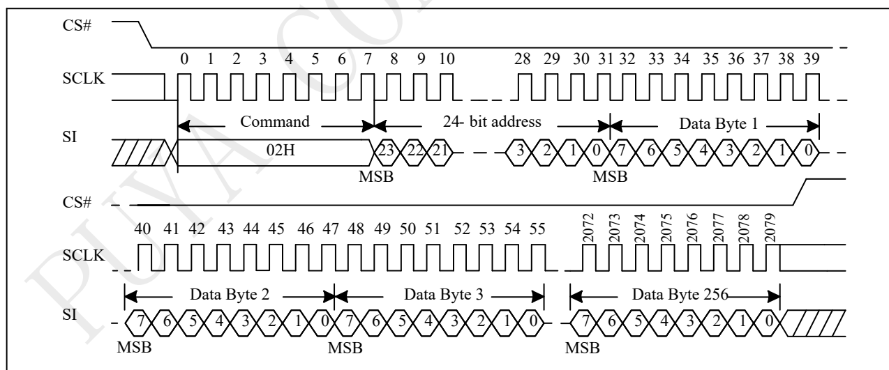
Figure 10-26 Page Program (PP) Sequence (Command 02)
