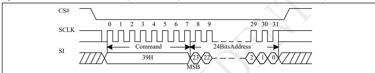
Figure 10-47 Individual Block Unlock (Command 39H)
