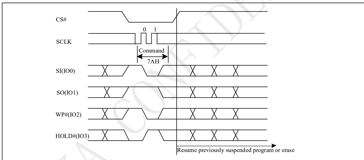
Figure 10-44a Resume to Read Latency(QPI)
