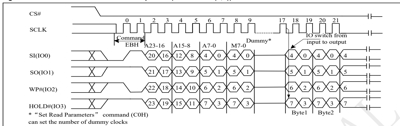
Figure 10-14a 4IO Read in QPI mode Sequence (QPI M5-4 ≠ (1,0))
