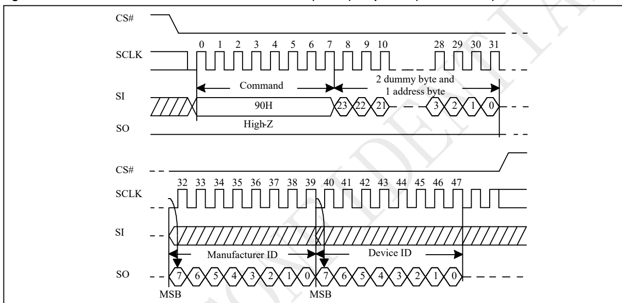
Figure 10-38 Read Electronic Manufacturer & Device ID (REMS) Sequence (Command 90)
