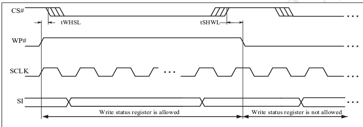
Figure 5-7 WP Timing
