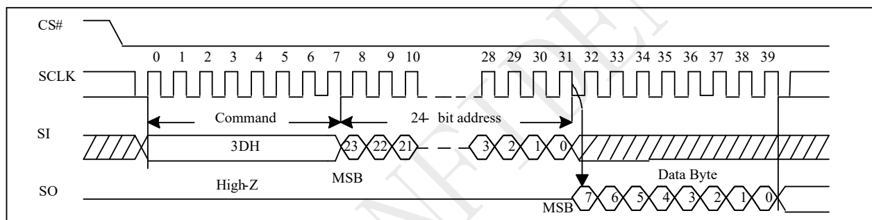
Figure 10-48 Read Block Lock Status (Command 3DH)
