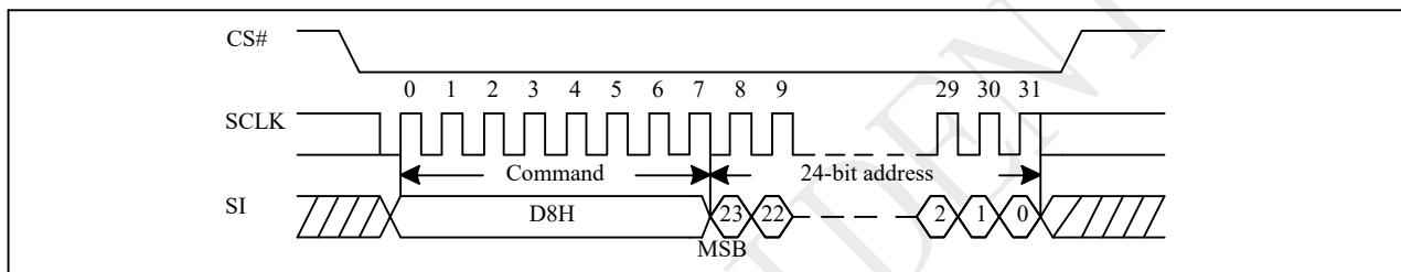
Figure 10-24 Block Erase (BE) Sequence (Command D8)
