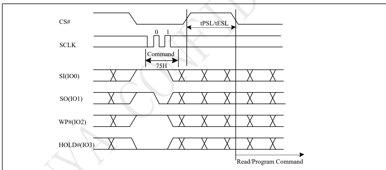
Figure 10-43a Suspend to Read/Program Latency(QPI)
