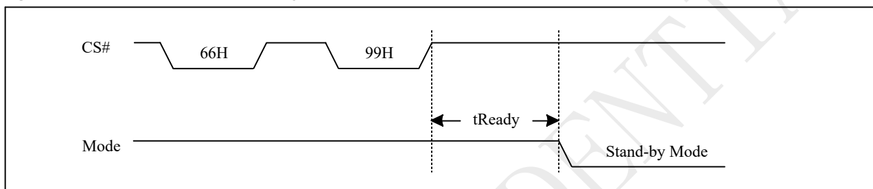
Figure 10-51a Reset Sequence
