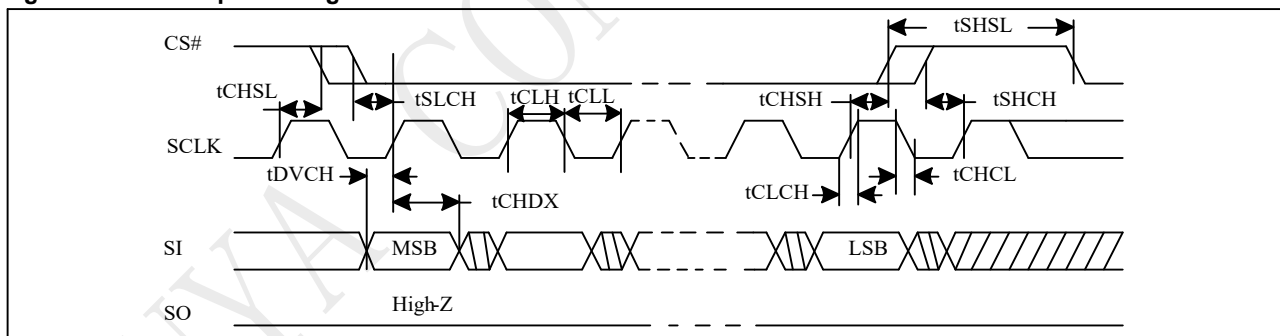
Figure 5-5 Output Timing
