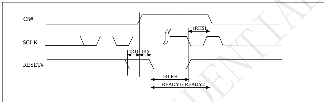
Figure 10-57 RESET Timing
