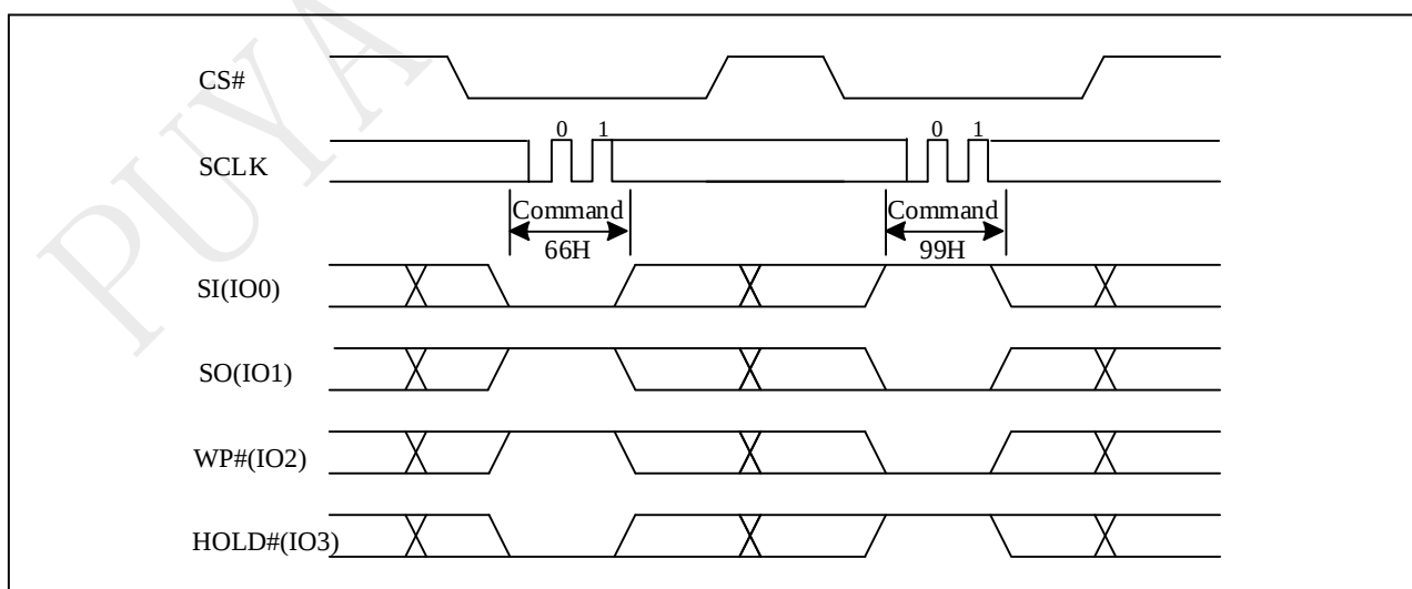
Figure 10-56b Reset Sequence(QPI)
