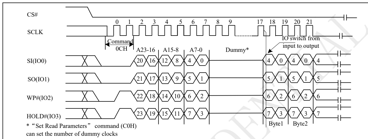
Figure 10-21 Burst Read with Wrap Sequence (QPI)
