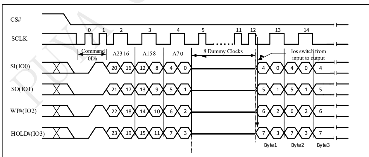
Figure 10-11a DTR Fast Read Sequence (QPI)
