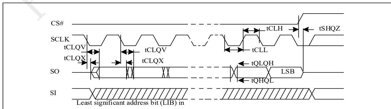
Figure 5-5 Output Timing
