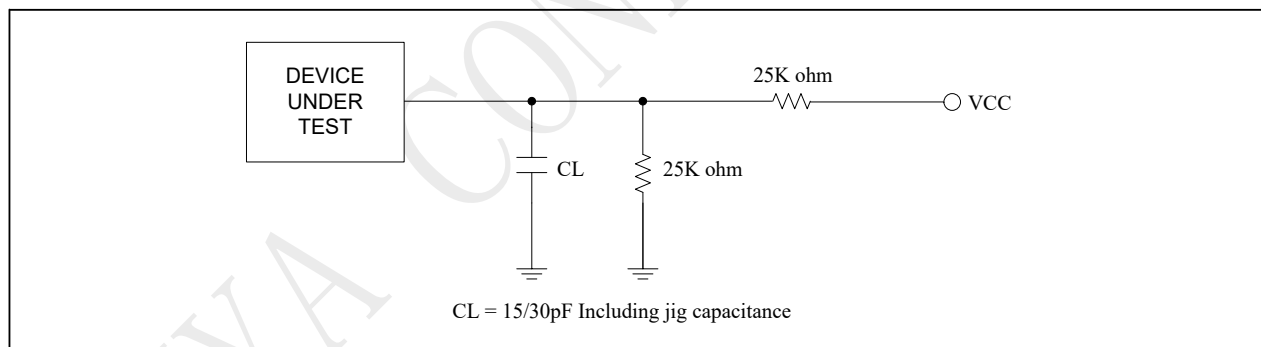
Figure 5-2 Output Loading
