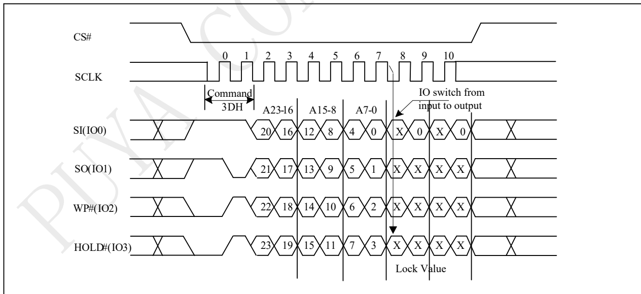
Figure 10-52a Read Block Lock Status (QPI)
