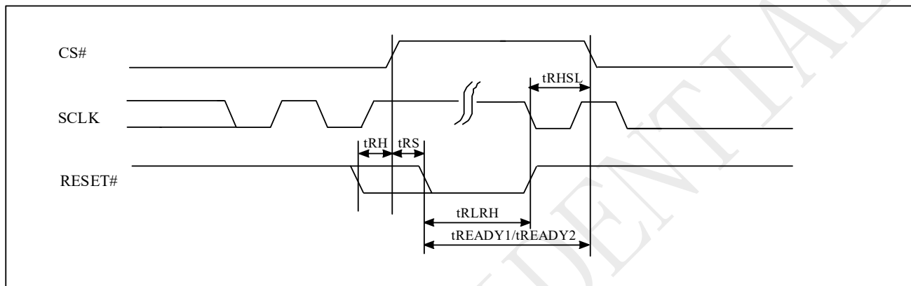
Figure 10-56 RESET Timing
