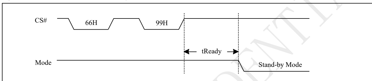
Figure 10-55a Reset Sequence
