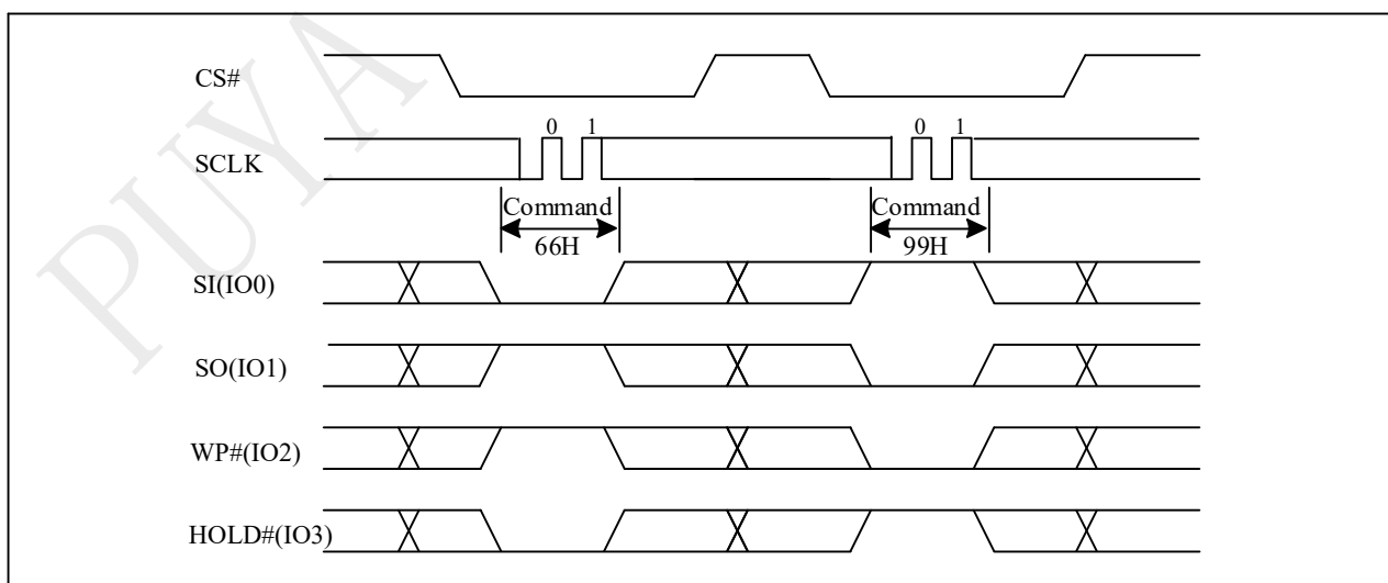
Figure 10-55b Reset Sequence(QPI)
