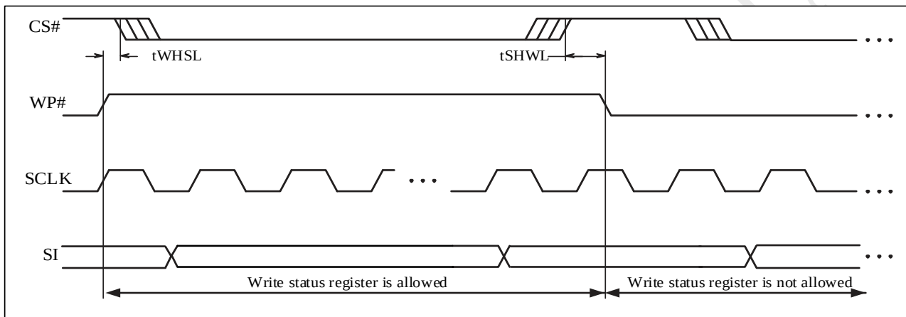
Figure 5-7 WP Timing
