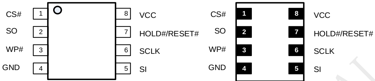
8-Lead SOP (150mil/208mil) and TSSOP
