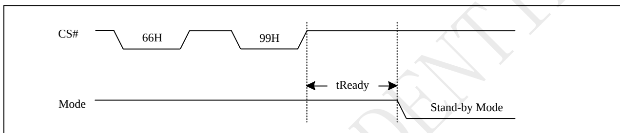
Figure 10-55a Reset Sequence
