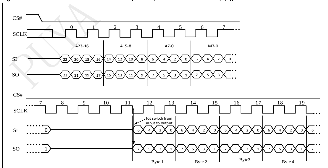
Figure 10-14a DTR 2IO Continuous Read Sequence (Command BD M5-4 = (1,0))
