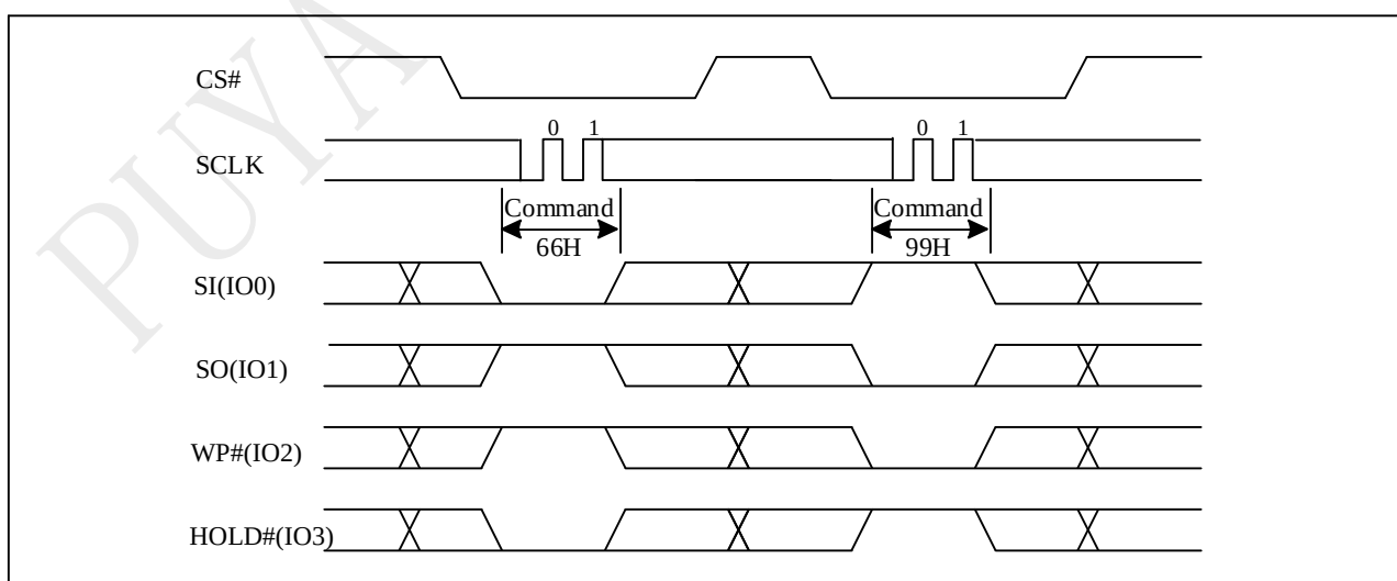
Figure 10-55b Reset Sequence(QPI)
