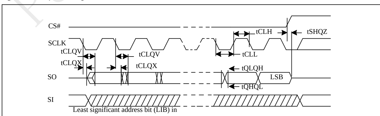
Figure 5-5 Output Timing
