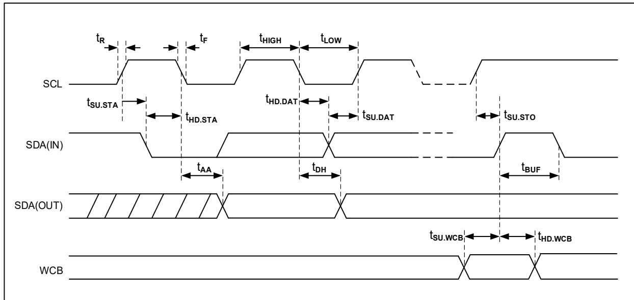
Figure 3-1 Bus Timing
