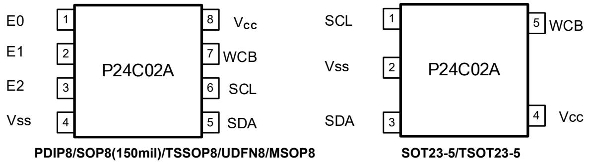
Figure 1-1 Pin Configuration
